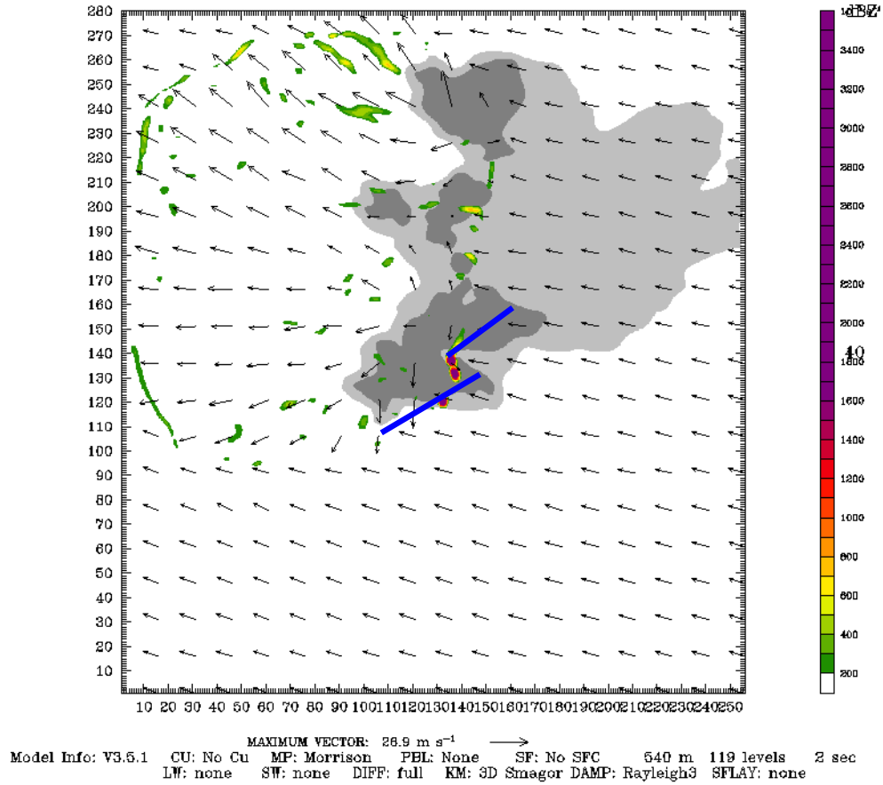
Figure 3.8: An example of a unfavorable gust front (blue lines) orientation taken from the 1500 \text{ J kg}^{-1} CAPE, 125 shear, x, y = -16, -16 case at 1 hour into the simulation. 1 km simulated reflectivity (dBZ) shaded at 10 dBZ (light gray) and 40 dBZ (dark gray). Surface vertical vorticity ( 10^{-5} \text{ s}^{-1} ; color fill starting at 200 \cdot 10^{-5} \text{ s}^{-1} ) and storm-relative winds (vectors).
