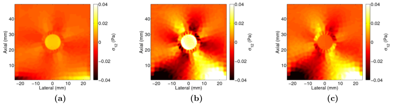
Figure 3.17: Comparison of the estimated shear stress field \sigma_{12} of phantom 1 using training versions (1) and (4). (a) Training version (1) corresponds to the shear response in Figure 3.5c. (b) Training version (4) where displacement convergence is required for nodes not used for training; the results correspond to the shear response in Fig. 3.16d. (c) Shear stress estimated for an ideal linear-elastic plane-stress model. This is the same shear stress field displayed in Figure 3.6c
