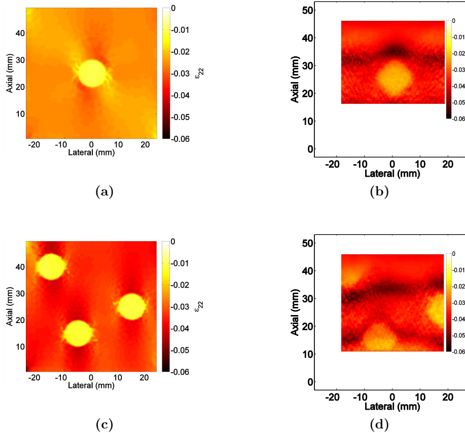
Figure 3.11: Comparison of the axial strain computed using trained ANN material models and a speckle-tracking algorithm. Axial strains computed using the ANNs come from FE_{ANN} . A least-squares estimator was used to compute strain after displacement estimation from speckle-tracking. (a) Phantom 1, axial strain computed from FE_{ANN} (b) Phantom 1, axial strain computed from speckle-tracking (c) Phantom 3, axial strain computed from FE_{ANN} (d) Phantom 3, axial strain computed from speckle-tracking
