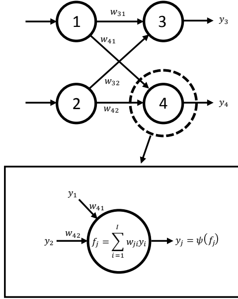
Figure 2.2: Example of a simple two-layer, feed-forward ANN. Output from nodes are weighted and summed to form the input to a node in the succeeding layer. The input signal is passed to an activation function, the output of which becomes the output of the node.
