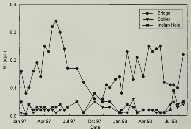
Figure 19 Temporal changes in Mn concentrations in spring and surface water samples showing seasonally elevated concentrations of Mn at the bridge site during spring.
