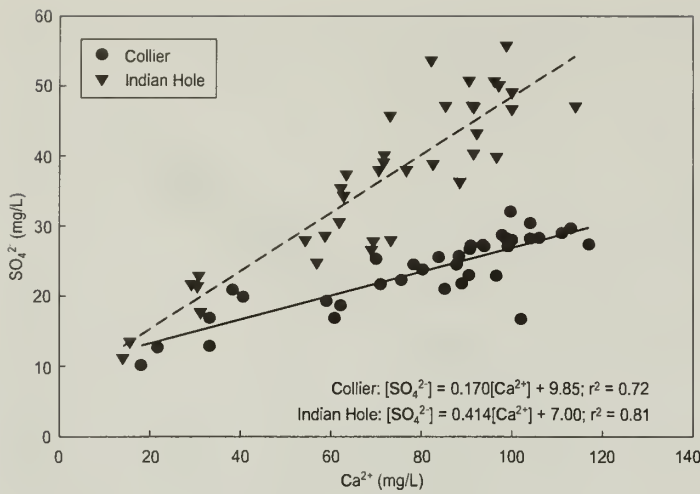
Figure 16 Relationships between Ca^{2+} and SO_4^{2-} concentrations for all samples collected at Indian Hole (dashed line) and Collier Springs (solid line). The data form two distinct trends, suggesting two distinctly different sources.
