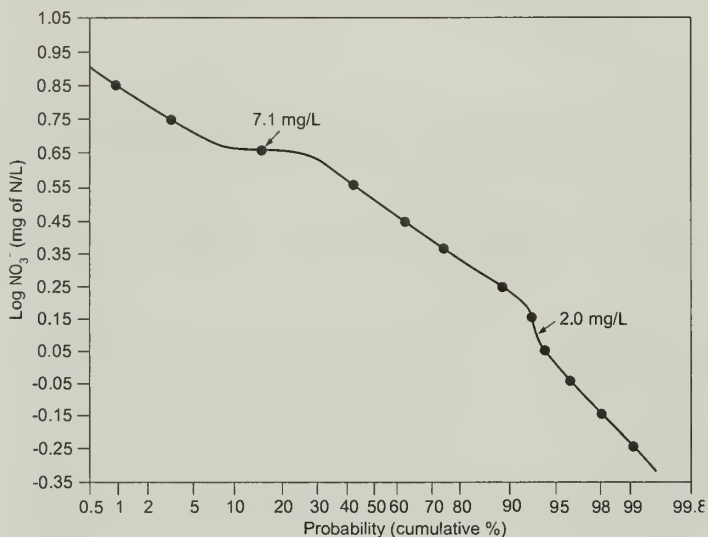
Figure 23 Cumulative probability plot of \text{NO}_3^- concentrations in water samples from springs, caves, and spring-fed surface water from southwestern Illinois. Threshold concentrations are 2.0 and 7.1 mg of N/L ( n = 219 ).
