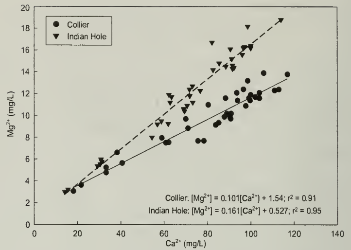
Figure 18 Calcium versus Mg^{2+} concentrations in water samples from Indian Hole (dashed line) and Collier Springs (solid line) showing two distinct trends.
