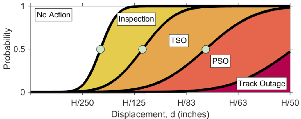
Figure 7.3. Fragility curves for Class I timber railroad bridges.
