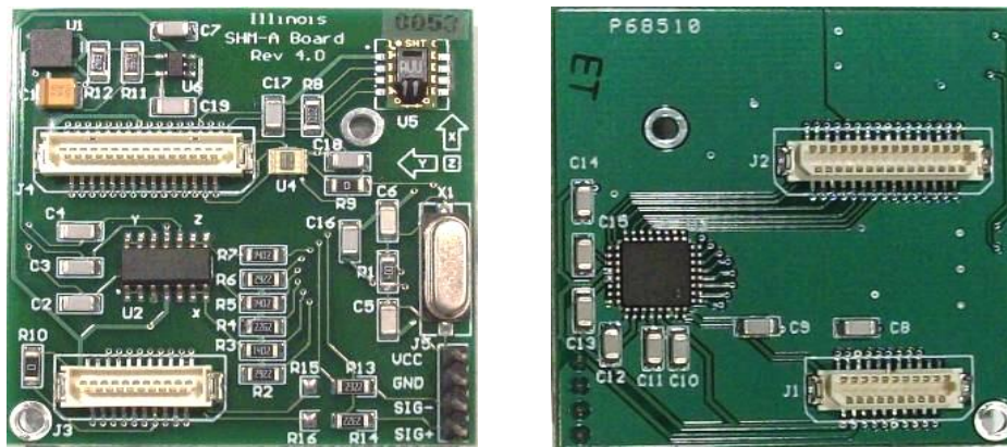
Figure 2.16 Multimetric sensor board (SHM-A board rev.4) for Imote2 platform by Rice et al. (2010); top (left) and bottom (right).
