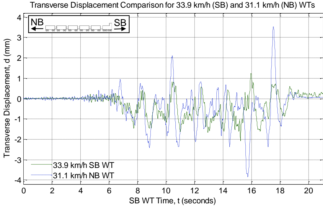
Figure 5.8. Comparison of transverse displacement under both SB and NB WTs.
