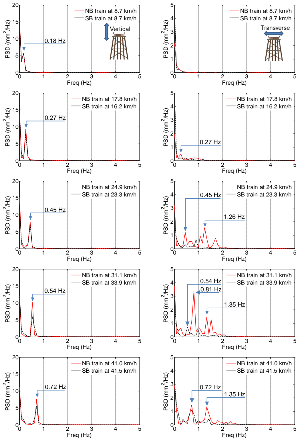
Figure 5.12. Frequency response to WTs in vertical (left) and transverse (right) direction
