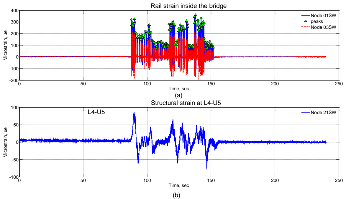
Figure 8.12 Strain collected during autonomous monitoring: (a) rail strain, (b) structural strain.
