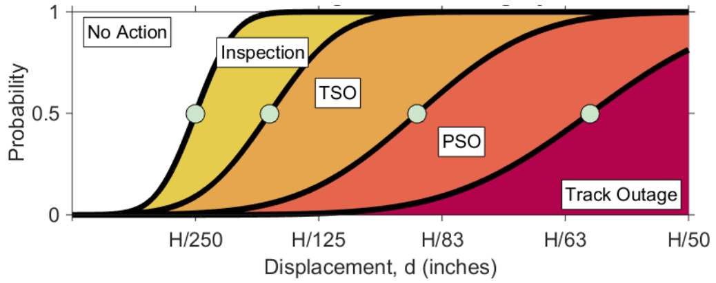
Figure 7.4. Fragility curves for Class II timber railroad bridges.
