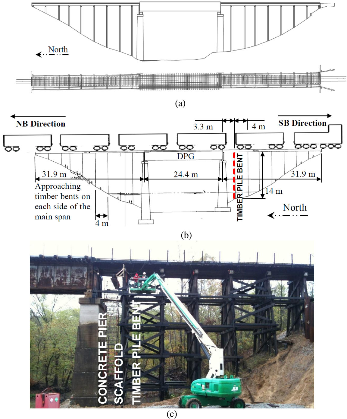
Figure 5.1 Bridge views: (a) CAD elevation and plan view, (b) bridge dimensions and traffic, (c) timber trestle South approach: concrete pier, scaffold, and timber pile bent during sensor deployment.
