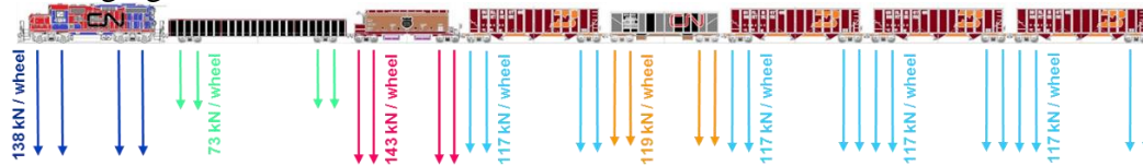
Figure 8.7 Work train wheel loading scheme.
