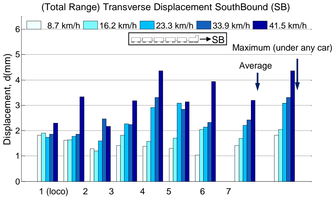
Figure 5.9. Total transverse displacement range vs. input loads for SB WTs.
