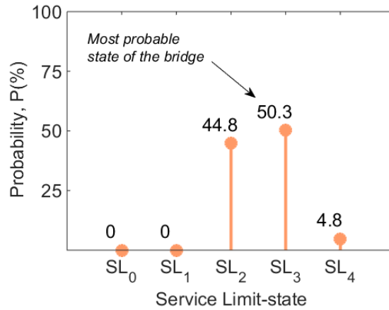
Figure 7.9. Updated distribution P^{\text{updated}}(SL = k | D = d_{\text{measured}}, Z = j) of SL_k , given the measured displacement D = d_{\text{measured}} and the track class Z_j .
