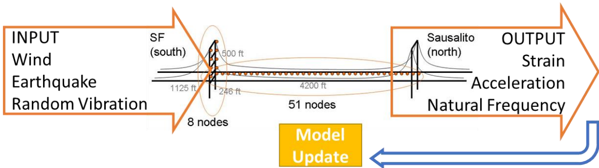
Figure 2.12. Monitoring of the Golden Gate Bridge (Kim et al. 2015).
