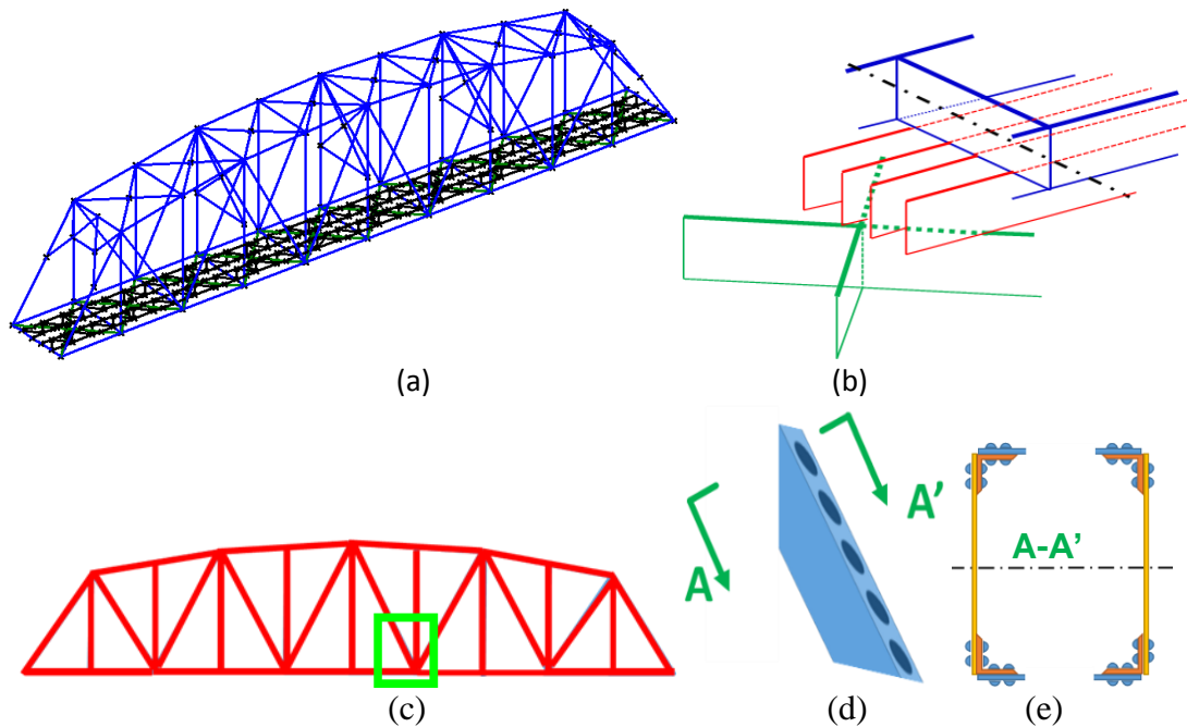
Figure 8.13. FE model: (a) 3D view, (b) floor system, (c) elevation, (d) element, and (e) gross area.
