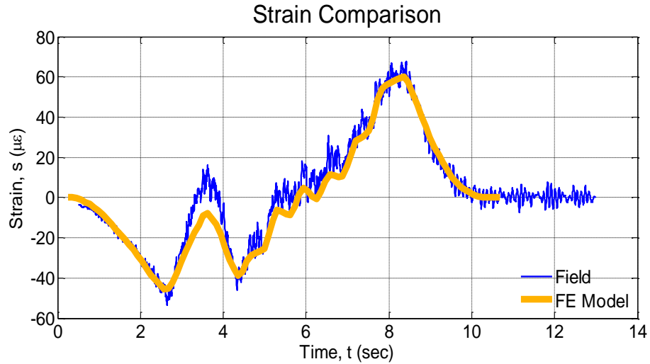
Figure 8.14. Strain prediction for L4-U5 diagonal member using FE model.
