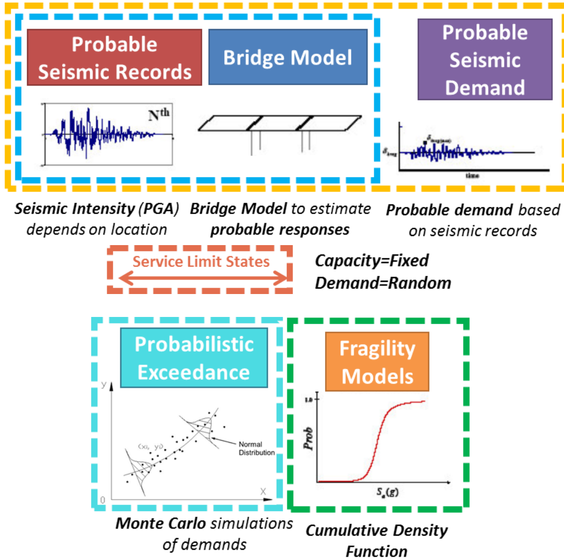
Figure 4.7. Seismic fragility.
