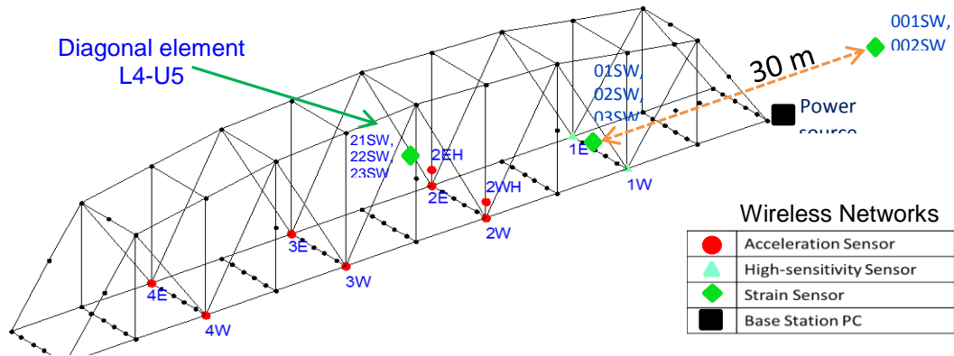
Figure 8.4. WSSs layout.
