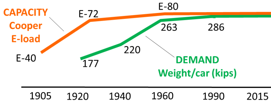
Figure 2.1. Railroad bridge capacity and weight/car demand comparison.
