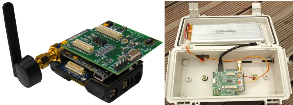
Figure 6.3. (a) Stacked WSS board with battery board and SHM-A sensor board, (b) enclosure for campaign monitoring applications (ISHMP 2014).
