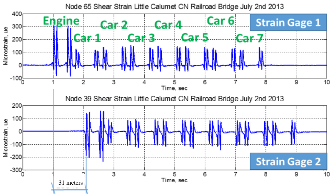
Figure 8.6 Estimation of train speed using two wireless strain gages installed in the rail.
