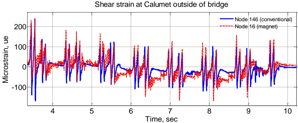
Figure 8.9 Comparison between conventional and magnetic strains at rail.
