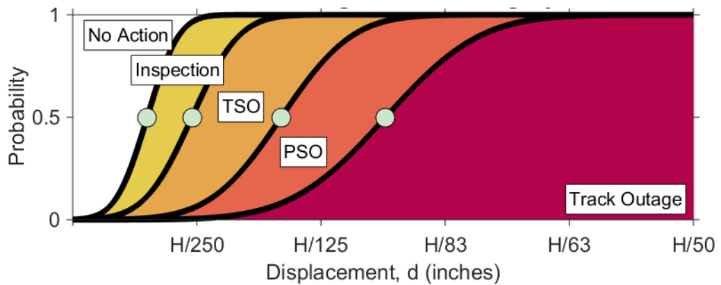
Figure 7.6. Fragility curves for Class IV timber railroad bridges.
