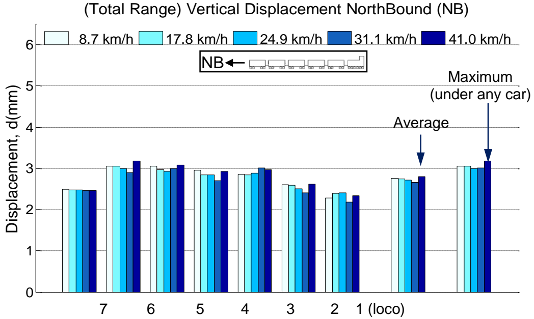
Figure 5.6. Total vertical displacement range vs. input loads for NB WTs.
