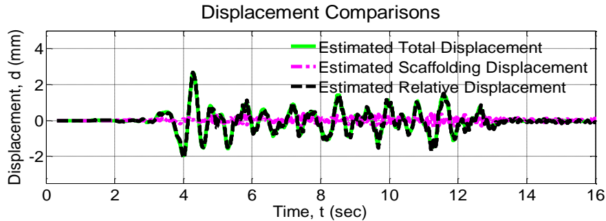
Figure 6.6. Estimated displacements of scaffolding under NB WT at 41.0 km/h
