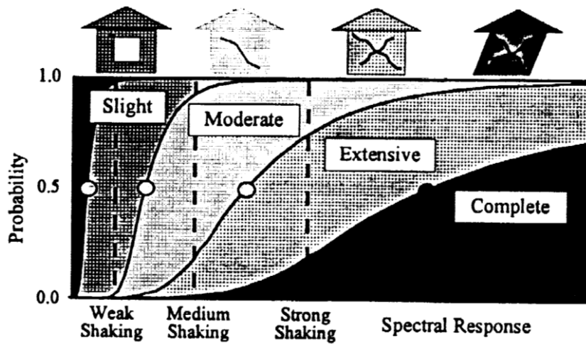
Figure 2.20. Fragility curve example for seismic engineering.
