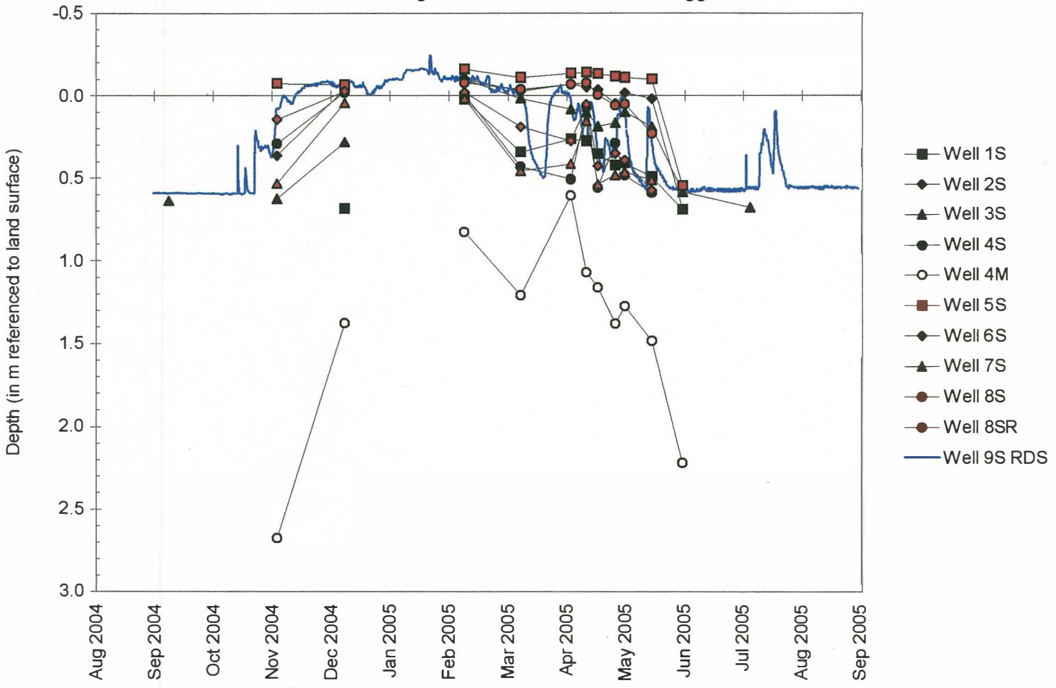
Depth to Water in Monitoring Wells and the RDS Data Logger
