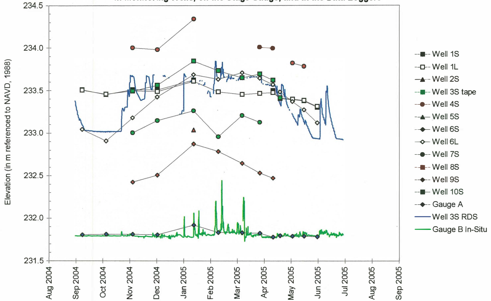
Water-Level Elevations in Monitoring Wells, on the Stage Gauge, and at the Data Loggers
