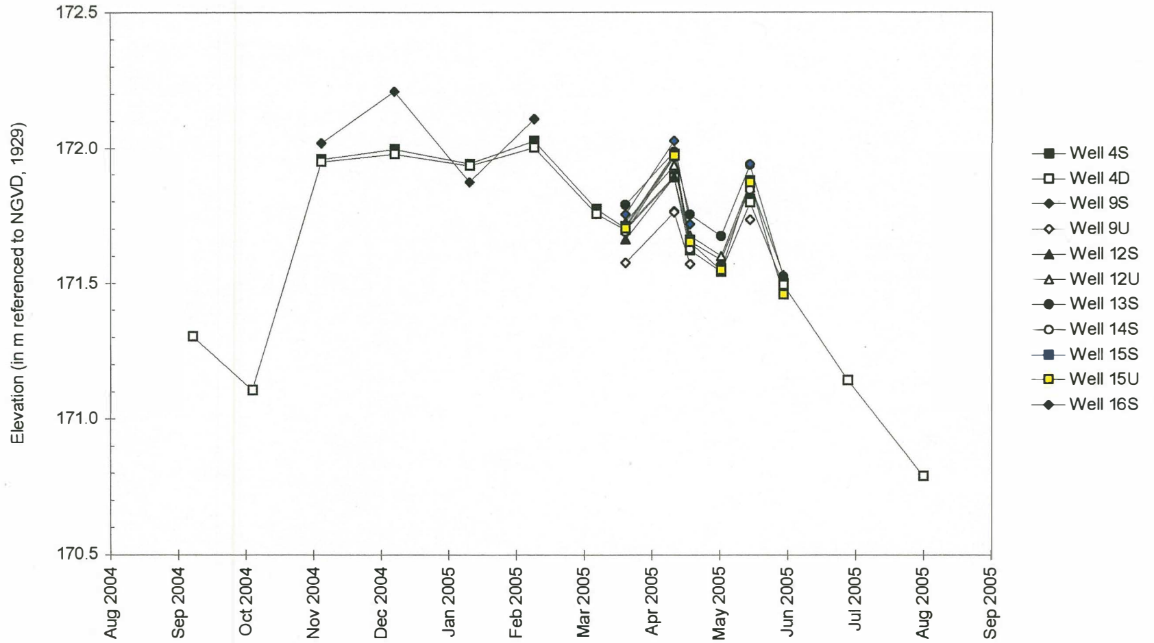
Water-Level Elevations in Selected Monitoring Wells
