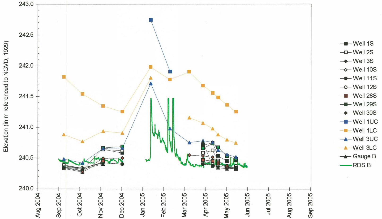
Water-Level Elevations at Site 1
