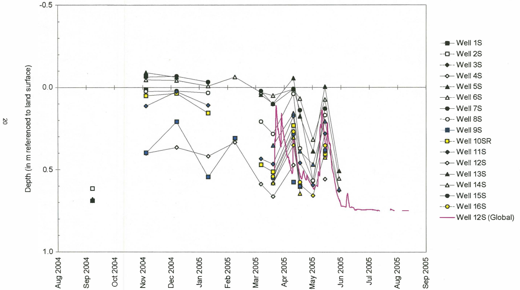
Depths to Water in Soil-Zone Monitoring Wells
