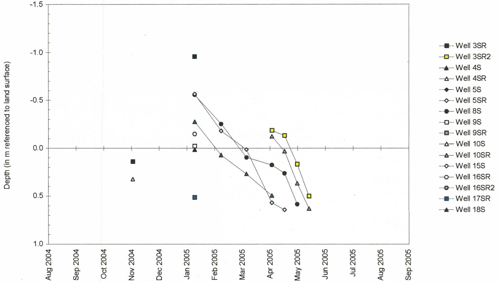
Depth to Water in Selected Monitoring Wells in the Floodplain Forest
