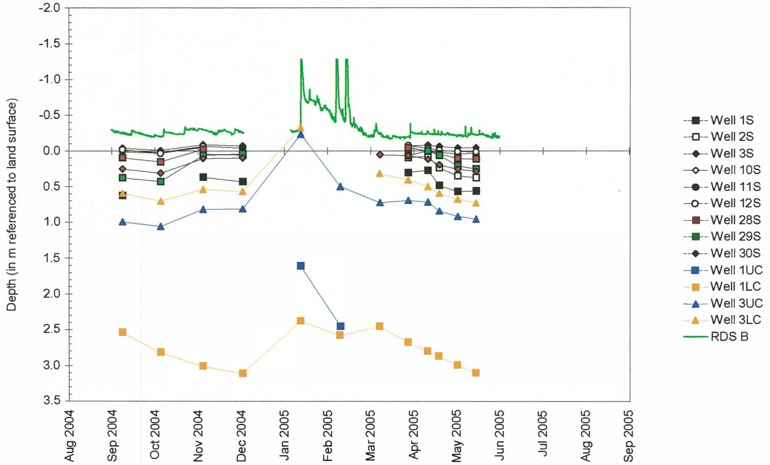
Depth to Water at Site 1
