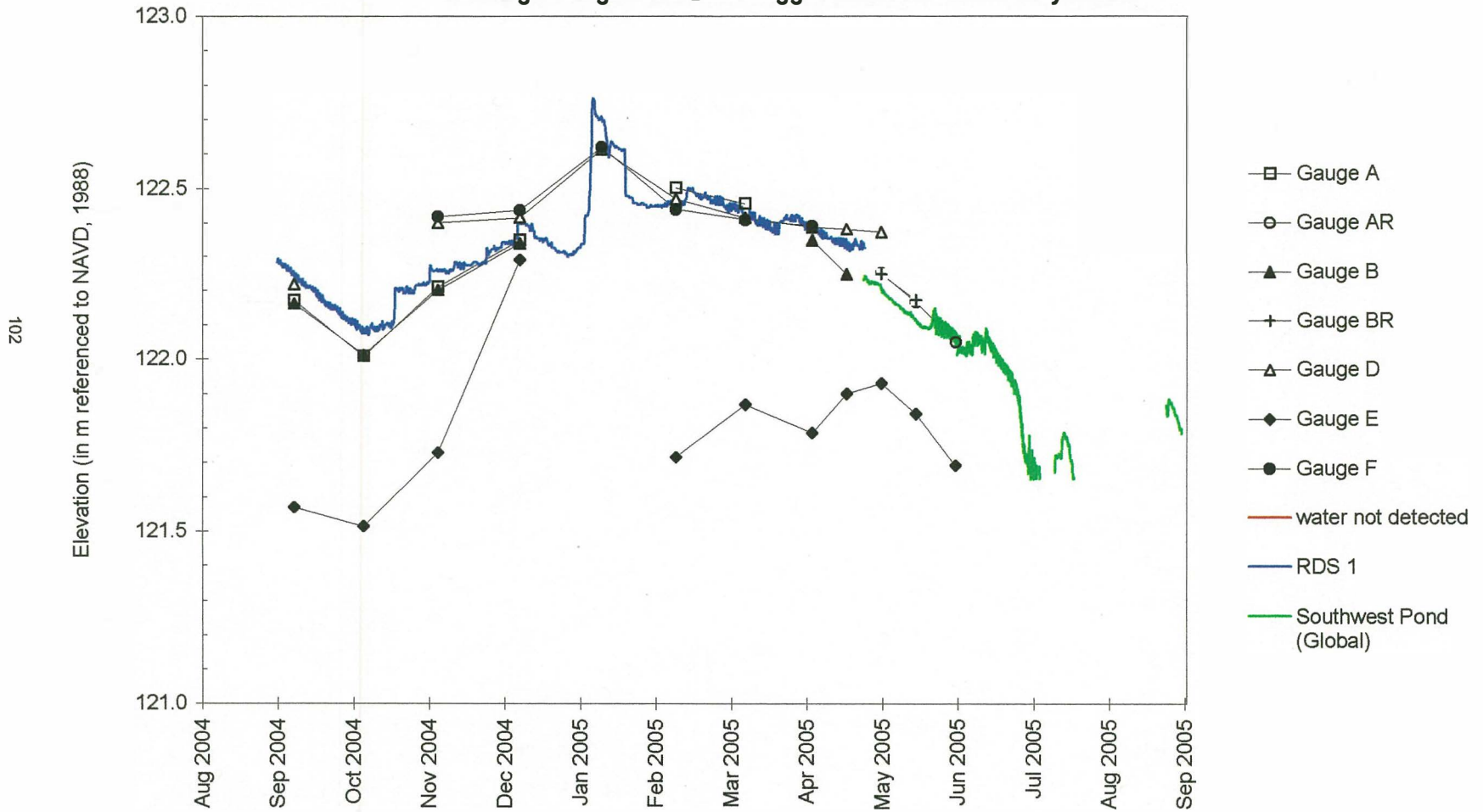
Water-Level Elevations on Stage Gauges and Data Loggers in the Fairmont City 1 Site
