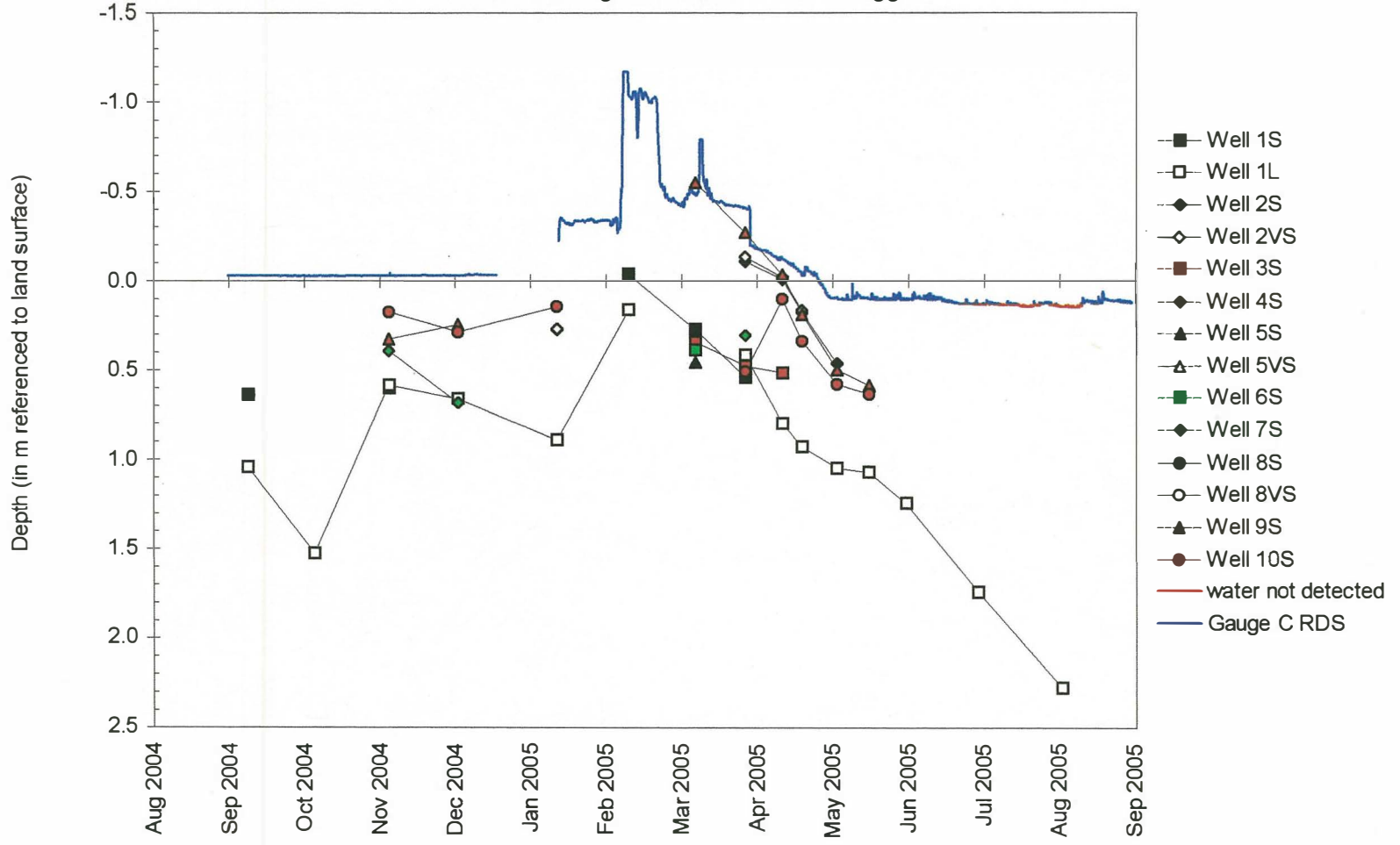
Depth to Water in Monitoring Wells and the Data Loggers
