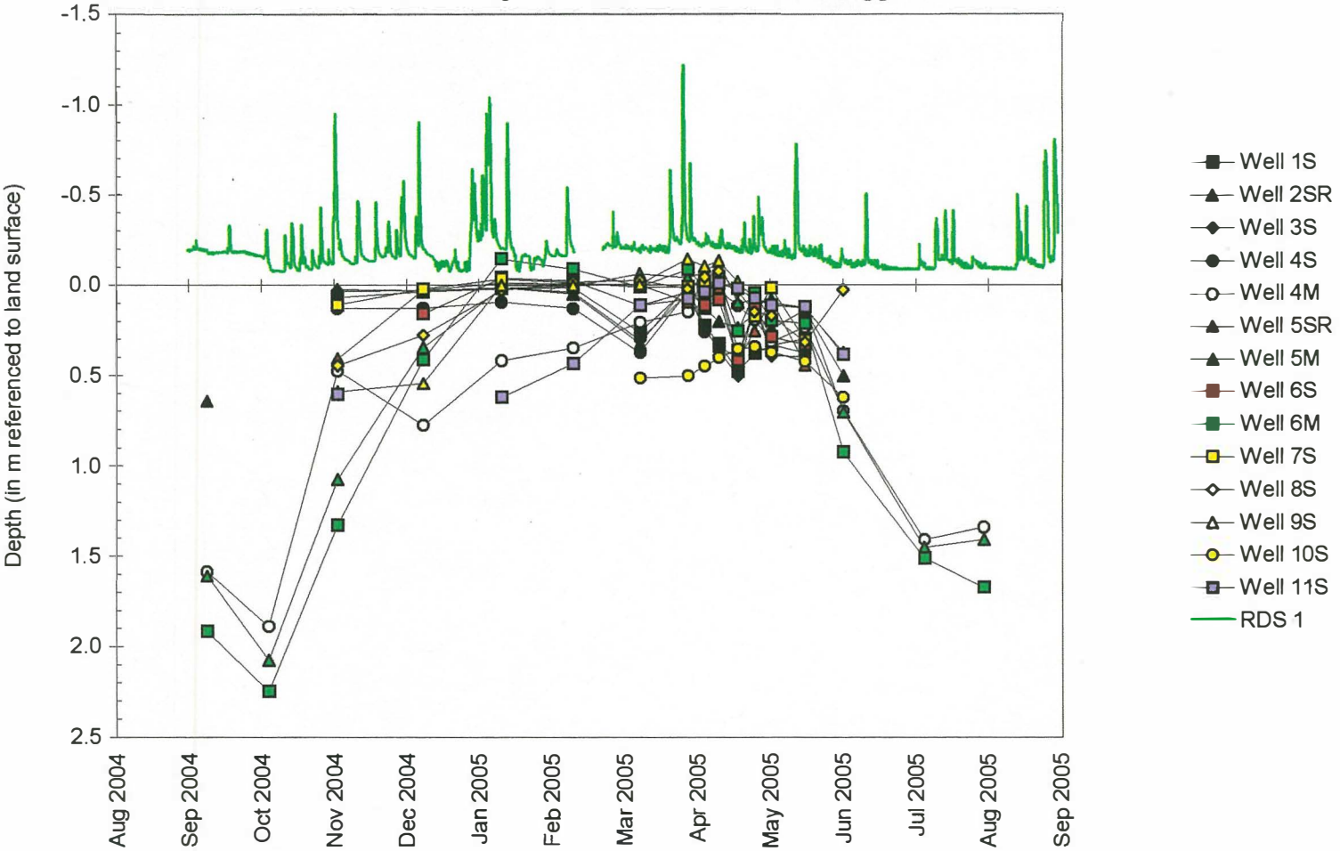
Depth to Water in Monitoring Wells and at the RDS Data Logger
