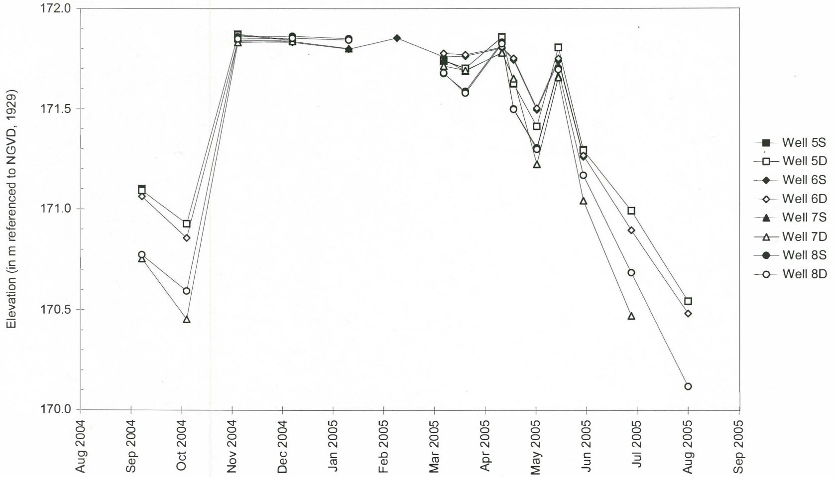
Water-Level Elevations in Selected Monitoring Wells
