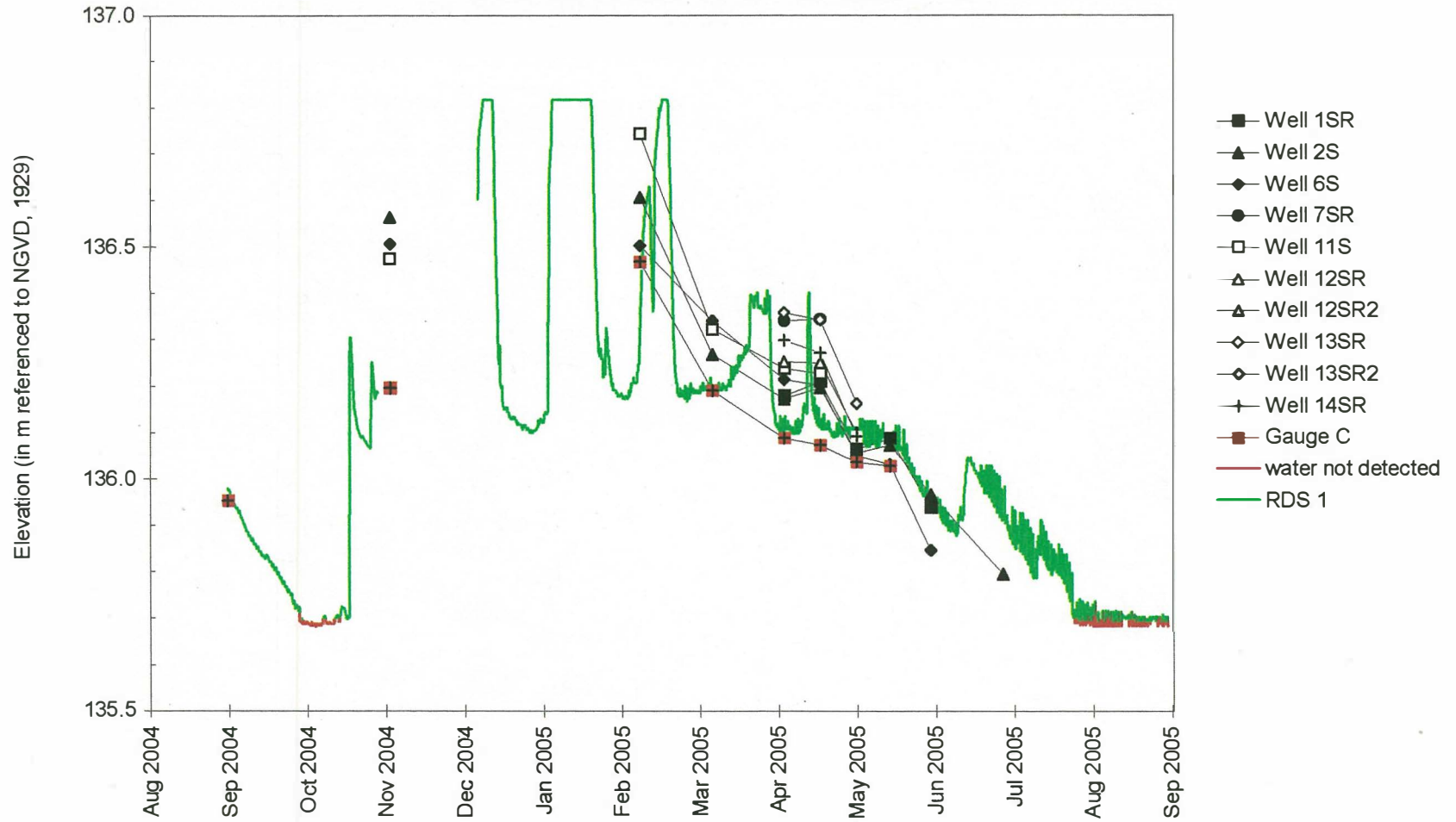
Water-Level Elevations in Selected Monitoring Wells in the Farm Field
