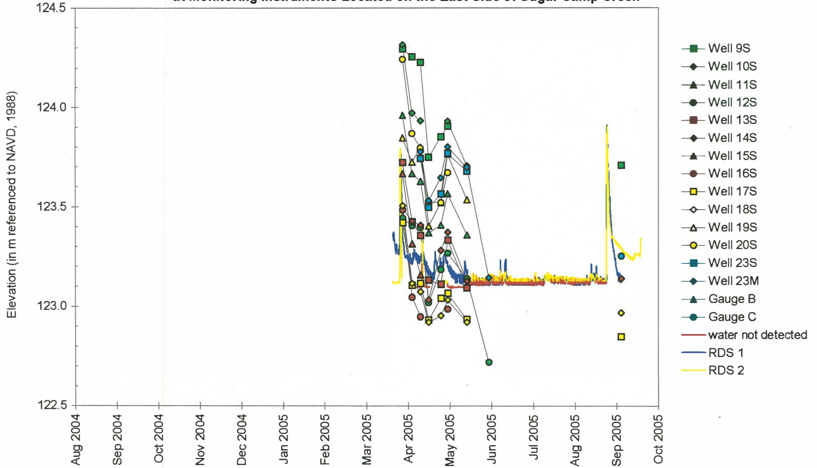
Water-Level Elevations at Monitoring Instruments Located on the East Side of Sugar Camp Creek
