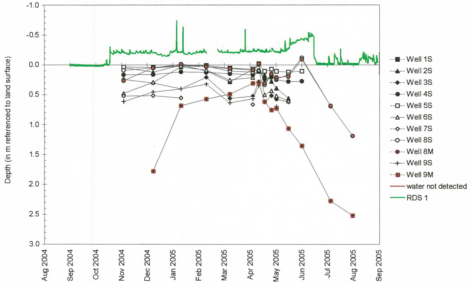
Depth to Water in Selected Monitoring Wells and at the RDS Data Logger
