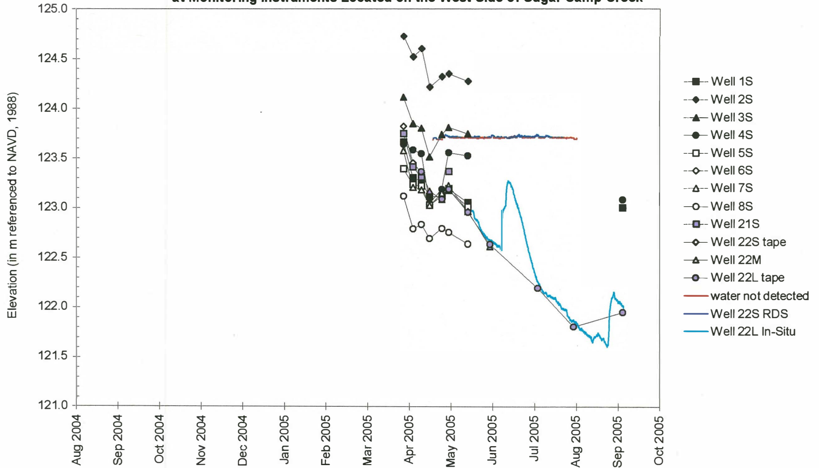
Water-Level Elevations at Monitoring Instruments Located on the West Side of Sugar Camp Creek
