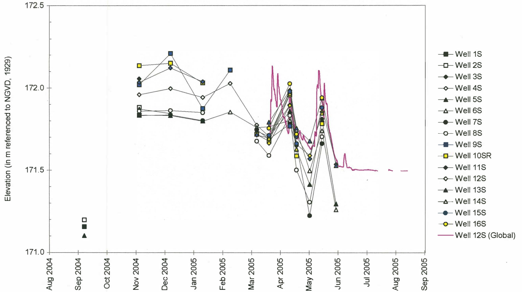
Water-Level Elevations in Soil-Zone Monitoring Wells
