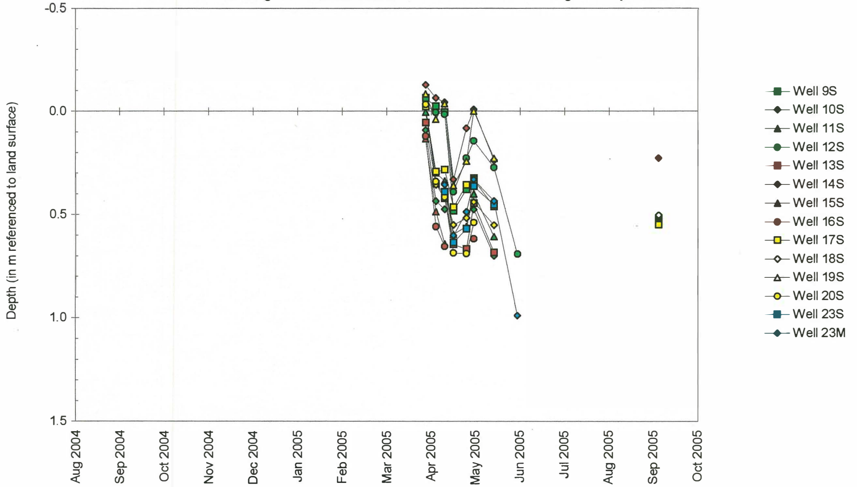
Depth to Water at Monitoring Instruments Located on the East Side of Sugar Camp Creek
