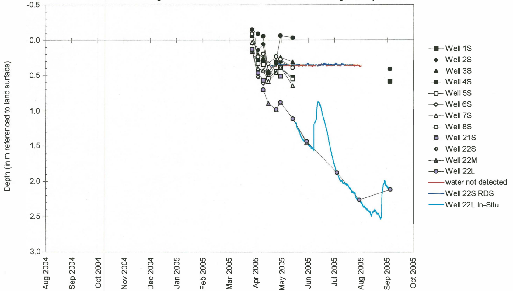
Depth to Water at Monitoring Instruments Located on the West Side of Sugar Camp Creek
