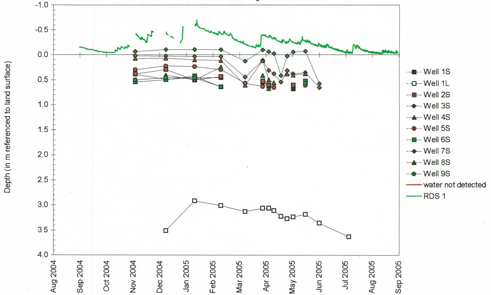
Depth to Water in Monitoring Wells
