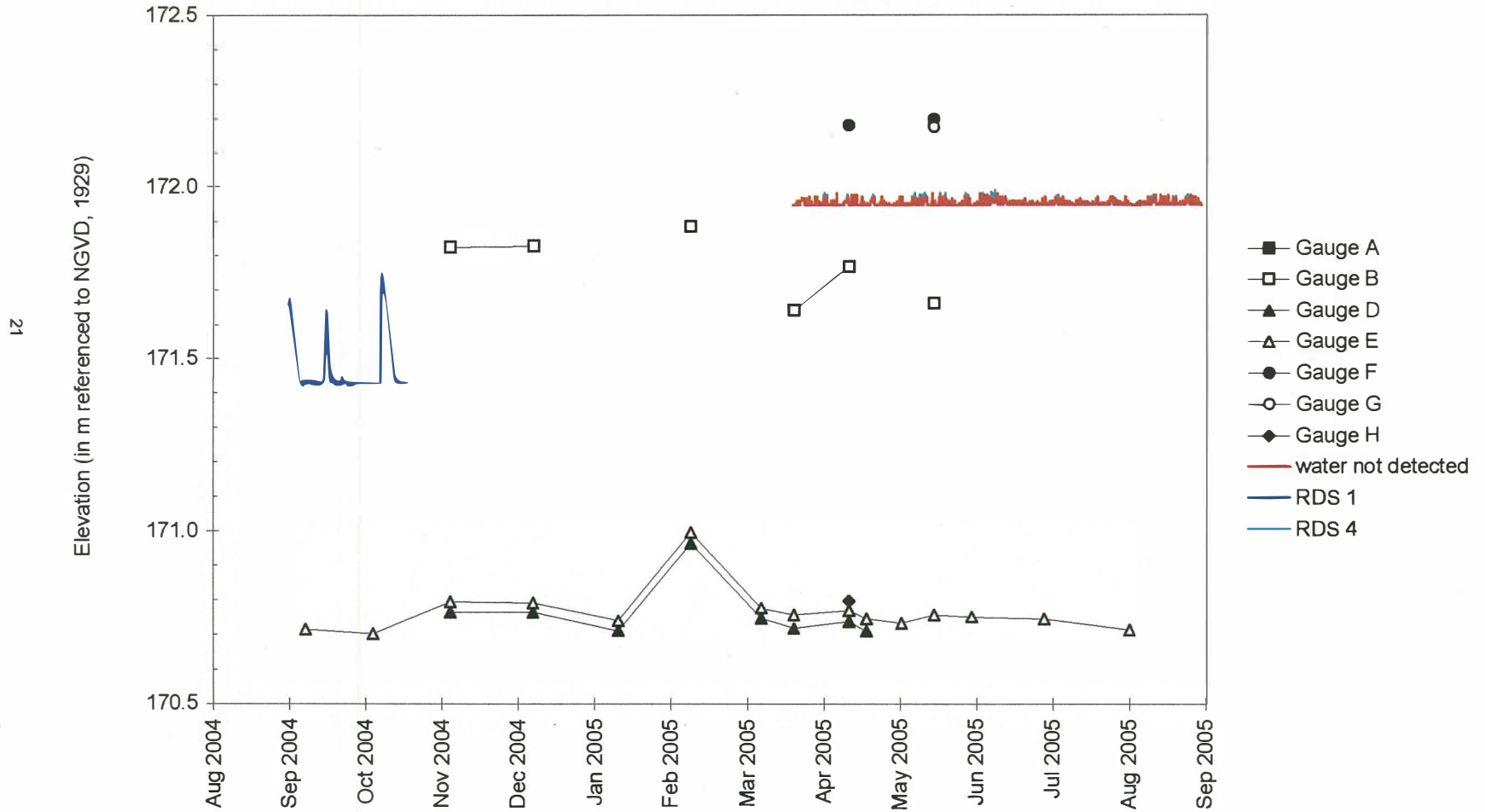
Water-Level Elevations at Surface-Water Gauges
