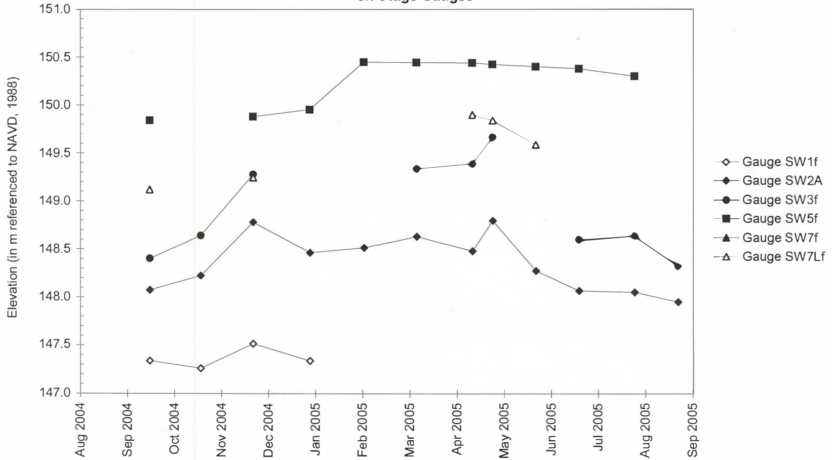
Water-Level Elevations on Stage Gauges
