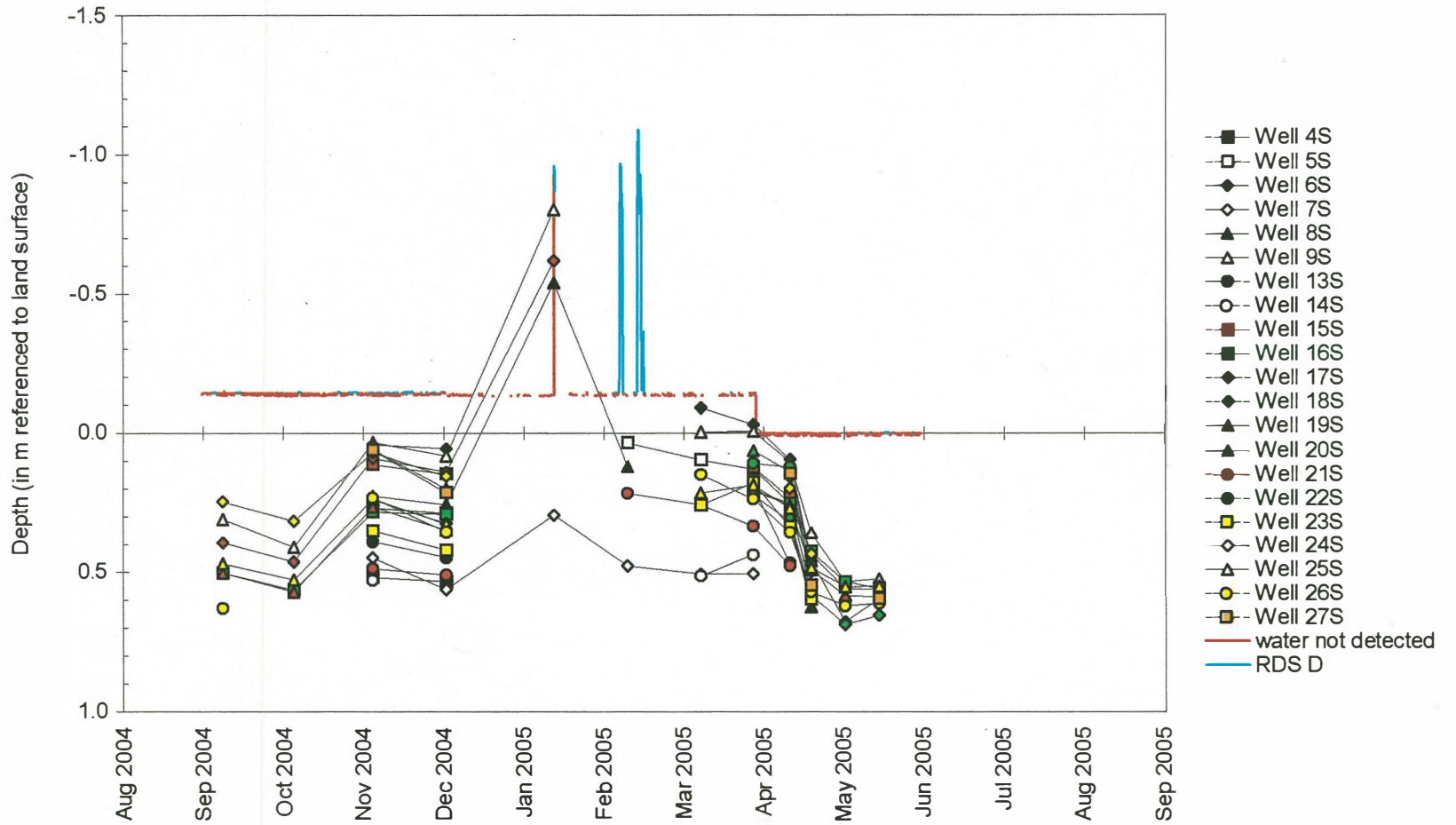
Depth to Water at Site 2
