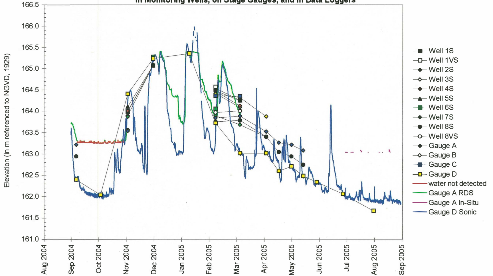
Water-Level Elevations in Monitoring Wells, on Stage Gauges, and in Data Loggers
