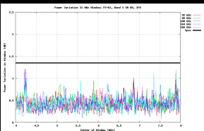
Fig 4: (Left) The plot shows IF frequency (GHz) vs. power (dB) for band 3, and is looking for spikes and large variations between the desired IF window (4 – 8 GHz). Each LO frequency for the band is represented. (Right) The plot shows the power variation (dB) over a 31 MHz window at the center frequency of the window (GHz). Each LO frequency for the band is represented, along with the specification line, at 1.35 dB.
