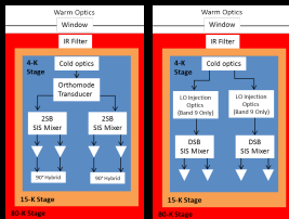
Fig 2: These are diagrams of the Cold Cartridge Assembly, which processes the sky signal to be sent to the back end of the antenna. (Left) Bands 3-7. (Right) Bands 8-10.
