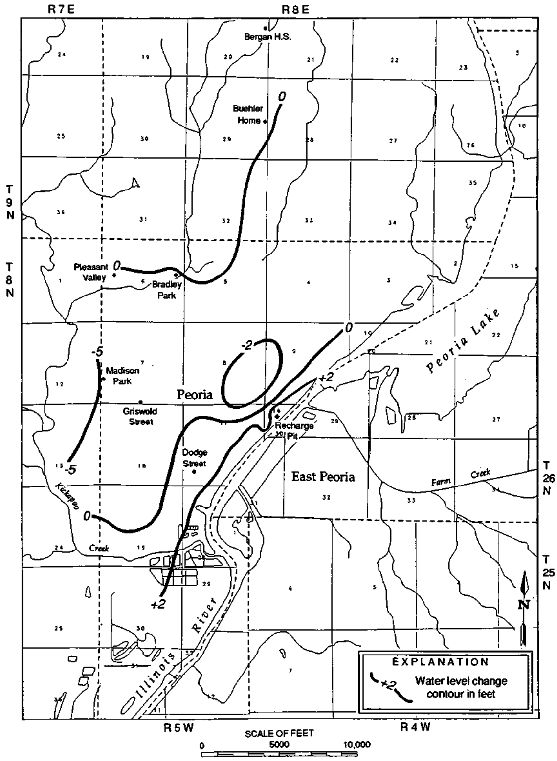
Figure 13. Ground-water level changes, August 1966-April 1967
