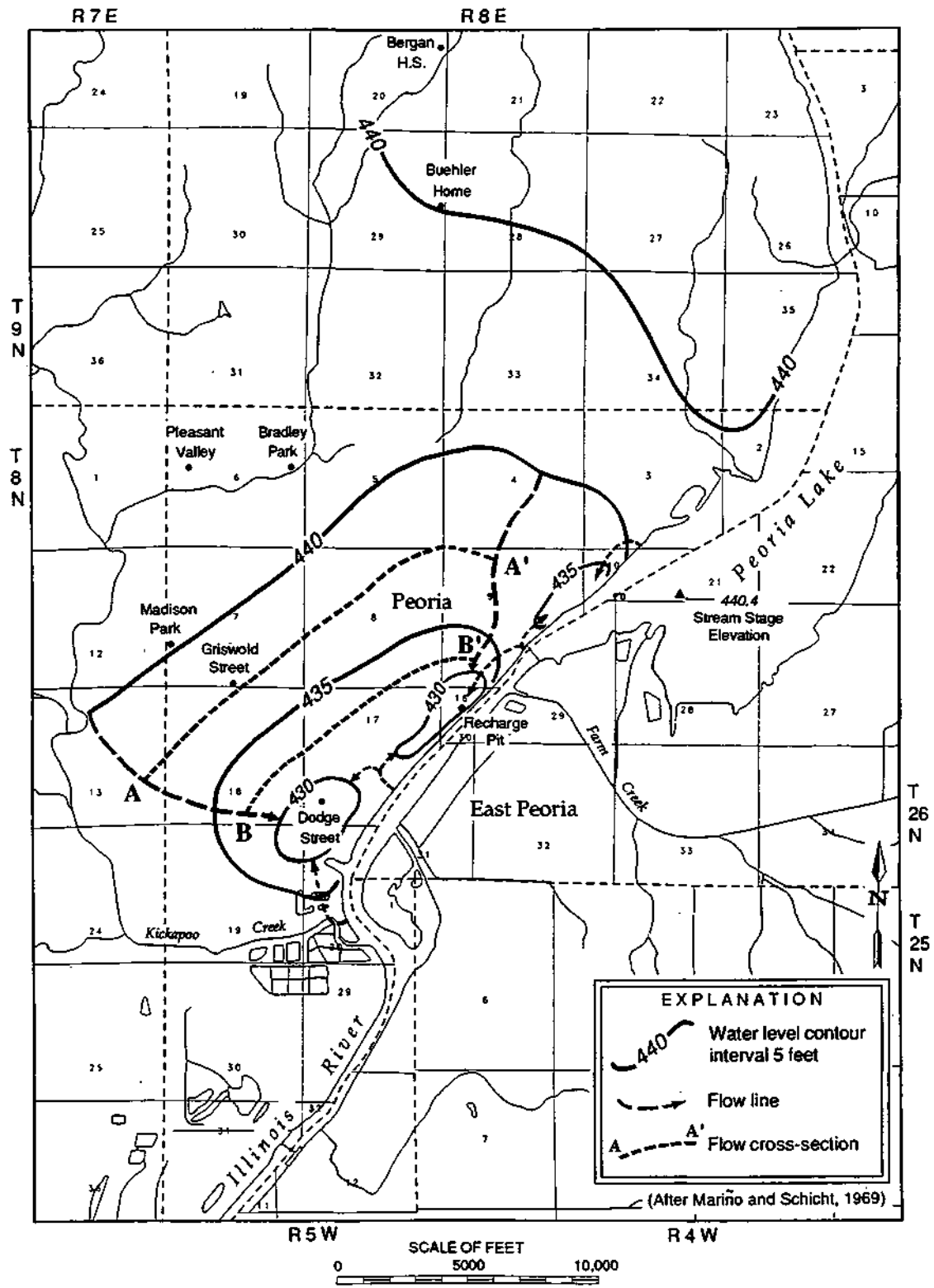
Figure 8. Water-table contour map, August 1966
