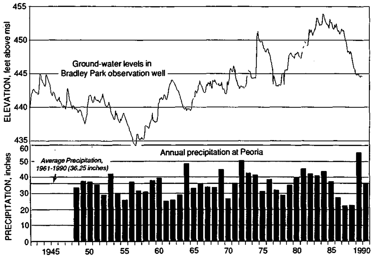
Figure 10. Ground-water levels at Bradley Park well, and annual precipitation at Peoria Airport
