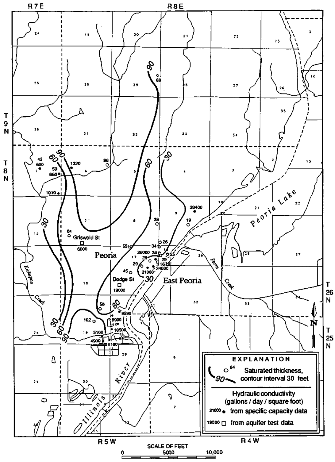
Figure 6. Aquifer hydraulic conductivity and saturated thickness
