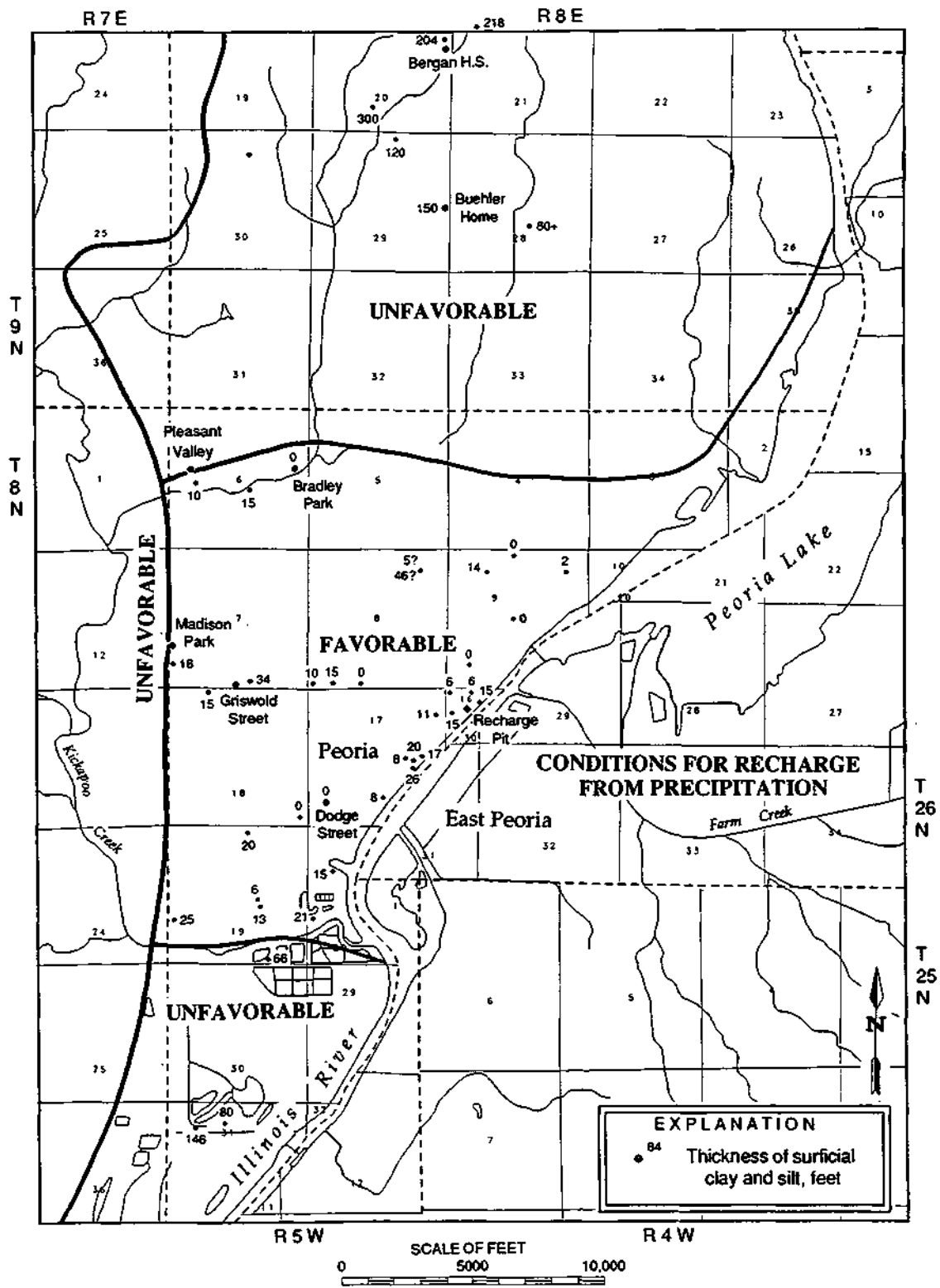
Figure 11. Conditions for recharge from precipitation
