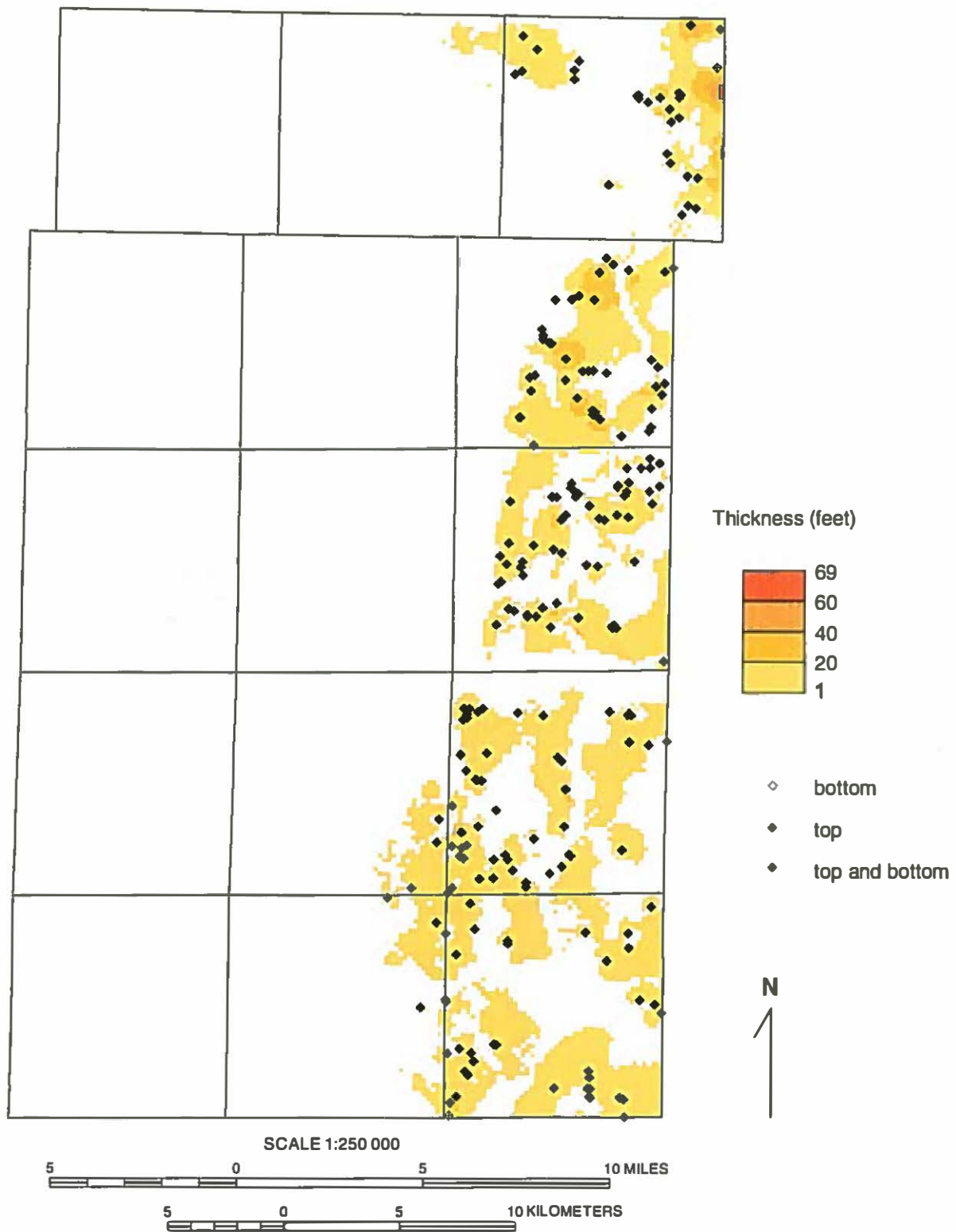
Figure 22 Isopach map of the sub-Yorkville tongue of the Henry Formation in Kane County and the distribution of primary wells used in mapping the unit.
