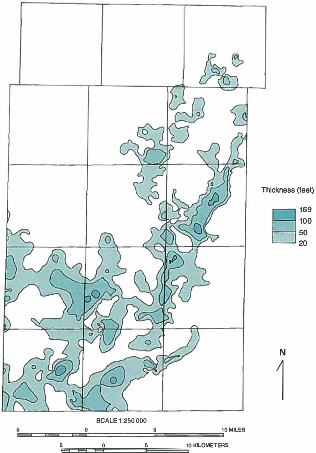
Figure 53 Distribution and thickness of the St. Charles aquifer in Kane County.
