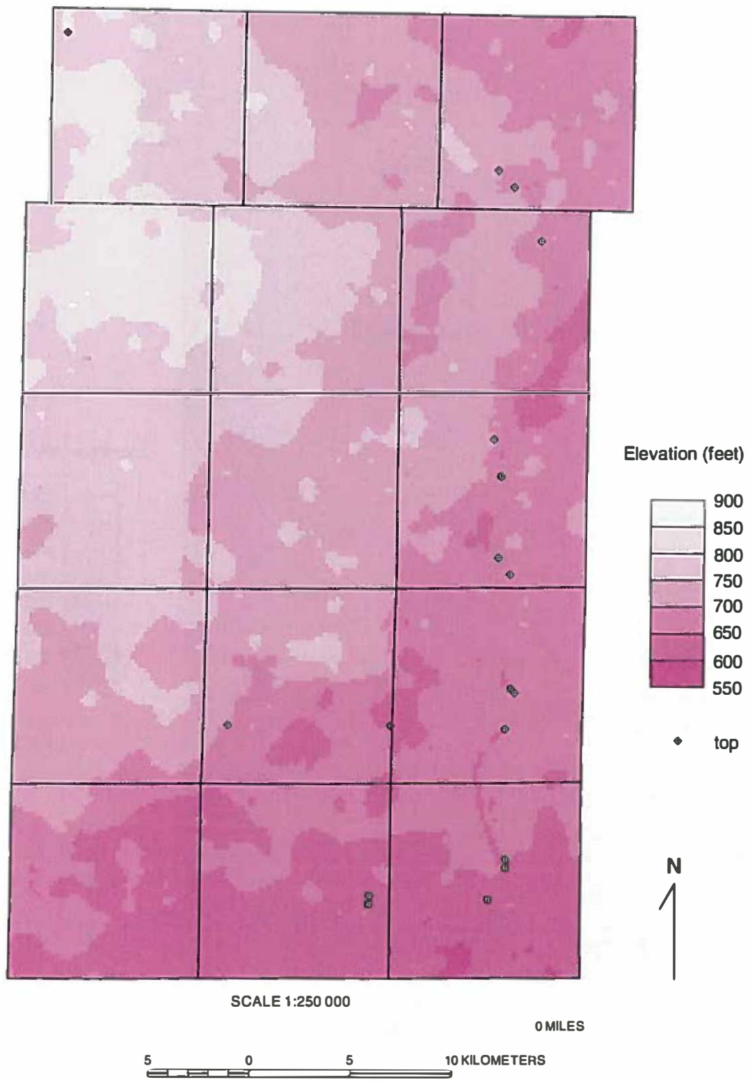
Figure 32 Elevation grid of the upper surface of the Glasford Formation in Kane County and the distribution of synthetic data points used mapping the surface.
