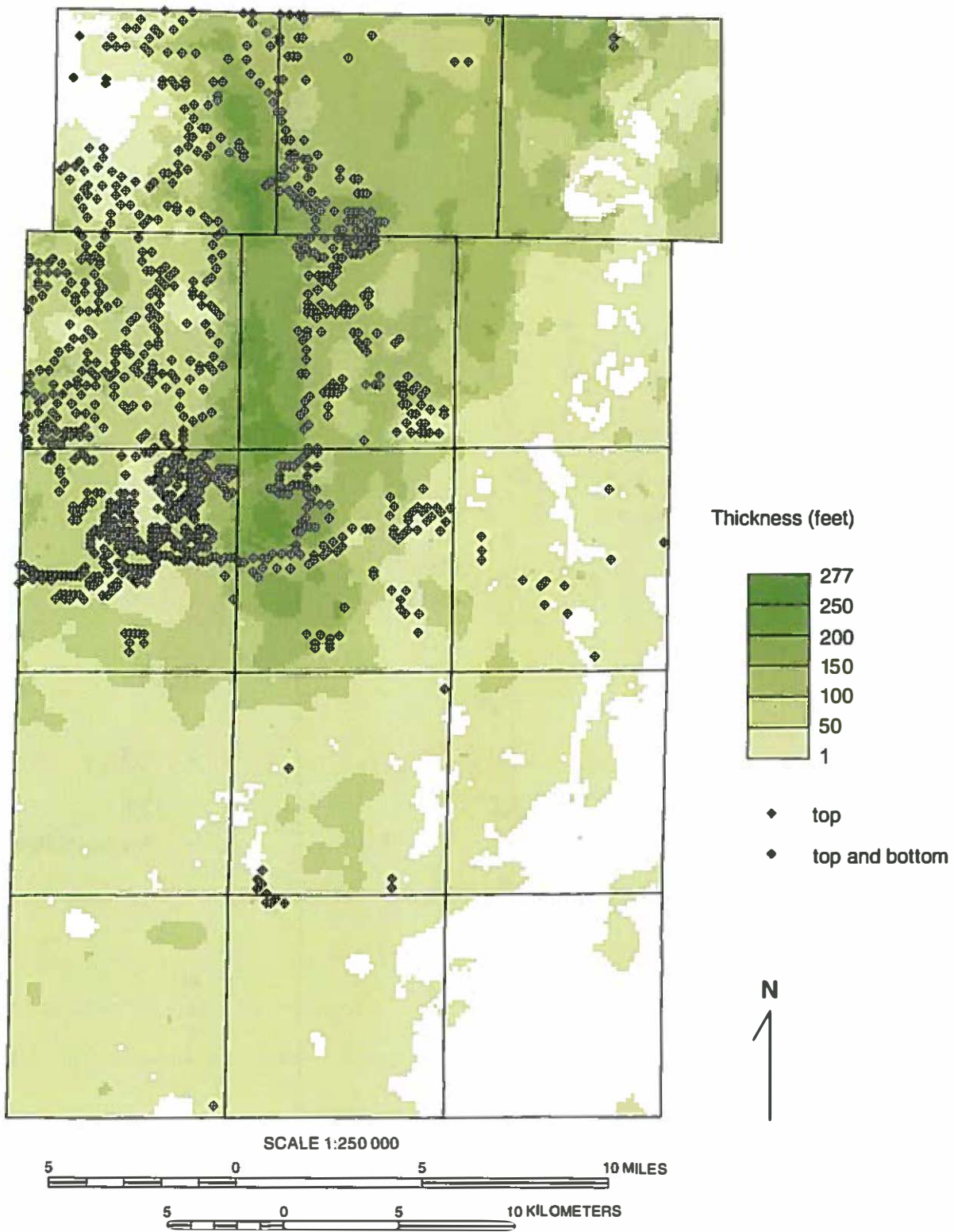
Figure 28 Isopach map of the Tiskilwa Formation in Kane County and the distribution of synthetic data points used in mapping the unit.
