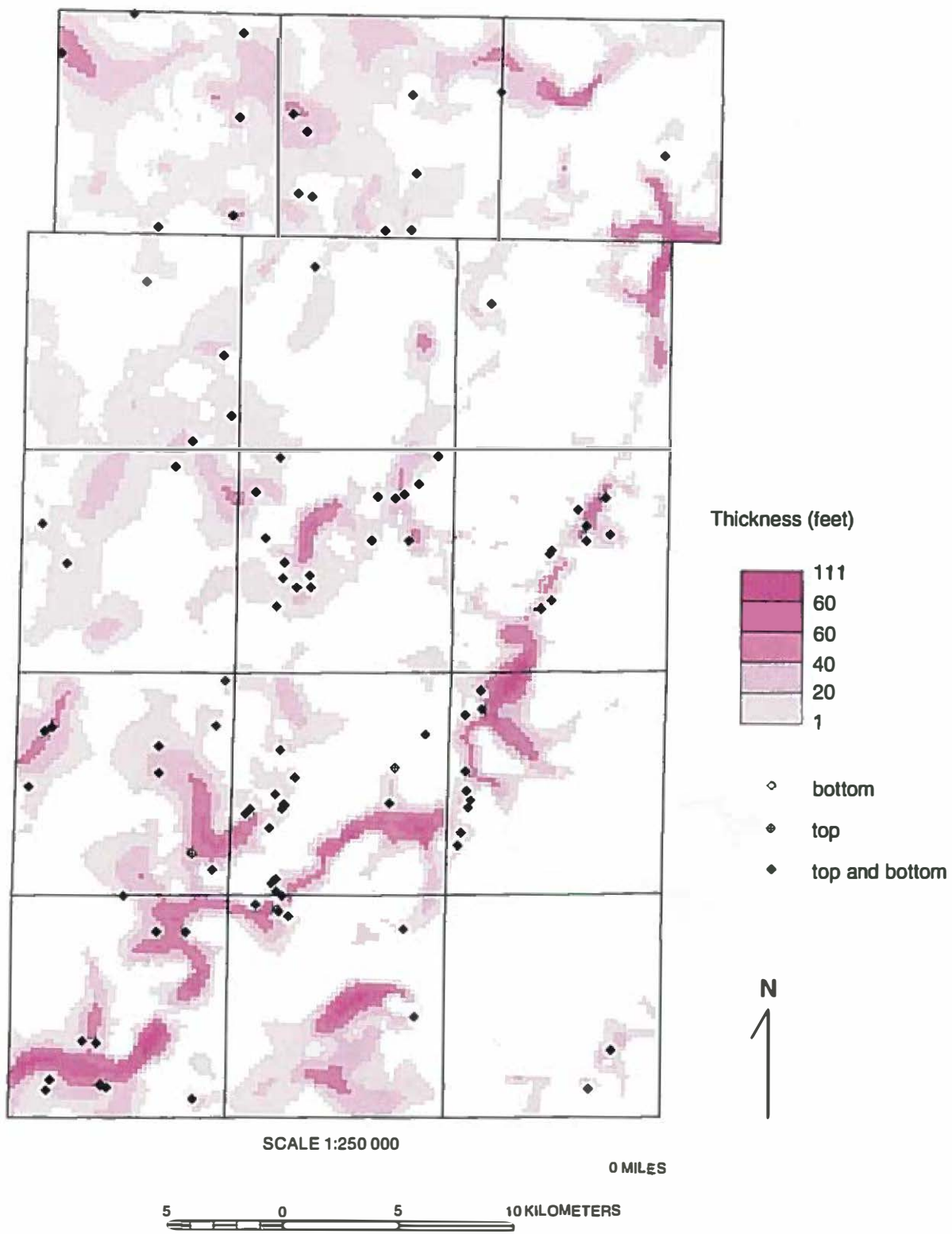
Figure 38 Isopach map of the lower fine-textured unit of the Glasford Formation in Kane County and the distribution of primary wells used in mapping the unit.
