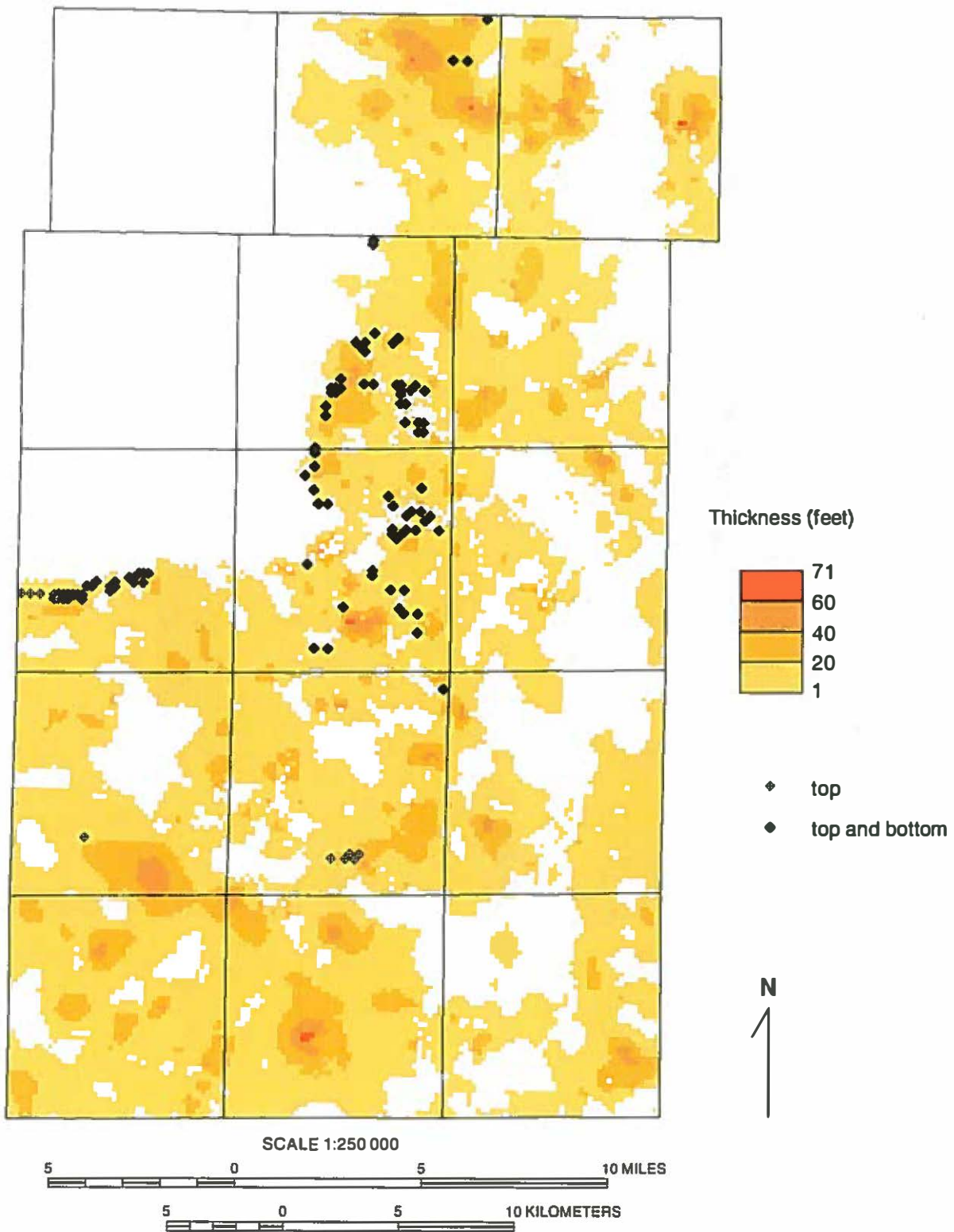
Figure 26 Isopach map of the sub-Batestown tongue of the Henry Formation in Kane County and the distribution of synthetic data points used in mapping the unit.
