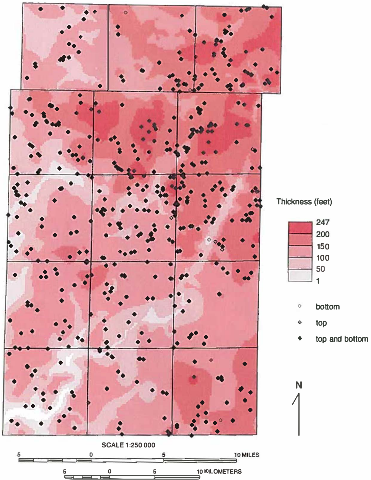
Figure 43 Isopach map of the Maquoketa Group of the Ordovician System in Kane County and the distribution of primary wells used in mapping the unit.
