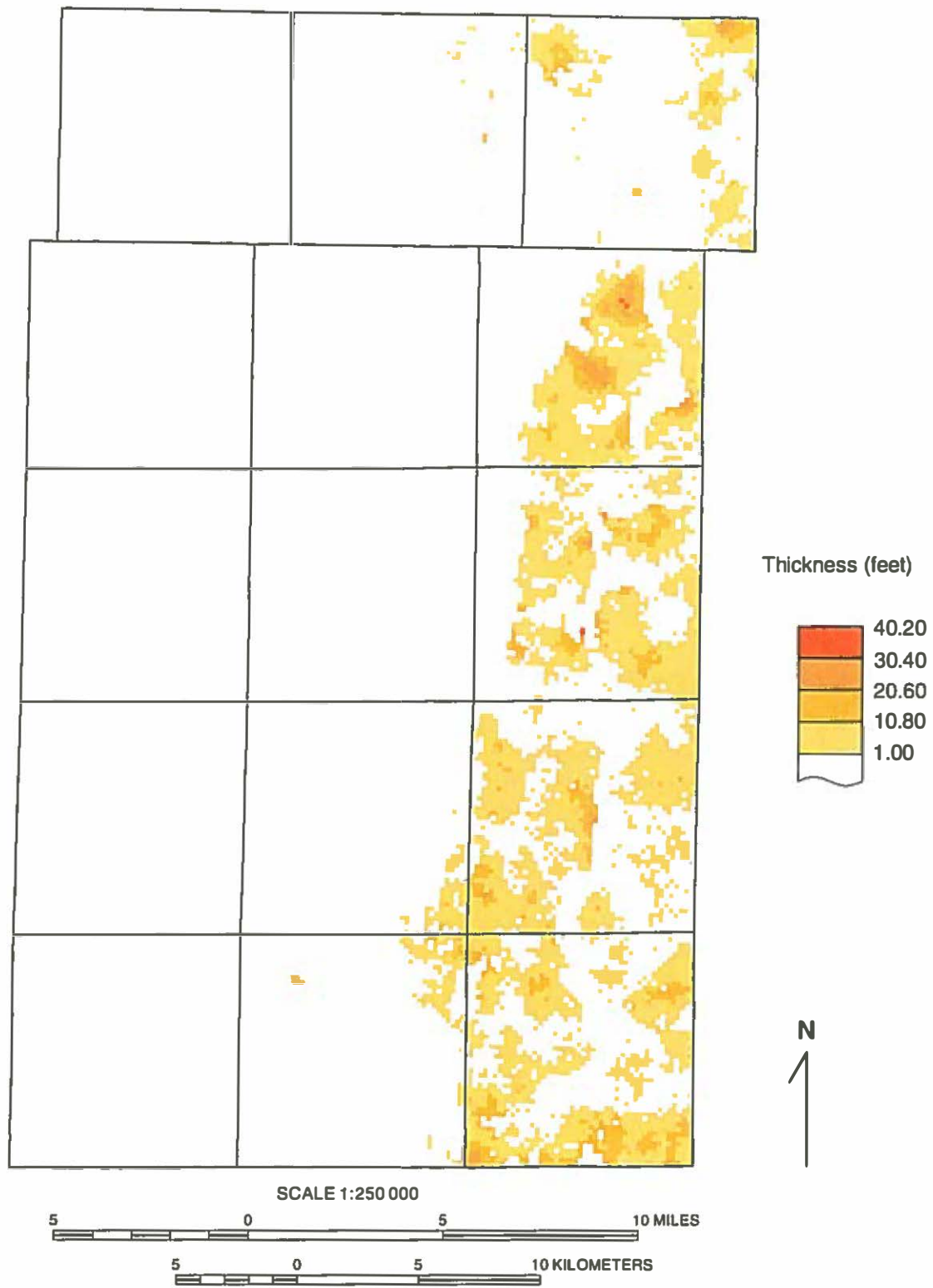
Figure A1 Simulation map of the thickness of the sub-Yorkville tongue of the Henry Formation showing small local variability.
