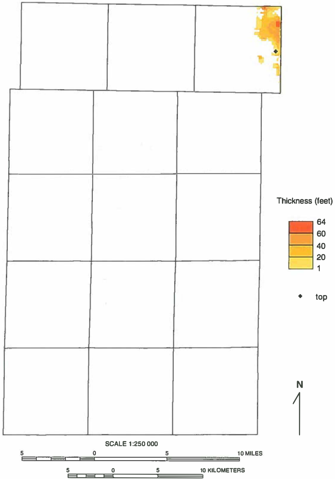
Figure 19 Isopach map of the Beverly Tongue of the Henry Formation and the distribution of synthetic data points used in mapping the unit.
