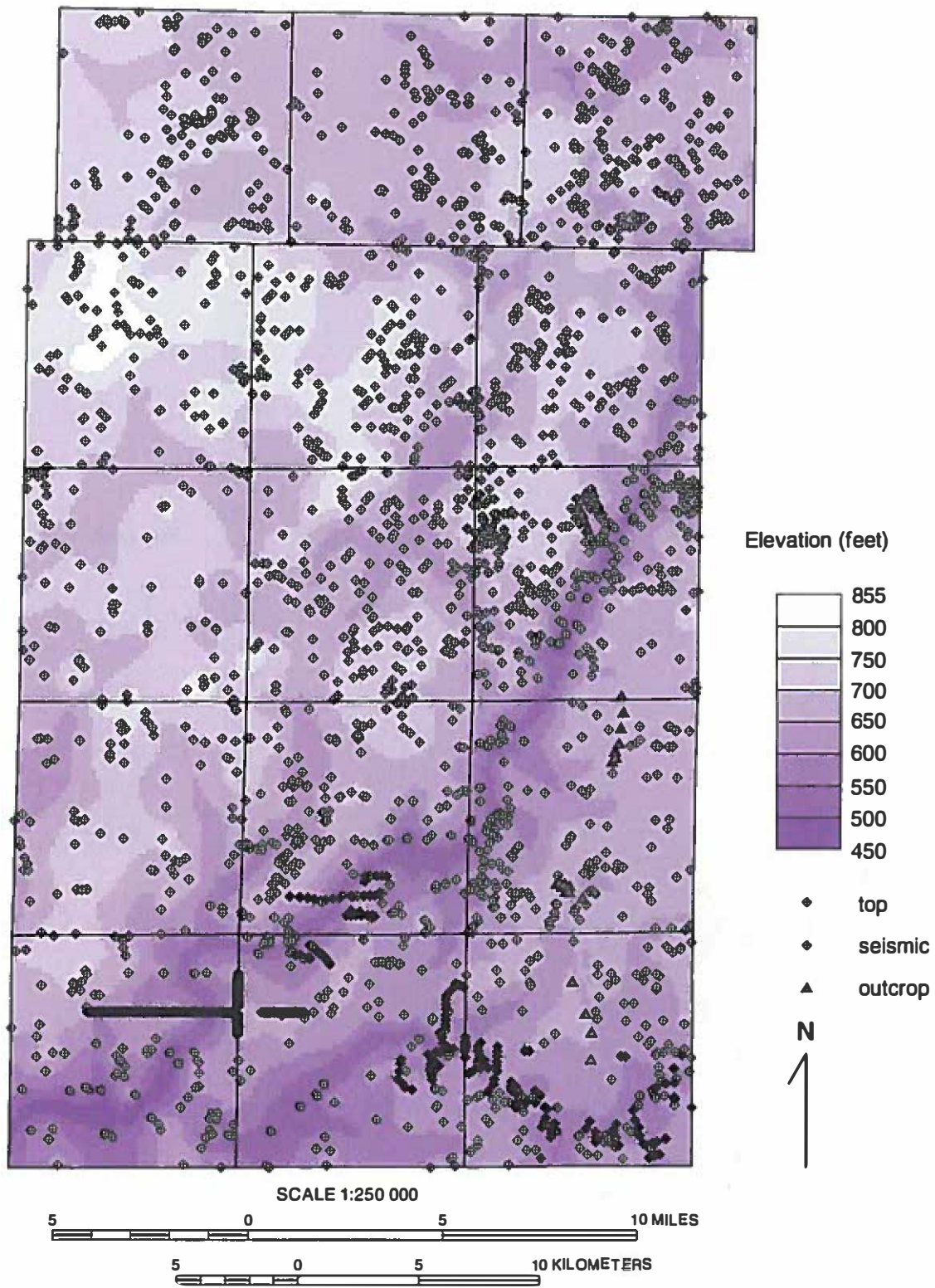
Figure 39 Bedrock topography of Kane County and the distribution of primary wells, seismic data, and outcrops used in mapping the surface.
