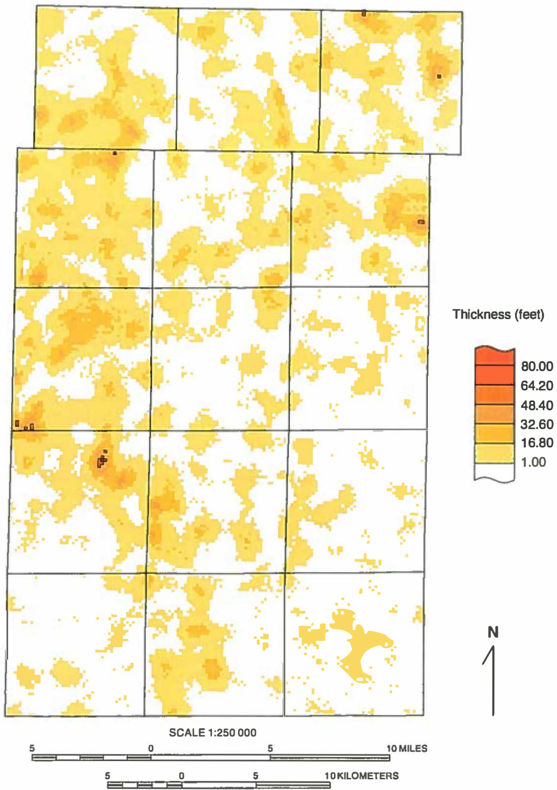
Figure A16 Thickness of the Ashmore Tongue of the Henry Formation showing small local variability. This map is the 50th percentile map when Step 1 results are sorted on total thickness.
