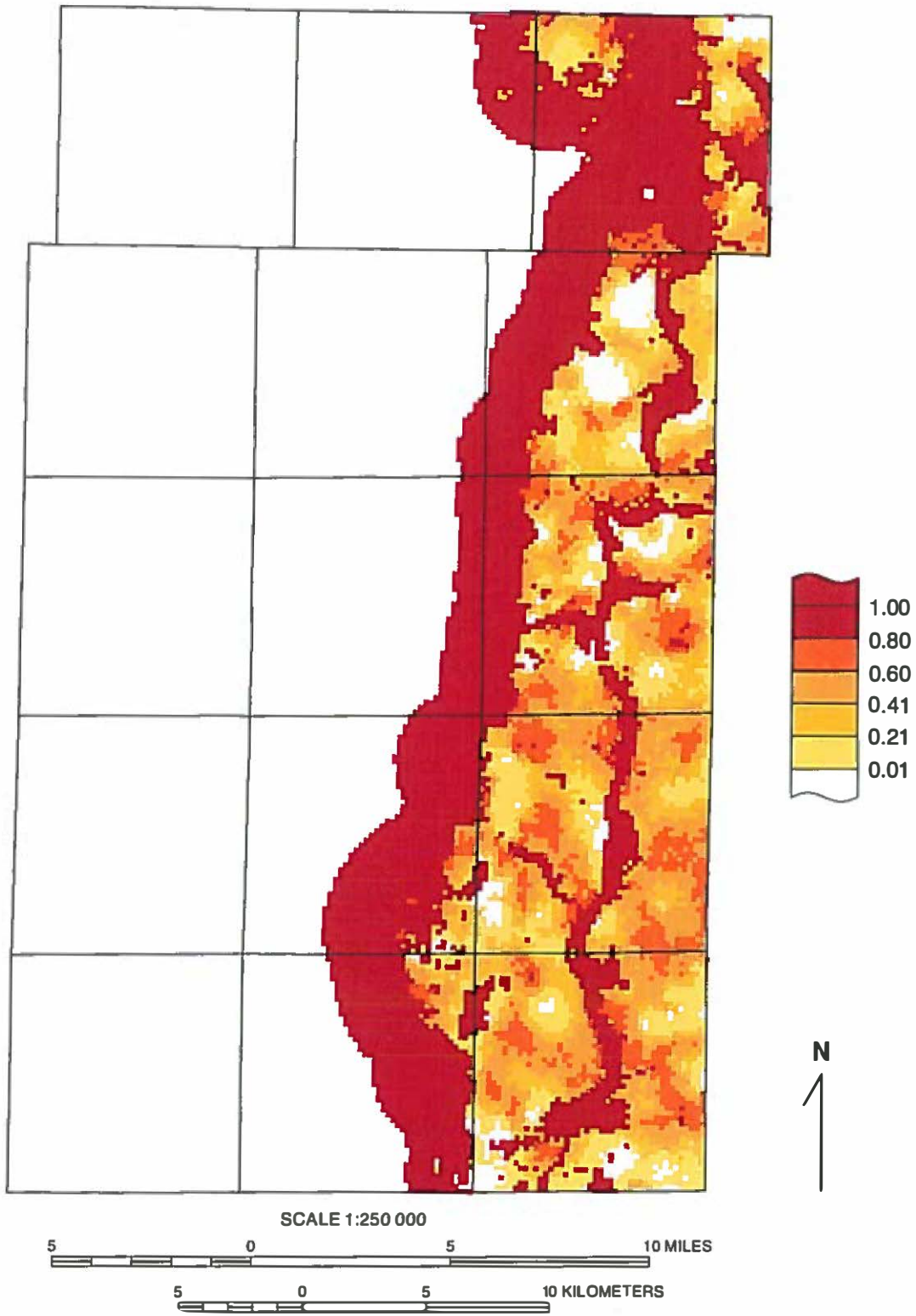
Figure A5 Probability that the sub-Yorkville tongue is less than 1 foot thick.
