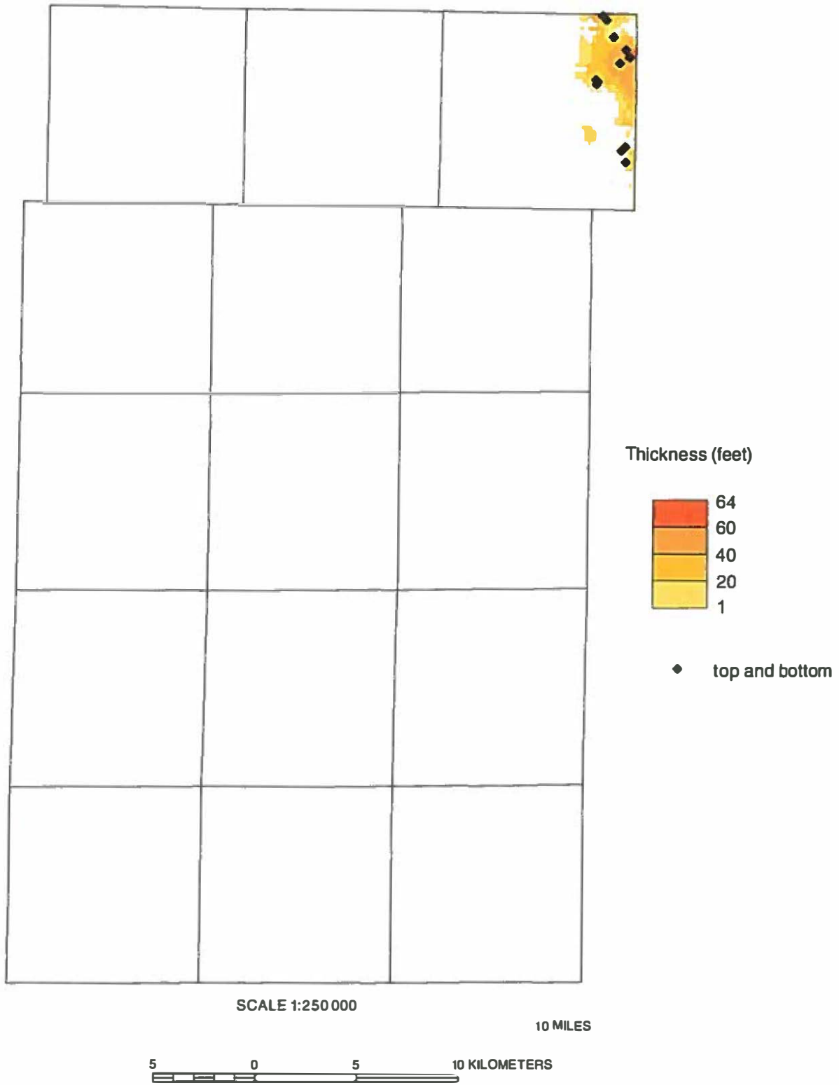
Figure 18 Isopach map of the Beverly Tongue of the Henry Formation and the distribution of primary wells used in mapping the unit.
