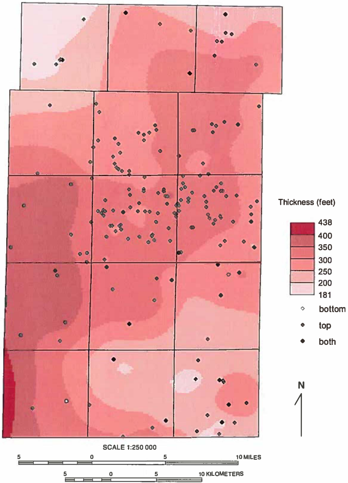
Figure 46 Isopach map of the Ansell Group of the Ordovician System in Kane County and the distribution of primary wells used in mapping the unit.
