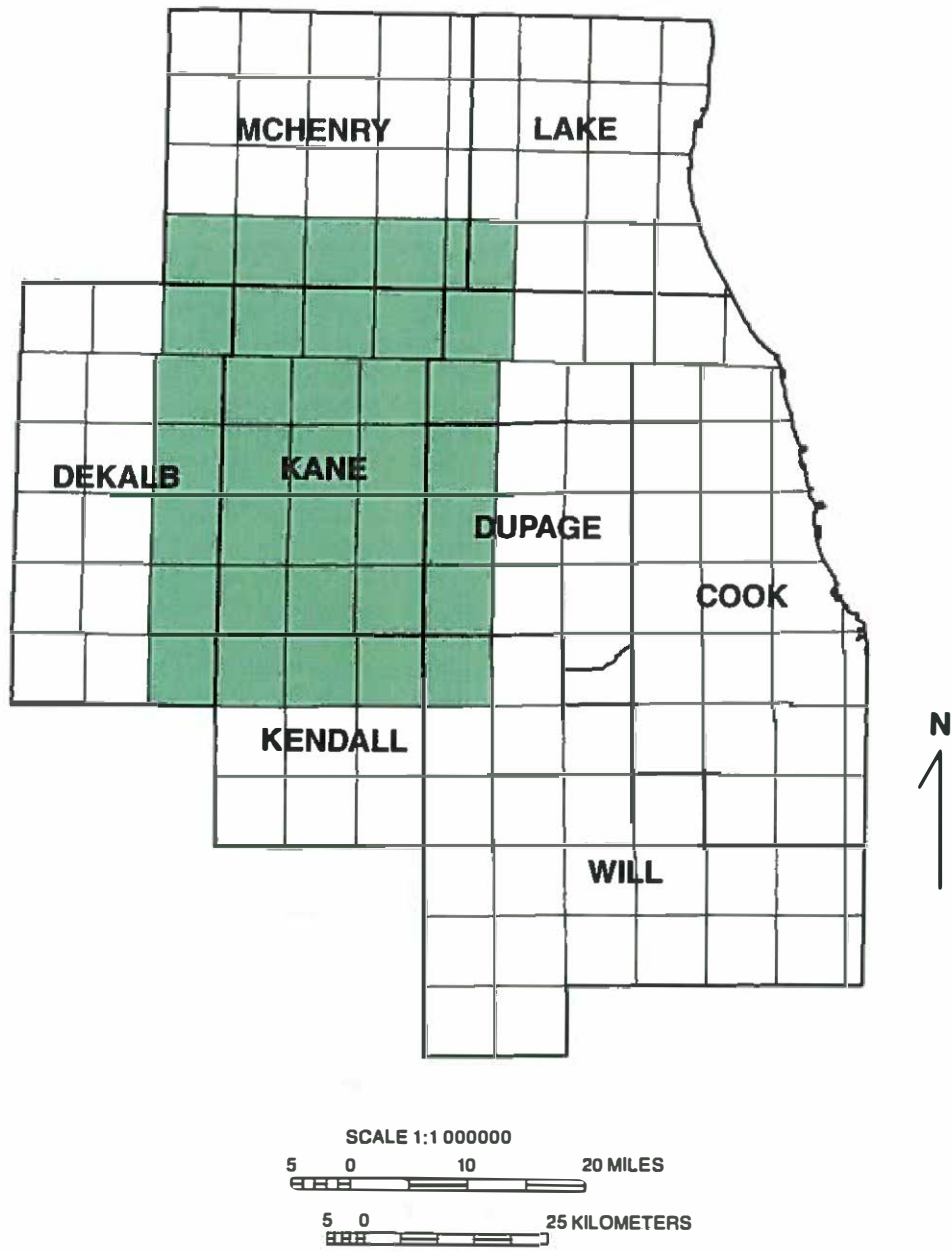
Figure 1 Location of the study area (in green).
