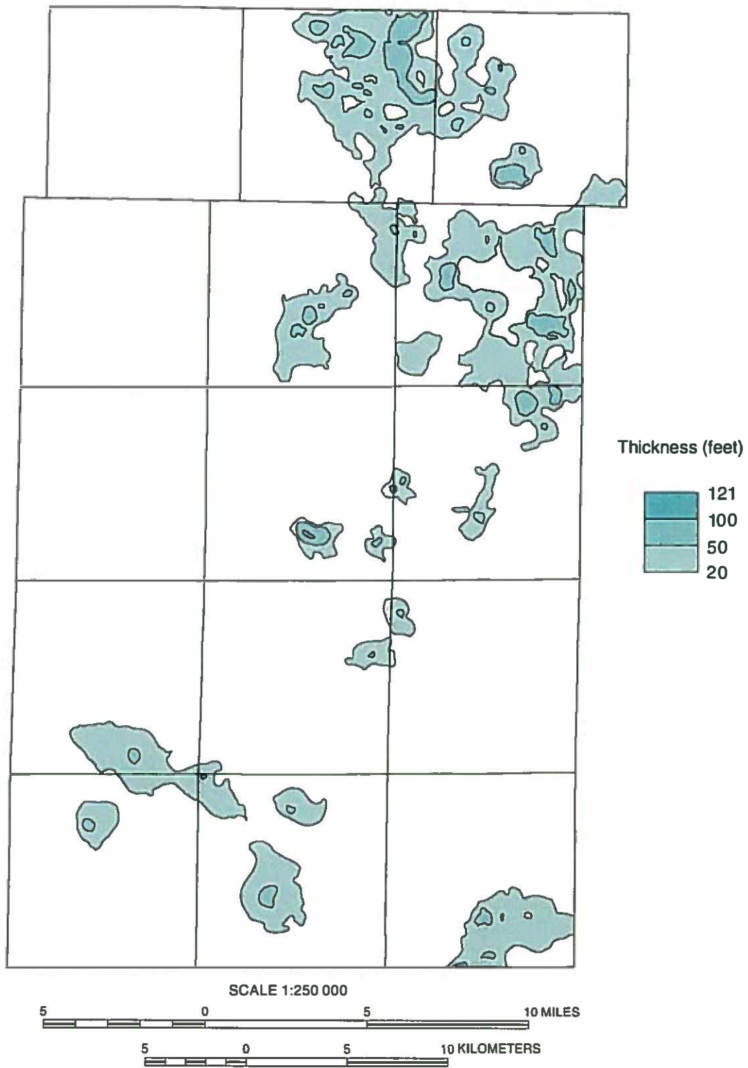
Figure 58 Distribution and thickness of the unnamed aquifers in Kane County.
