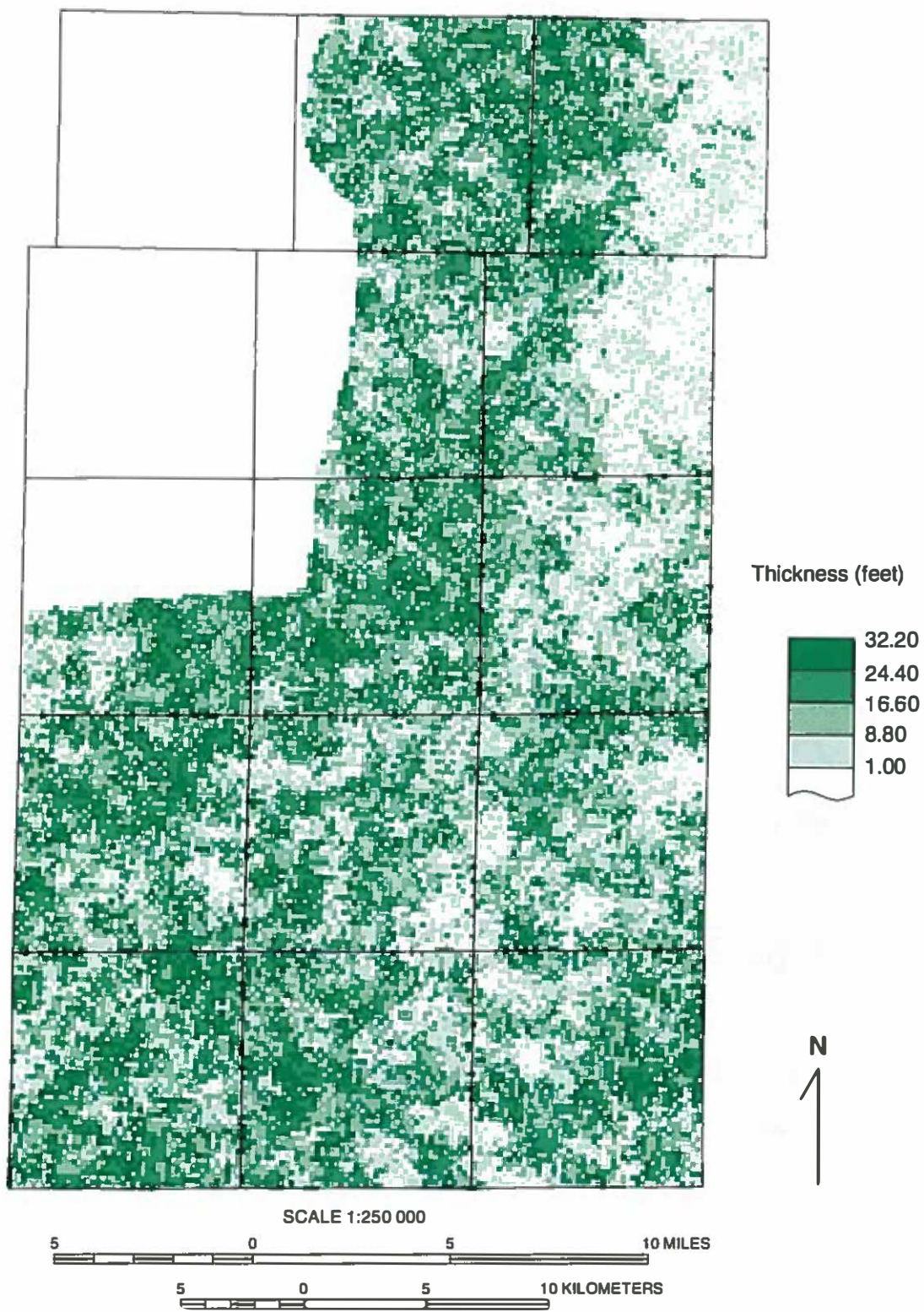
Figure A7 Simulation map of the thickness of the Batestown Member of the Lemont Formation showing large local variability.
