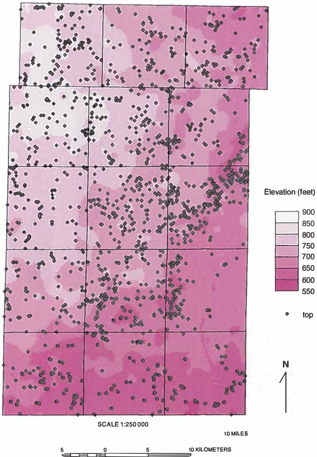
Figure 31 Elevation grid of the upper surface of the Glasford Formation in Kane County and the distribution of primary wells used in mapping the surface.
