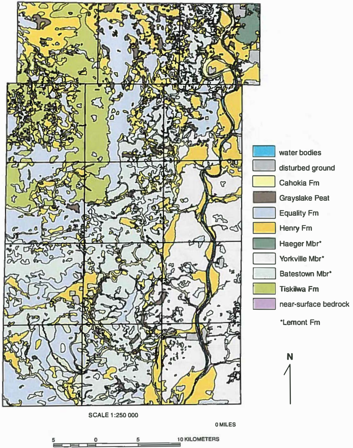
Figure 4 Lithostratigraphic units that are present at the ground surface.
