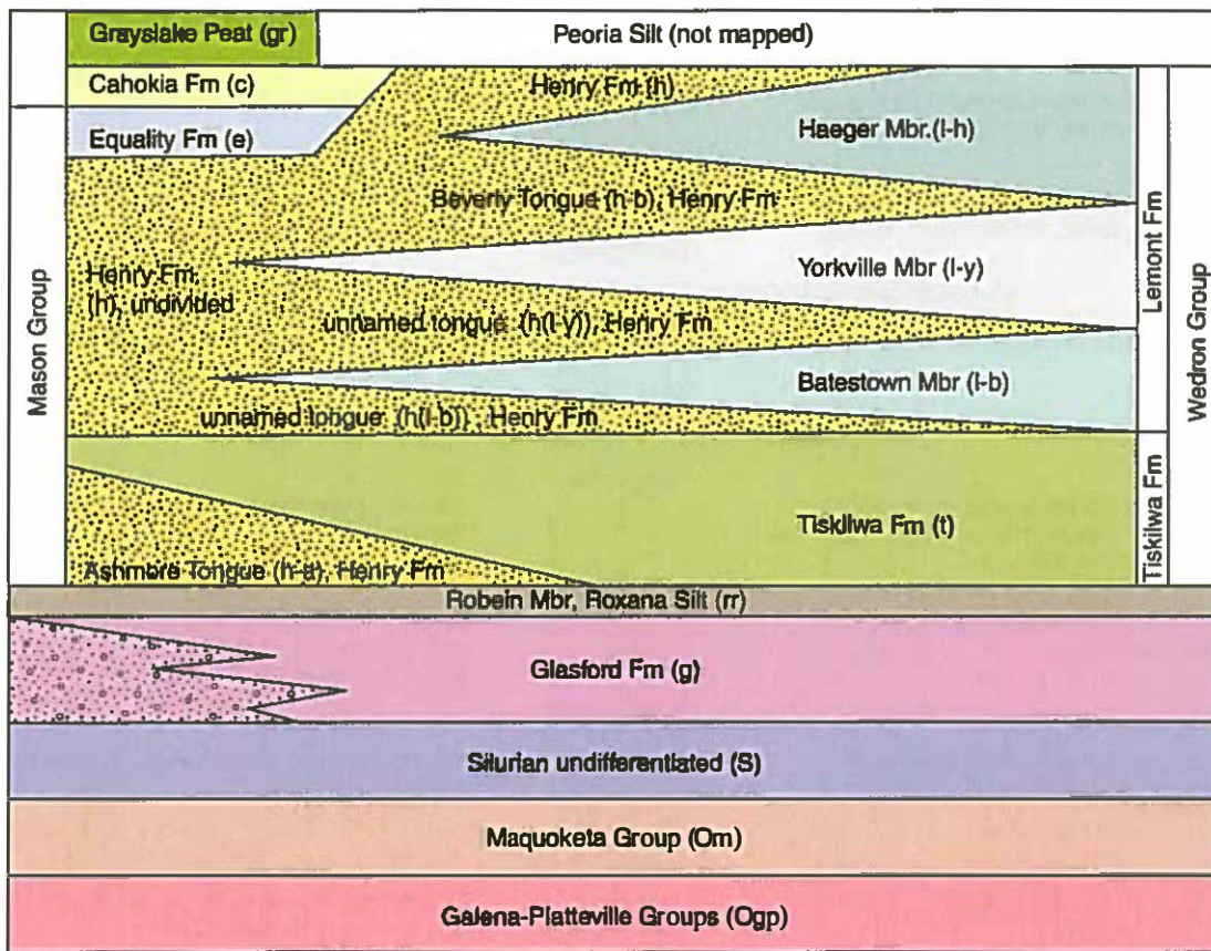
Figure 3 Schematic diagram showing lateral and vertical relationships between Mason Group units and diamictics of the Wedron Group and the vertical sequence of shallow bedrock units below the Glasford Formation (modified from Curry et al. 1999).
