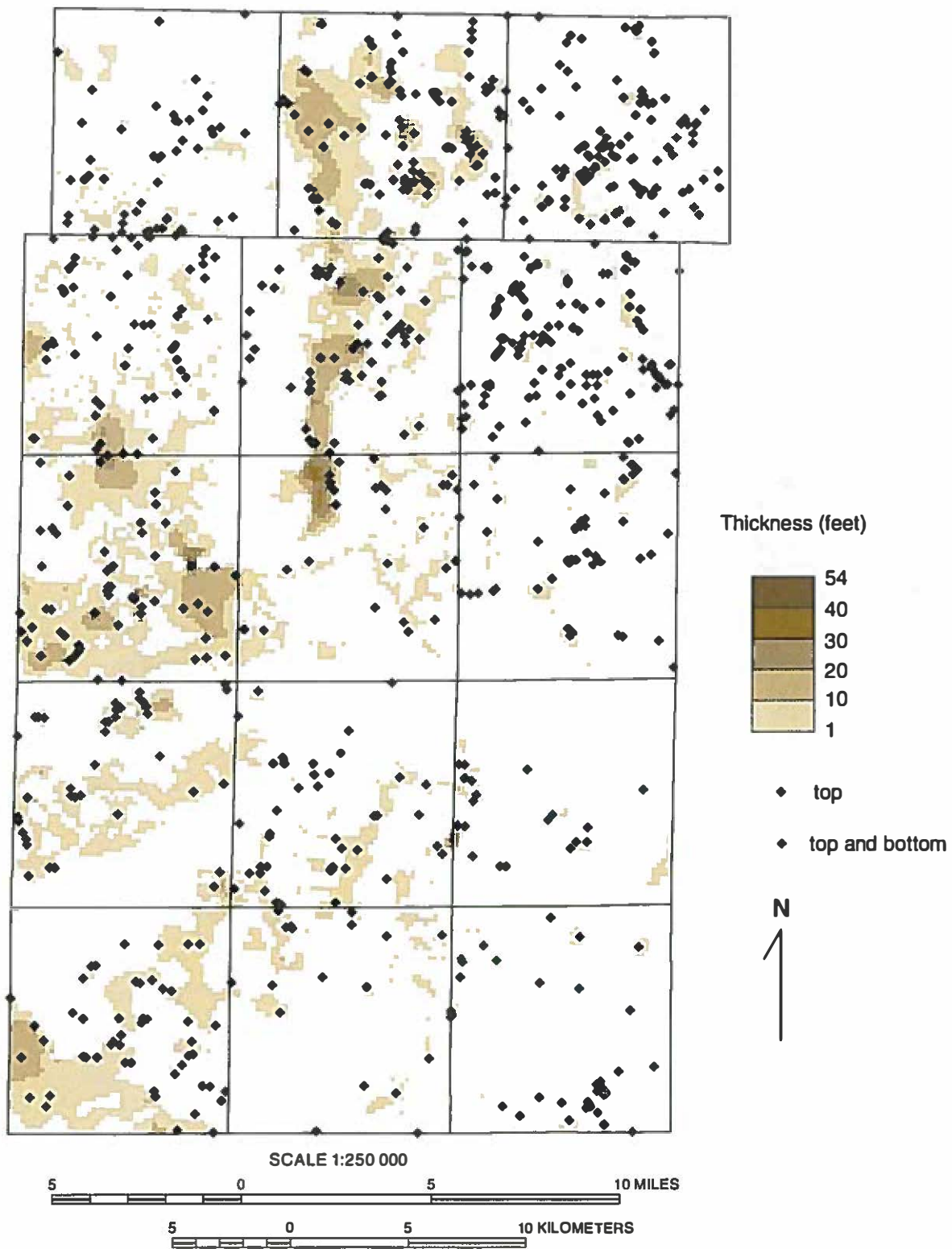
Figure 11 Isopach map of the surficial fine-textured layer (i.e., the combined thickness of the Grayslake Peat, fine-textured facies of the Cahokia Formation, and surficial deposits of the Equality Formation) in Kane County and the distribution of primary wells used in mapping the unit.
