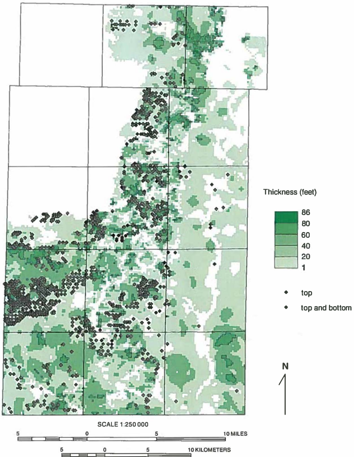
Figure 24 Isopach map of the Batestown Member, Lemont Formation, in Kane County and the distribution of synthetic data points used in mapping the unit.
