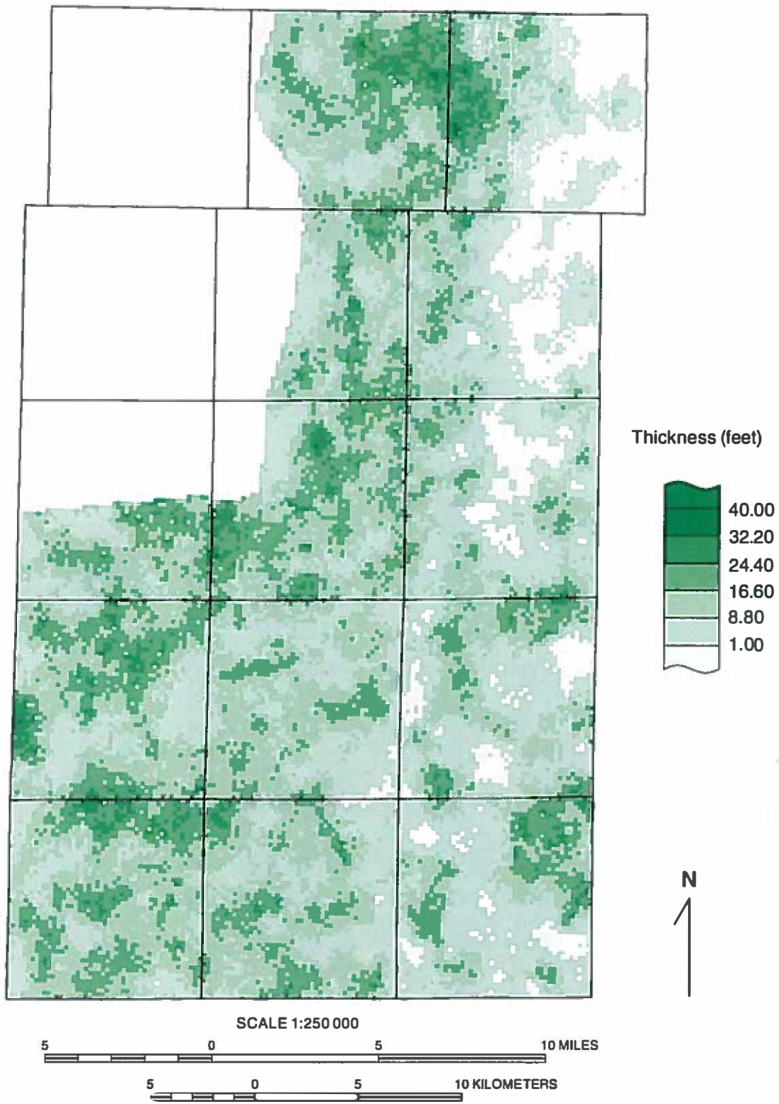
Figure A6 Simulation map of the thickness of the Batestown Member of the Lemont Formation showing small local variability.
