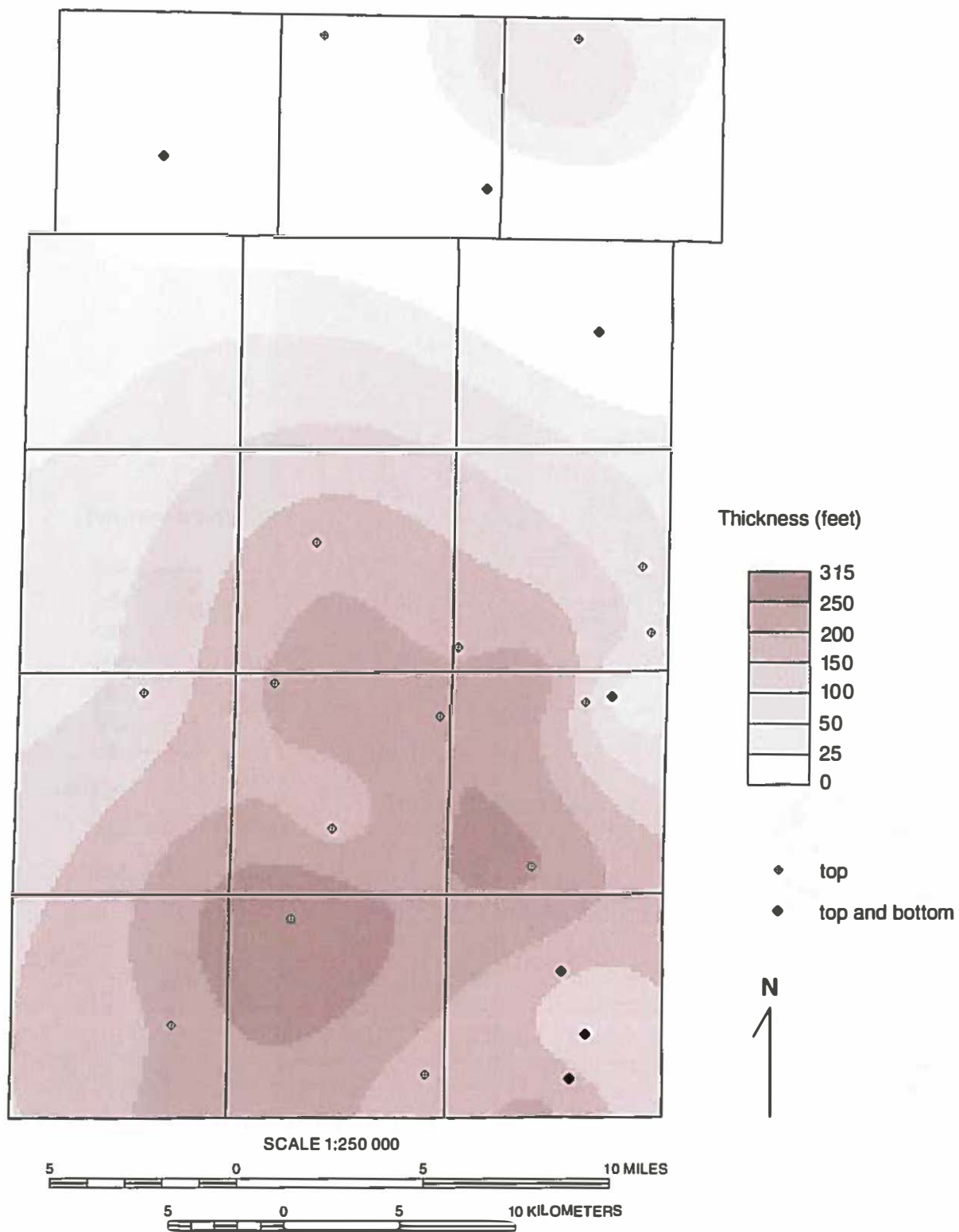
Figure 47 Isopach map of the Prairie du Chien Group of the Ordovician System in Kane County and the distribution of primary wells used in mapping the unit.
