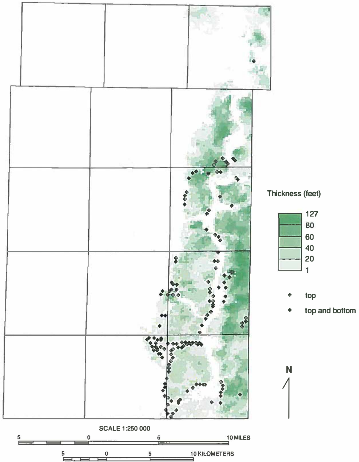
Figure 21 Isopach map of the Yorkville Member, Lemont Formation, in Kane County and the distribution of synthetic data points used in mapping the unit.
