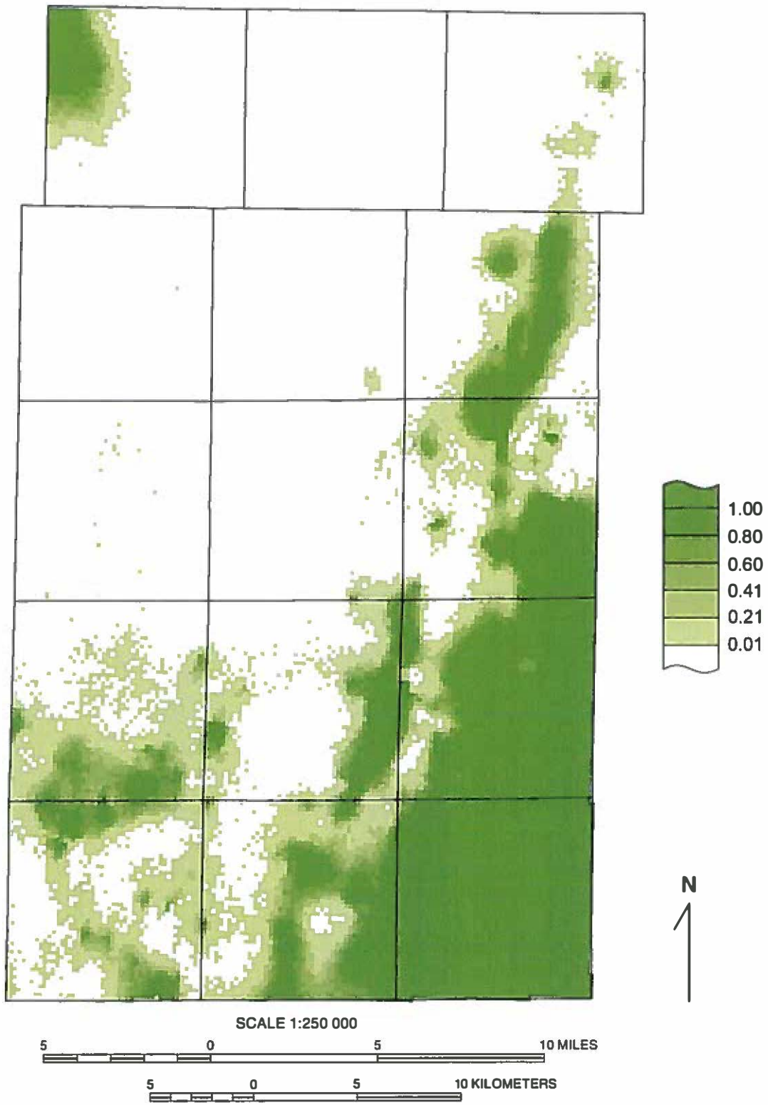
Figure A15 Probability that the Tiskilwa Formation diamicton is less than 1 foot thick. This map is based on step-one simulation results.
