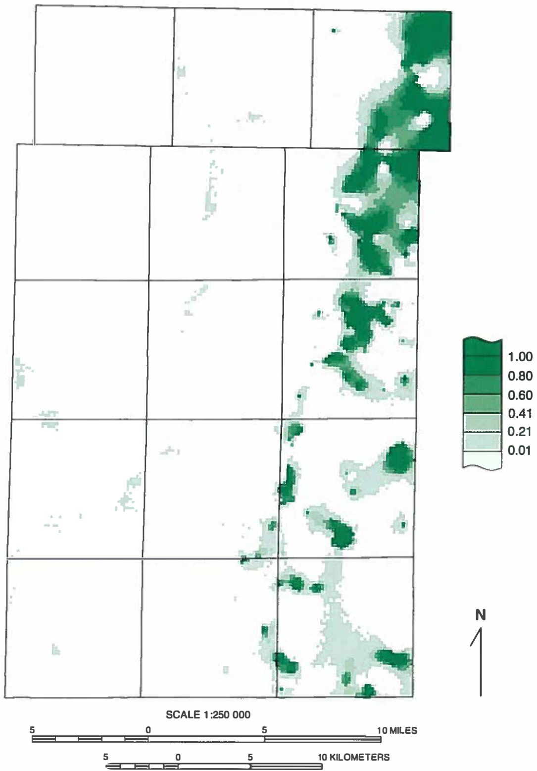
Figure A10 Probability that the Batestown Member diamicton is less than 1 foot thick.
