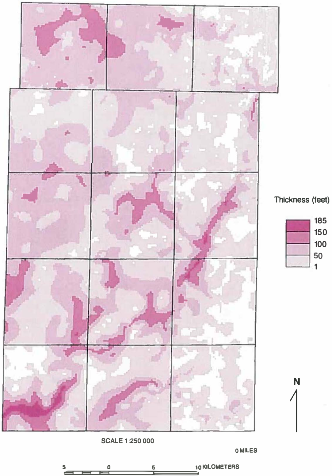
Figure 33 Isopach map of the Glasford Formation in Kane County.
