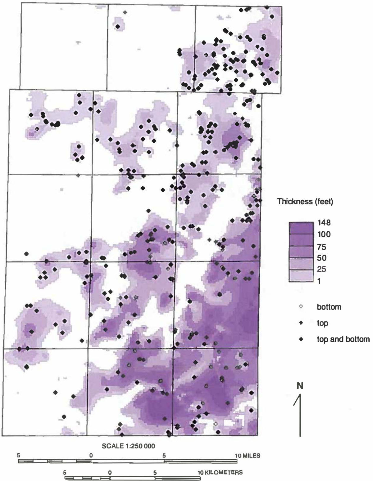
Figure 42 Isopach map of the Silurian System in Kane County and the distribution of primary wells used in mapping the unit.
