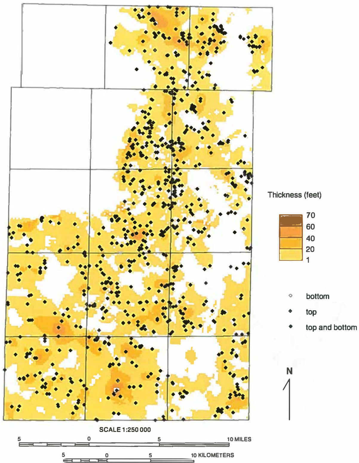
Figure 25 Isopach map of the sub-Batestown tongue of the Henry Formation in Kane County and the distribution of primary wells used in mapping the unit.
