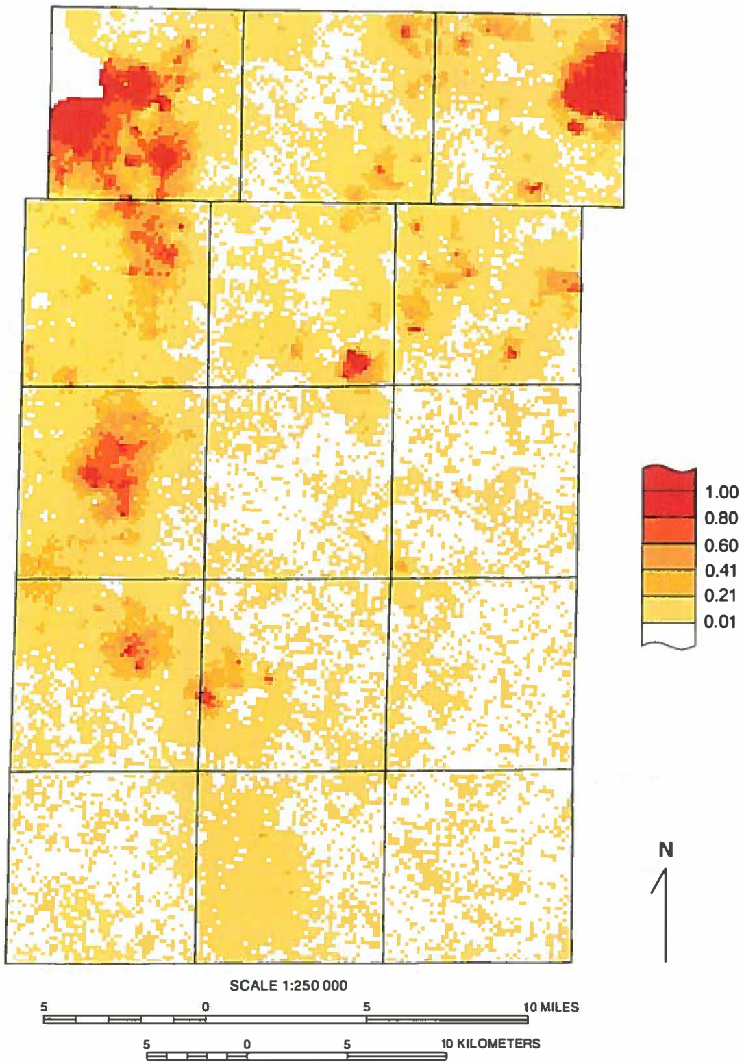
Figure A19 Probability that the Ashmore Tongue is greater than 20 feet thick. This map was based on the Step 2 simulation results.
