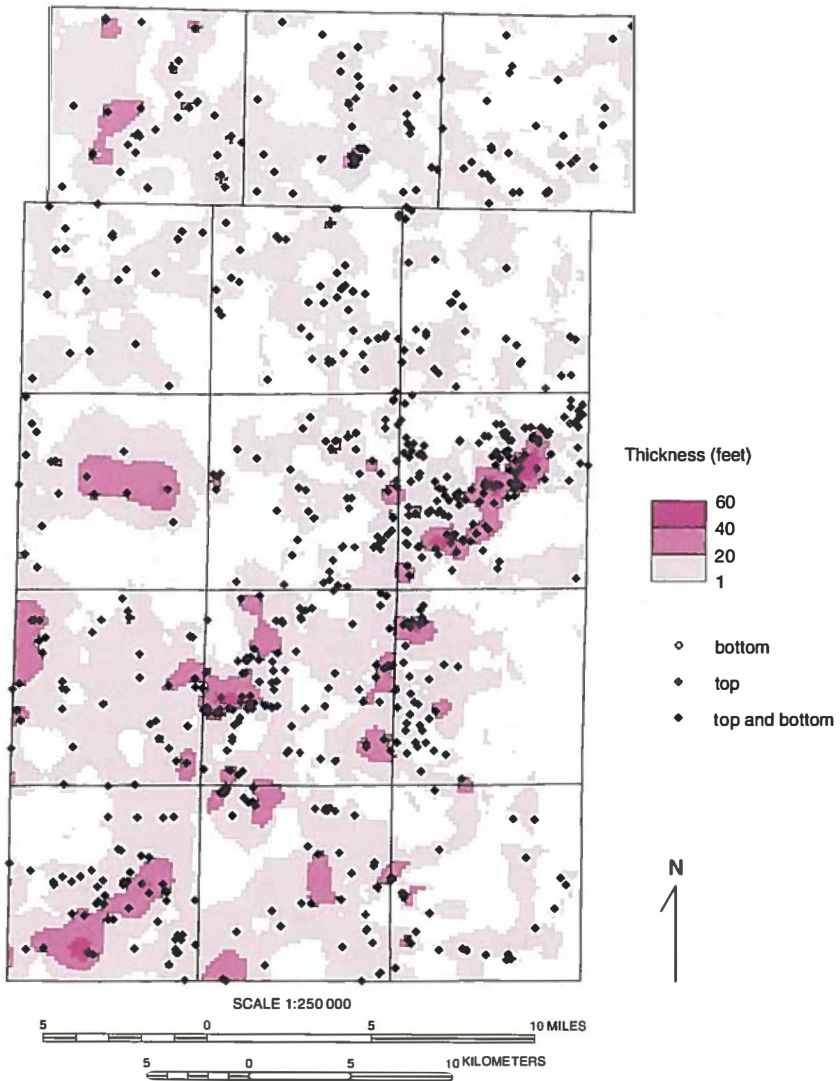
Figure 35 Isopach map of the upper coarse-textured unit of the Glasford Formation in Kane County and the distribution of primary wells used in mapping the unit.
