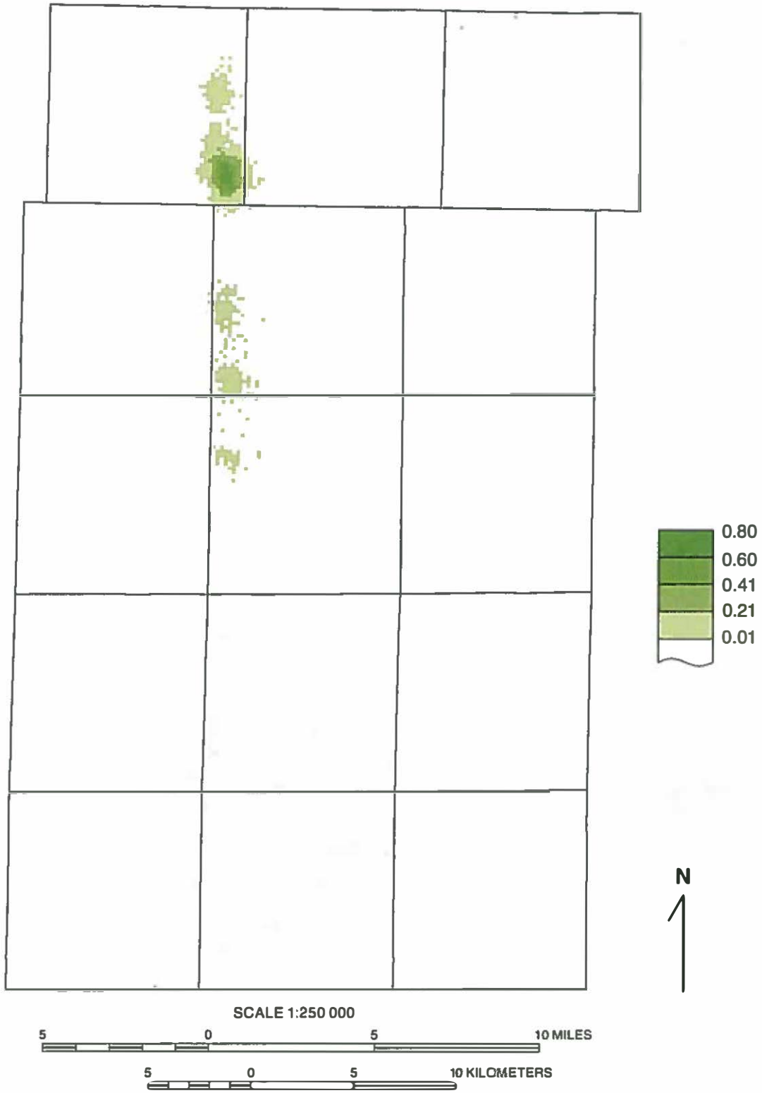
Figure A14 Probability that the Tiskilwa Formation diamicton is greater than 250 feet thick. This map is based on step-one simulation results.
