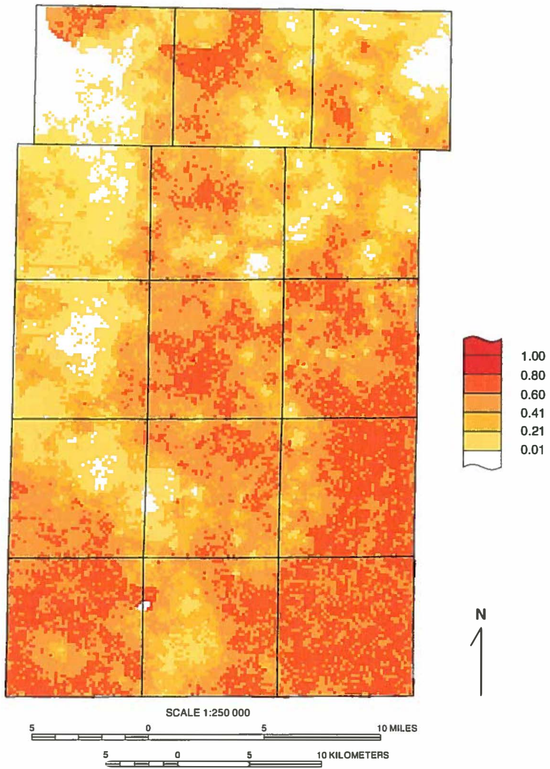
Figure A20 Probability that the Ashmore Tongue is less than 1 foot thick. This map was based on the Step 2 simulation results.
