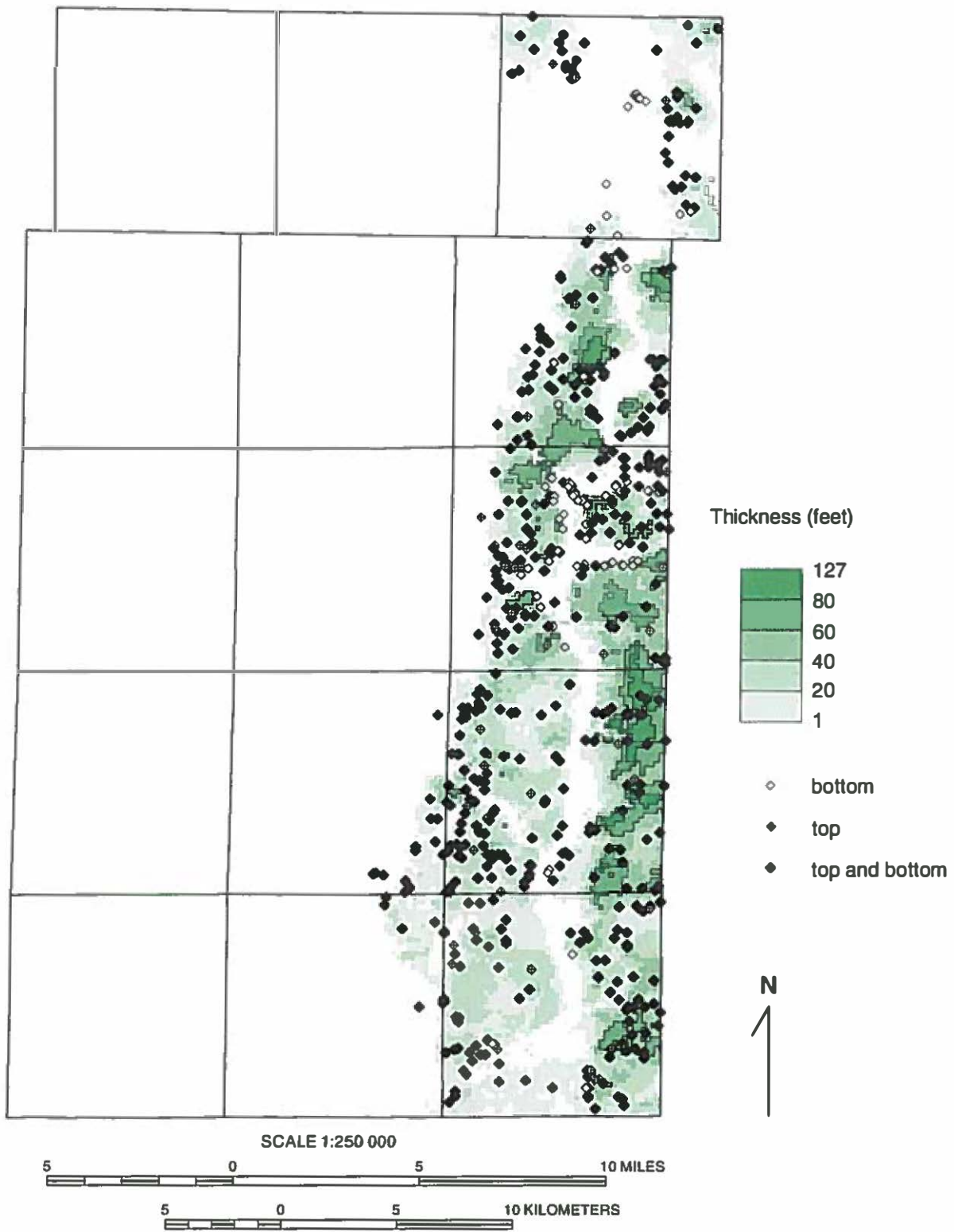
Figure 20 Isopach map of the Yorkville Member, Lemont Formation, in Kane County and the distribution of primary wells used in mapping the unit.
