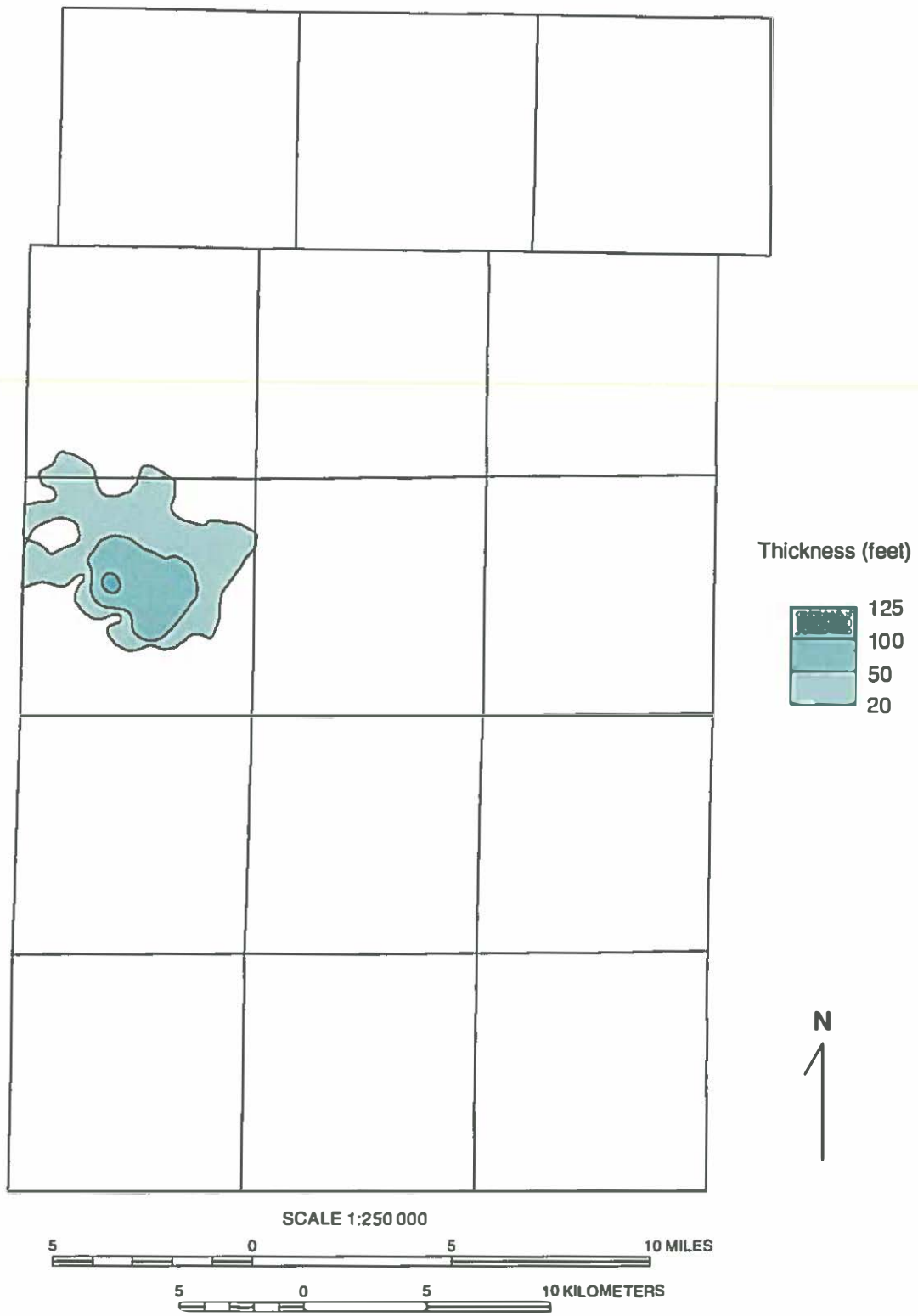
Figure 55 Distribution and thickness of the Virgil aquifer in Kane County.
