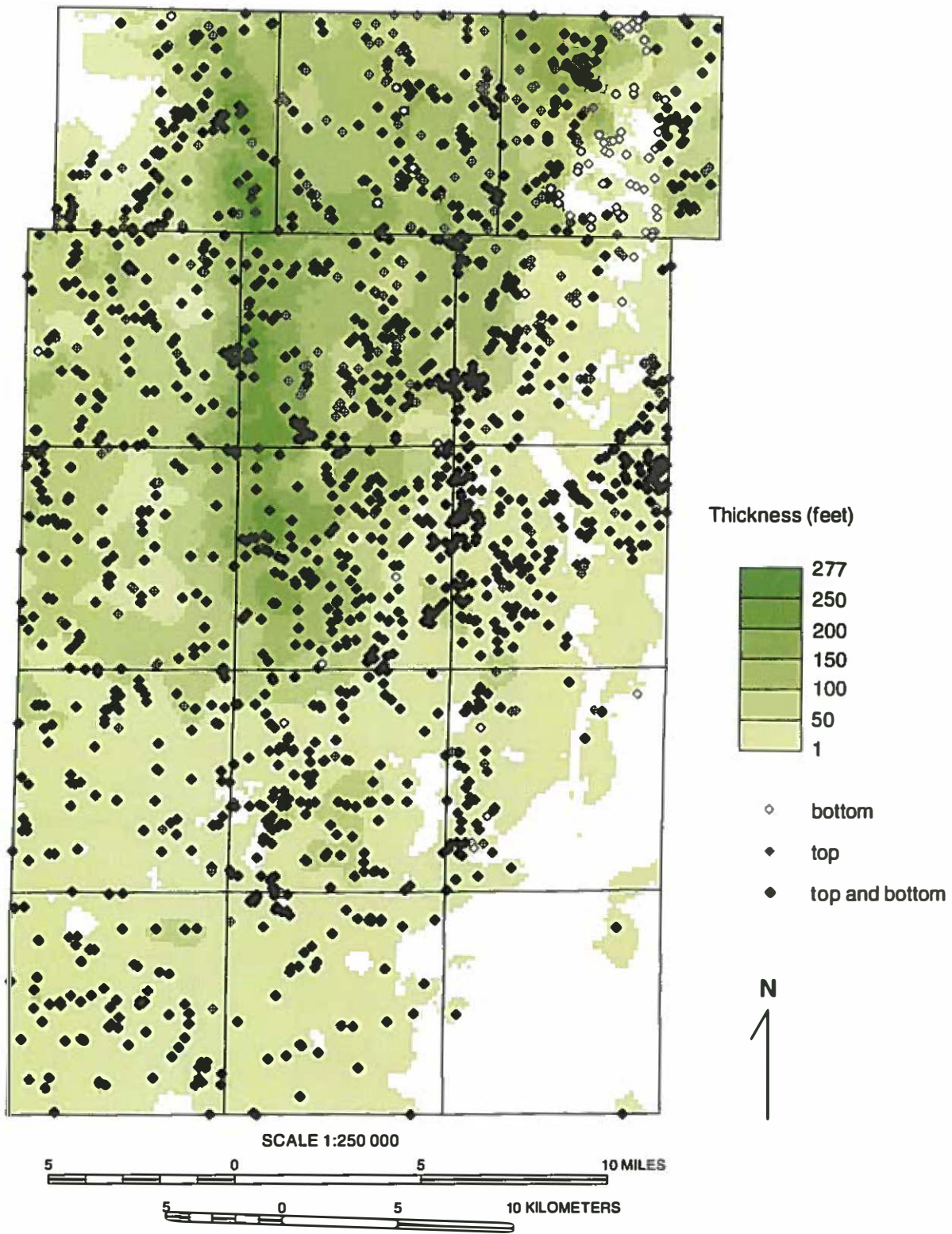
Figure 27 Isopach map of the Tiskilwa Formation in Kane County and the distribution of primary wells used in mapping the unit.
