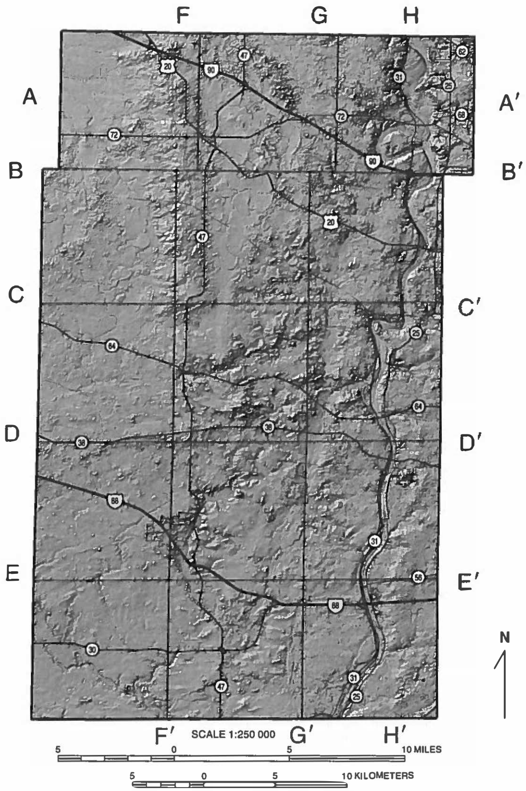
Figure 49 Location of geologic cross section lines in Kane County. Cross sections are shown on pp. 110-111.
