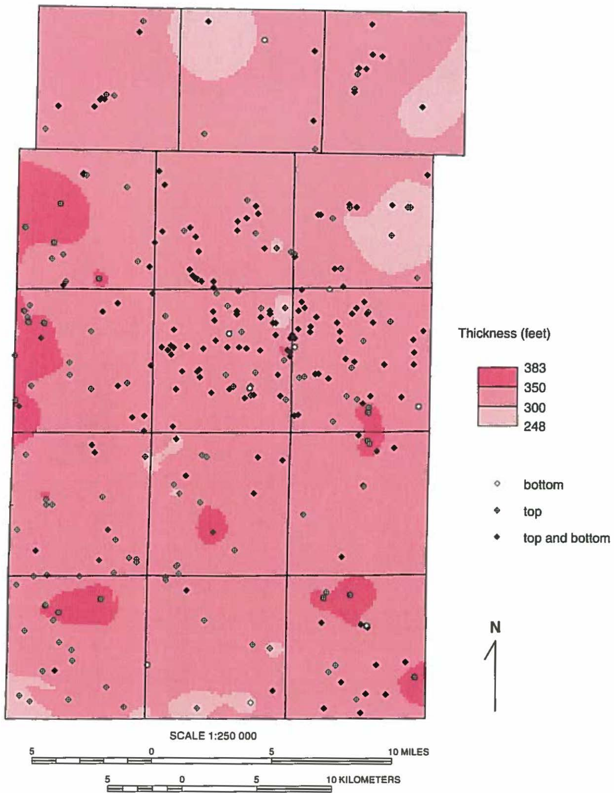
Figure 45 Isopach map of the Galena and Platteville Groups of the Ordovician System in Kane County and the distribution of primary wells used in mapping the unit.
