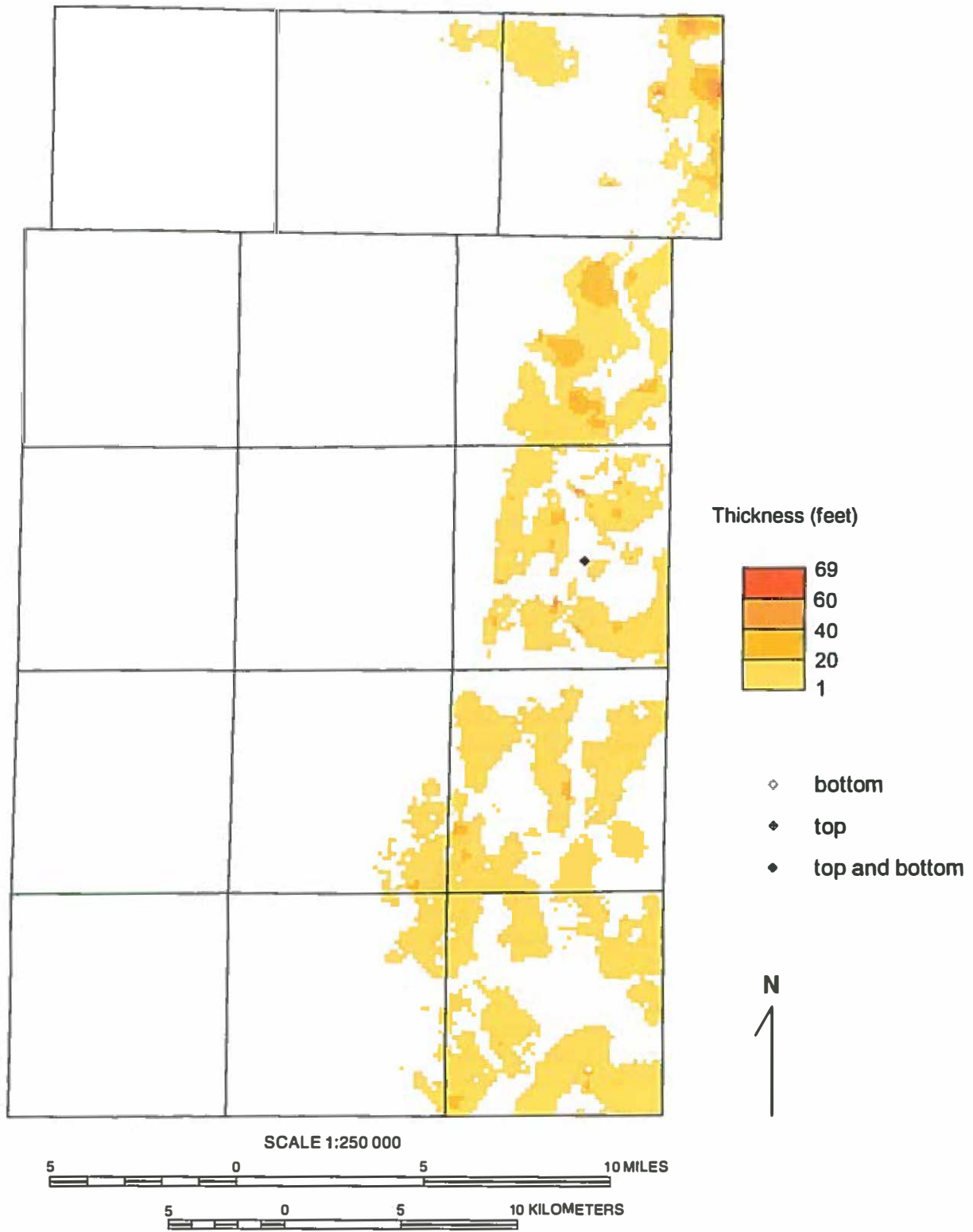
Figure 23 Isopach map of the sub-Yorkville tongue of the Henry Formation in Kane County and the distribution of synthetic data points used in mapping the unit.
