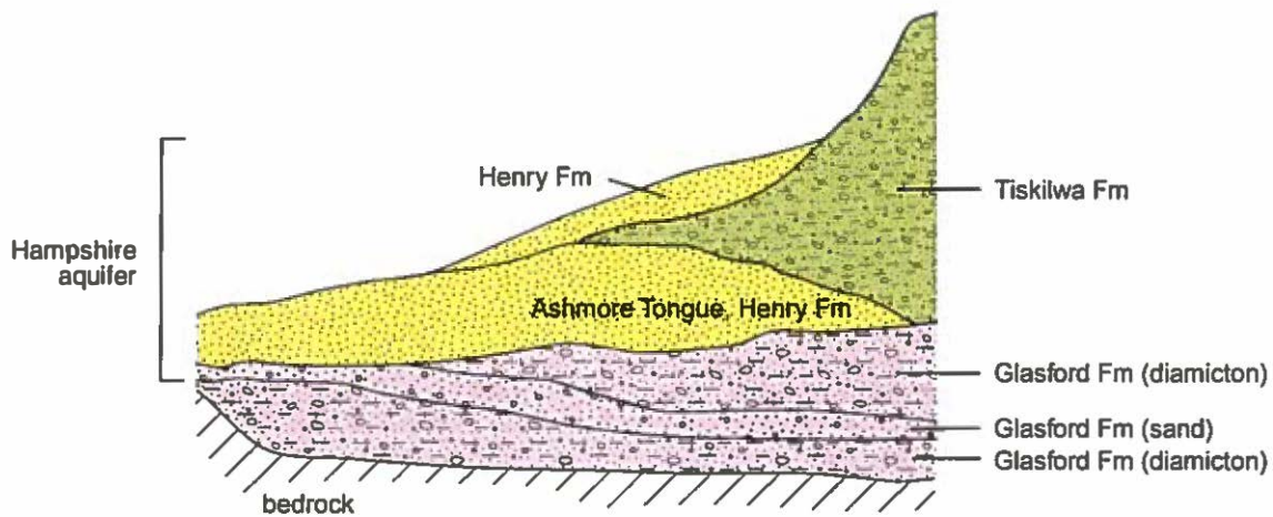
Figure 51 Schematic diagram of the Hampshire aquifer.
