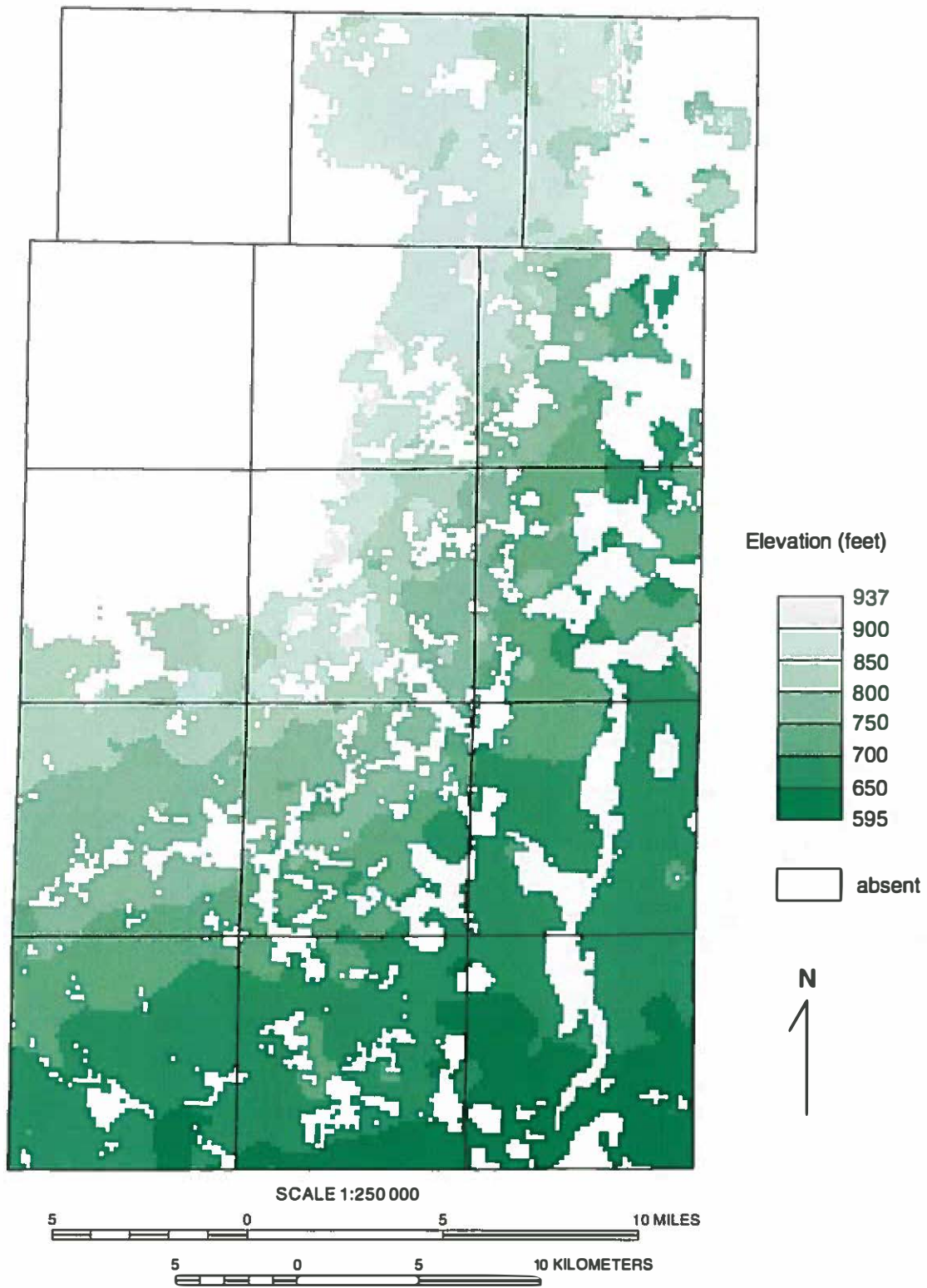
Figure 9 Elevation grid of the lower surface of the Batestown Member, Lemont Formation, in Kane County.
