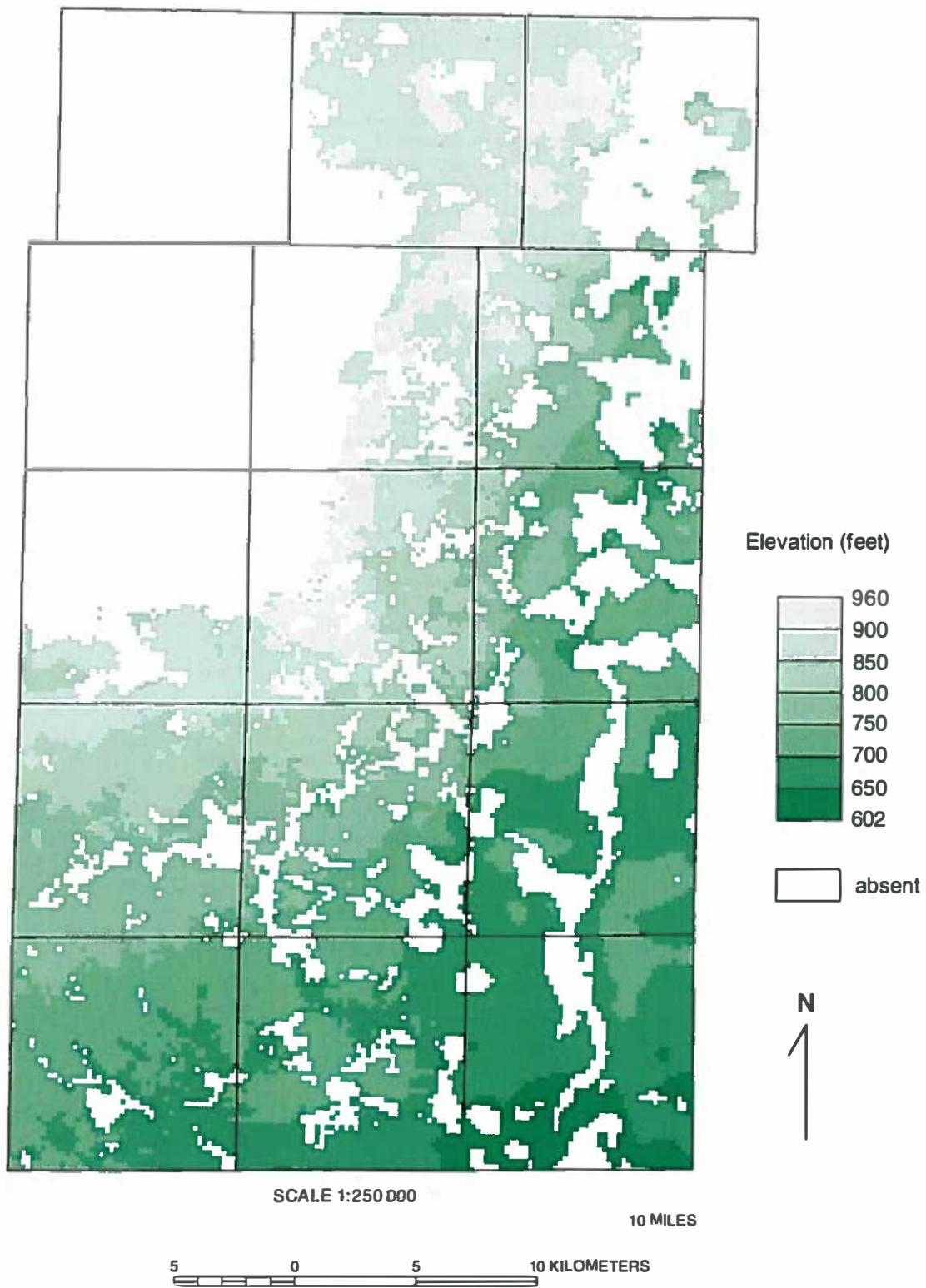
Figure 8 Elevation grid of the upper surface of the Batestown Member, Lemont Formation, in Kane County.
