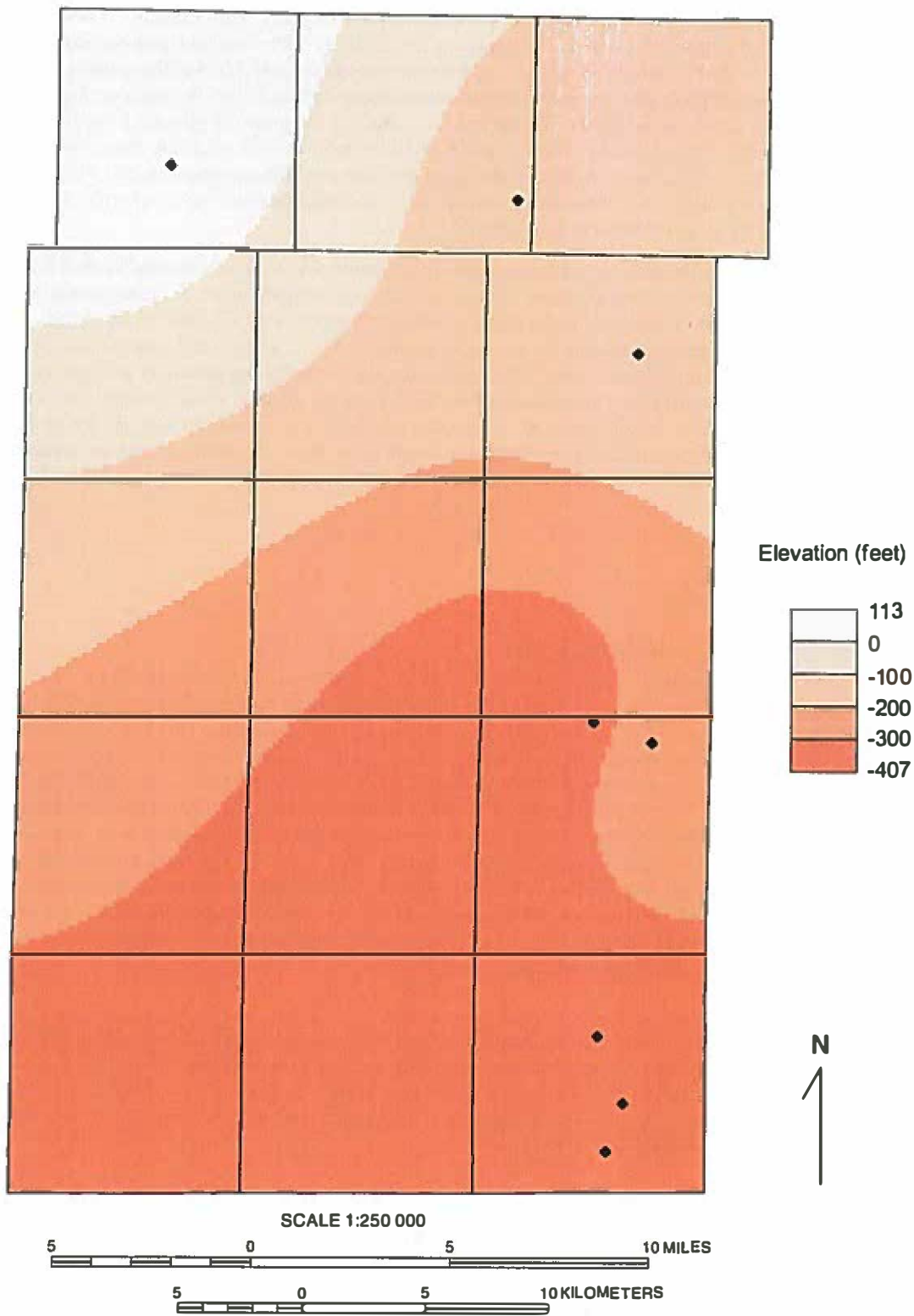
Figure 48 Elevation of the upper surface of the Cambrian System in Kane County and the distribution of primary wells used in mapping the surface.
