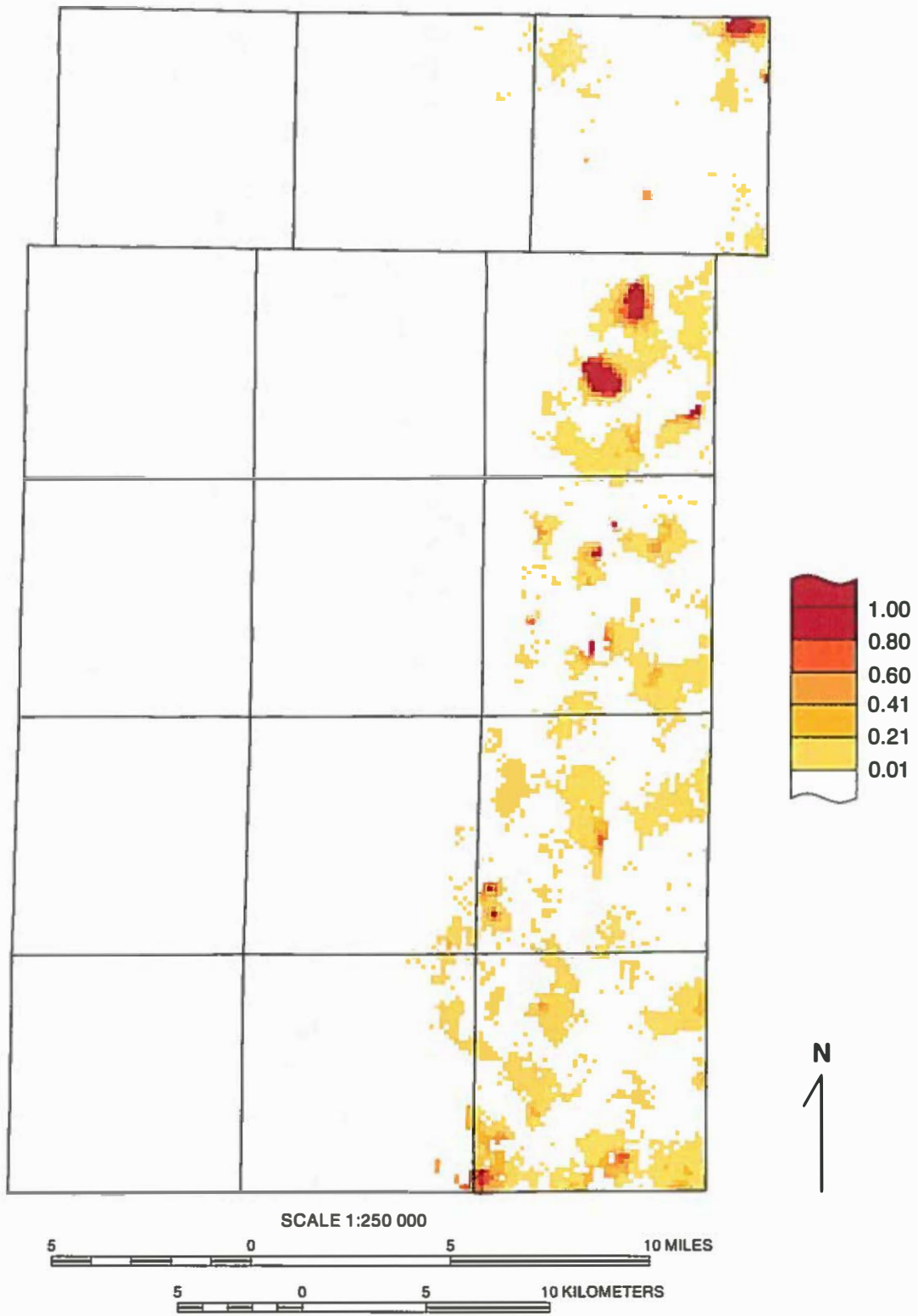
Figure A4 Probability that the sub-Yorkville tongue is greater than 20 feet thick.
