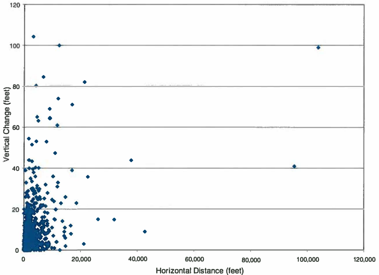
Figure 7 Horizontal and vertical adjustments to wells assigned new location coordinates through field verification.
