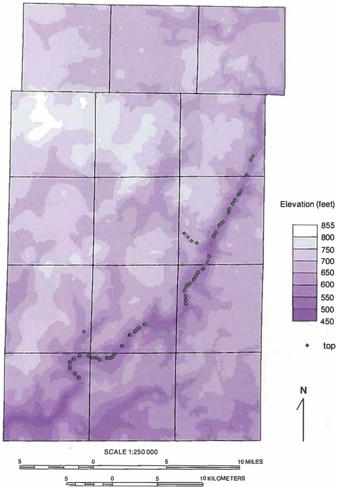
Figure 40 Bedrock topography of Kane County and the distribution of synthetic data points used in mapping the surface.
