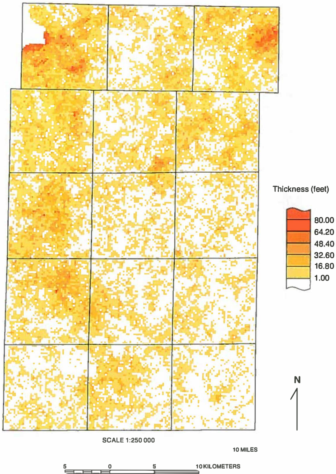
Figure A17 Thickness of the the Ashmore Tongue of the Henry Formation showing large local variability. This map is the 50th percentile map when Step 2 results are sorted on total thickness.
