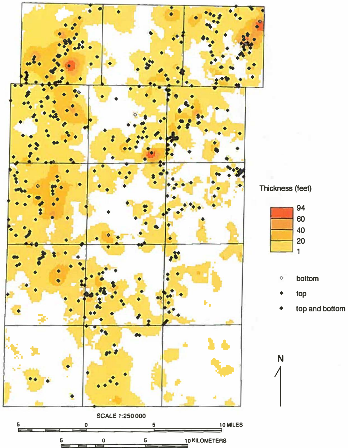
Figure 29 Isopach map of the Ashmore Tongue of the Henry Formation in Kane County and the distribution of primary wells used in mapping the unit.
