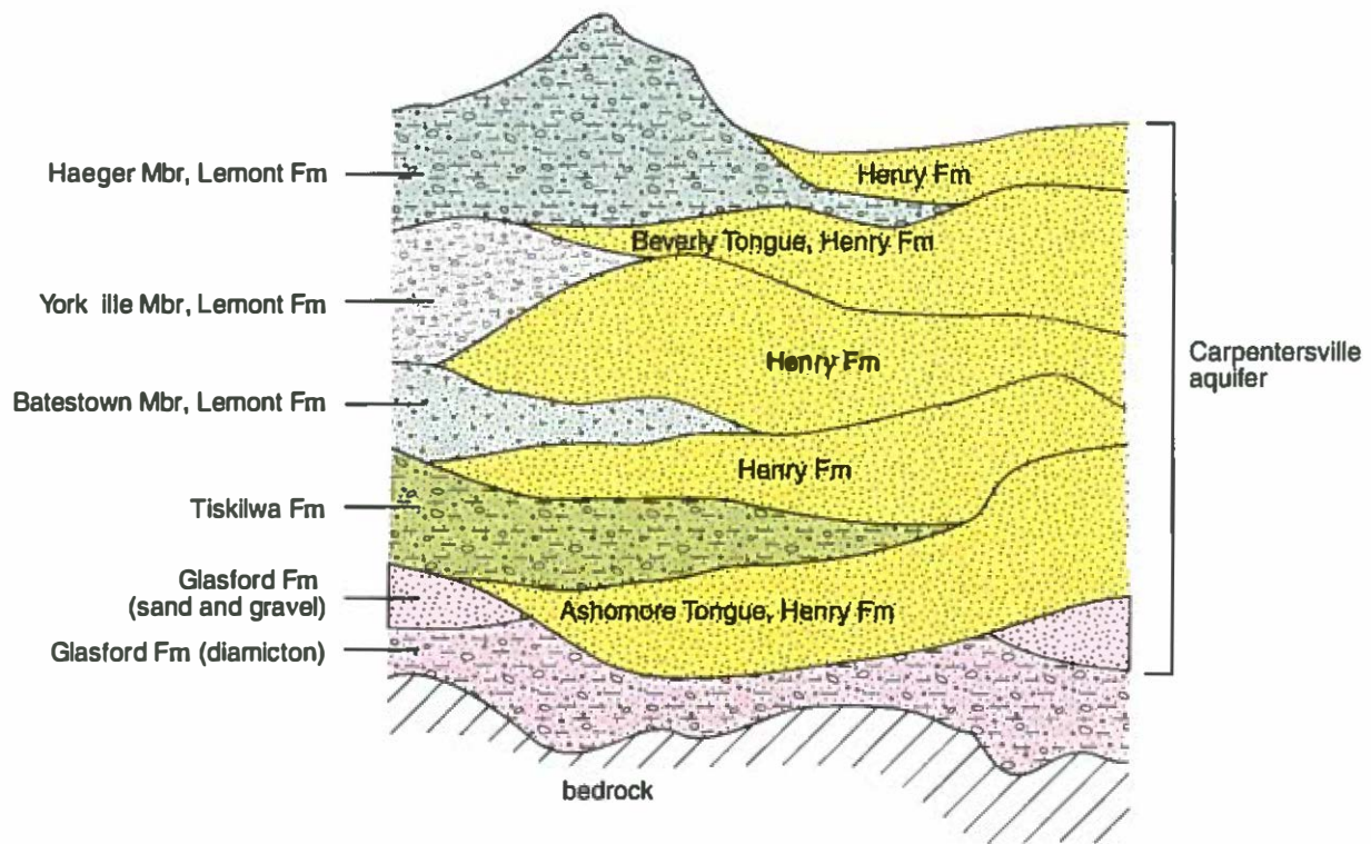
Figure 52 Schematic diagram of the Carpentersville aquifer.
