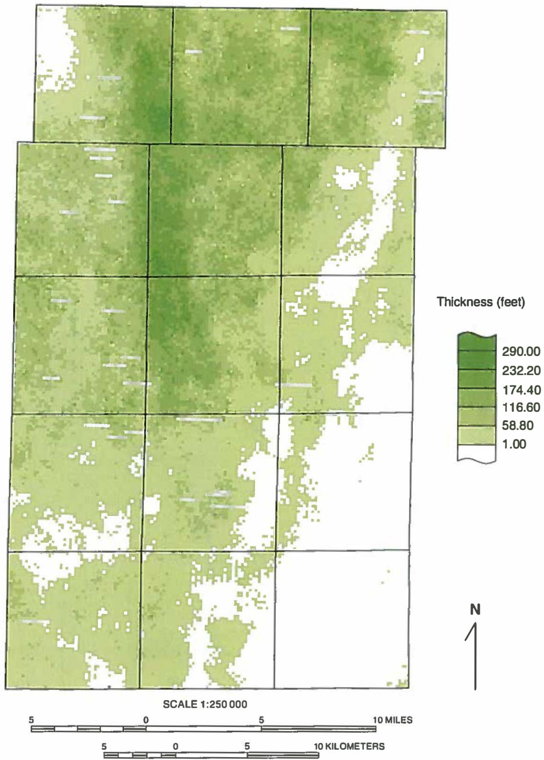
Figure A11 Simulation map of the thickness of the Tiskilwa Formation diamicton showing small local variability.
