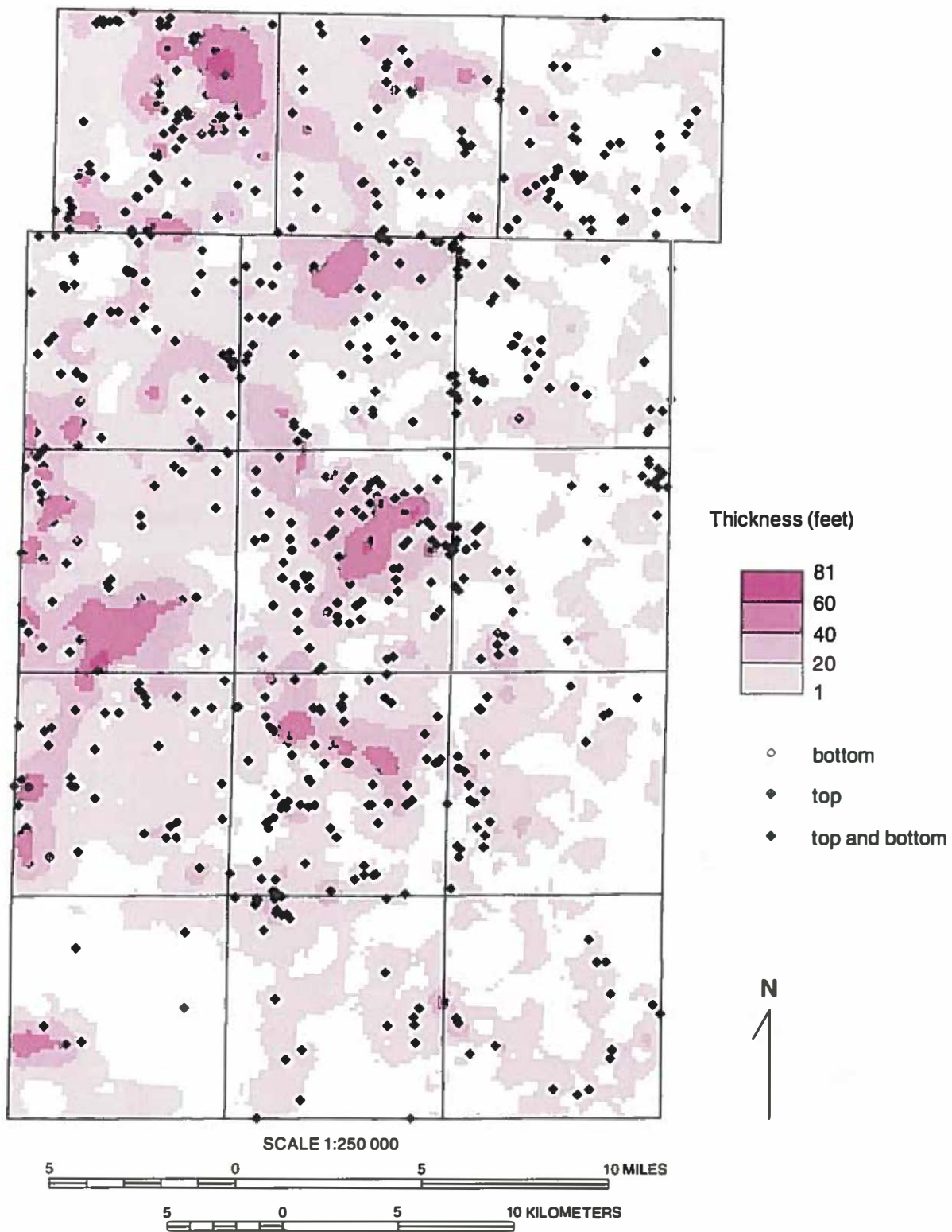
Figure 34 Isopach map of the upper fine-textured unit of the Glasford Formation in Kane County and the distribution of primary wells used in mapping the unit.
