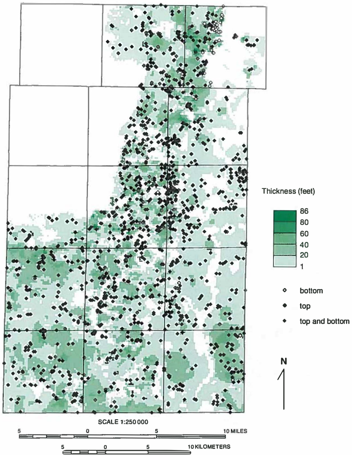
Figure 10 Isopach map of the Batestown Member, Lemont Formation, in Kane County and the distribution of primary wells used in mapping the unit.
