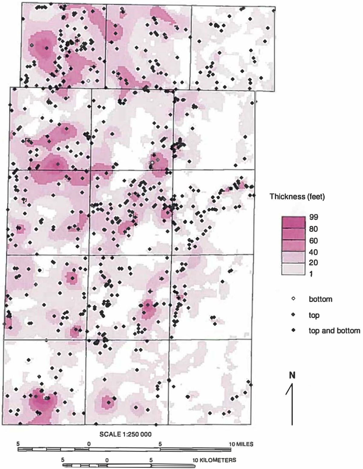
Figure 36 Isopach map of the middle fine-textured unit of the Glasford Formation in Kane County and the distribution of primary wells used in mapping the unit.
