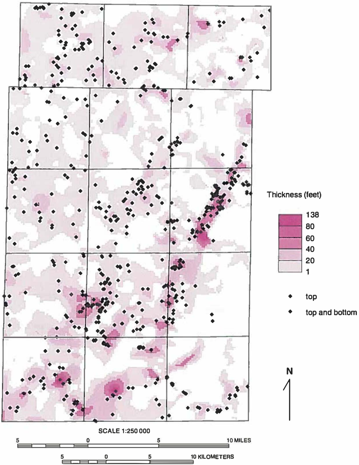
Figure 37 Isopach map of the lower coarse-textured unit of the Glasford Formation in Kane County and the distribution of primary wells used in mapping the unit.
