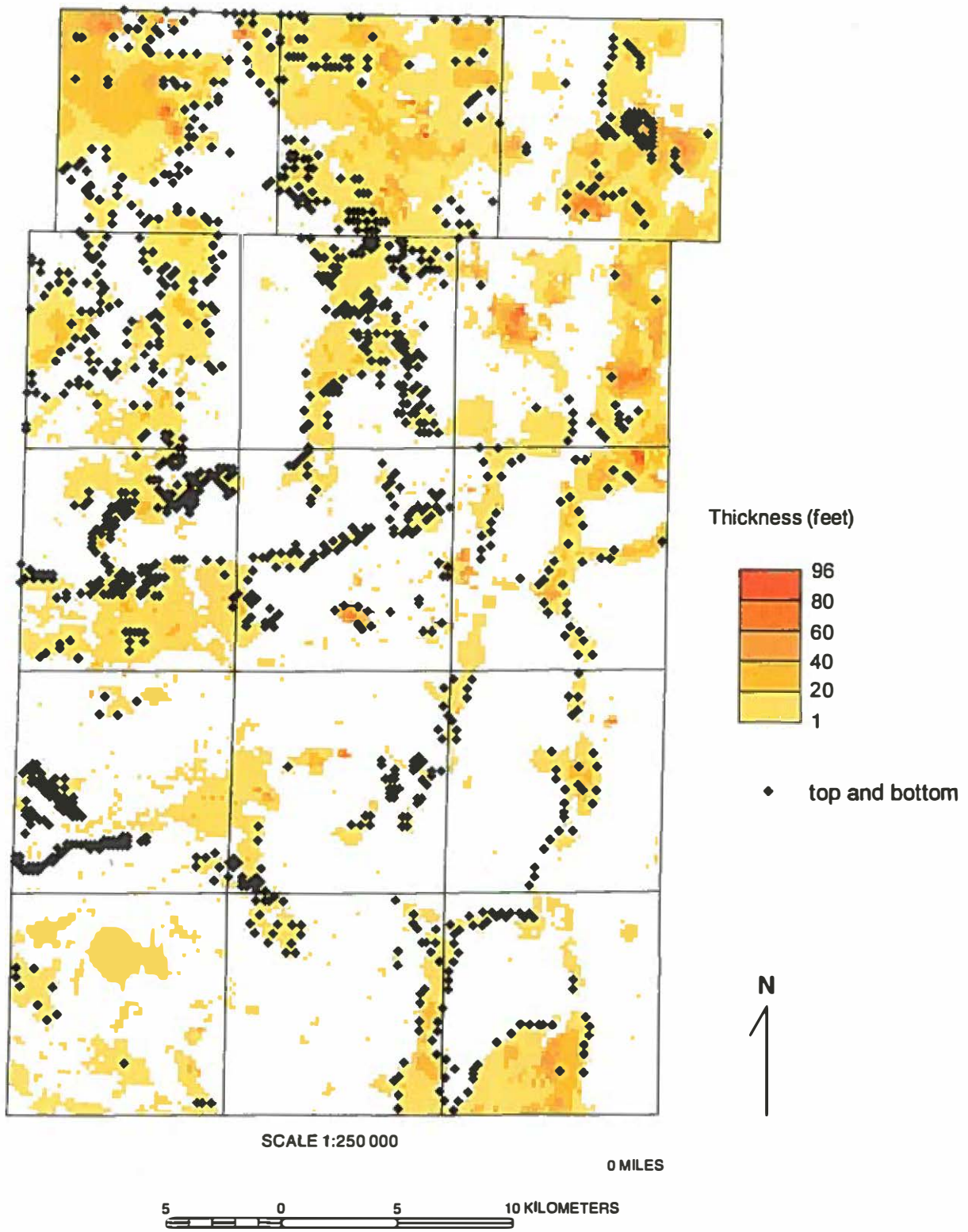
Figure 14 Isopach map of the surficial Henry Formation in Kane County and the distribution of synthetic data points used in mapping the unit.
