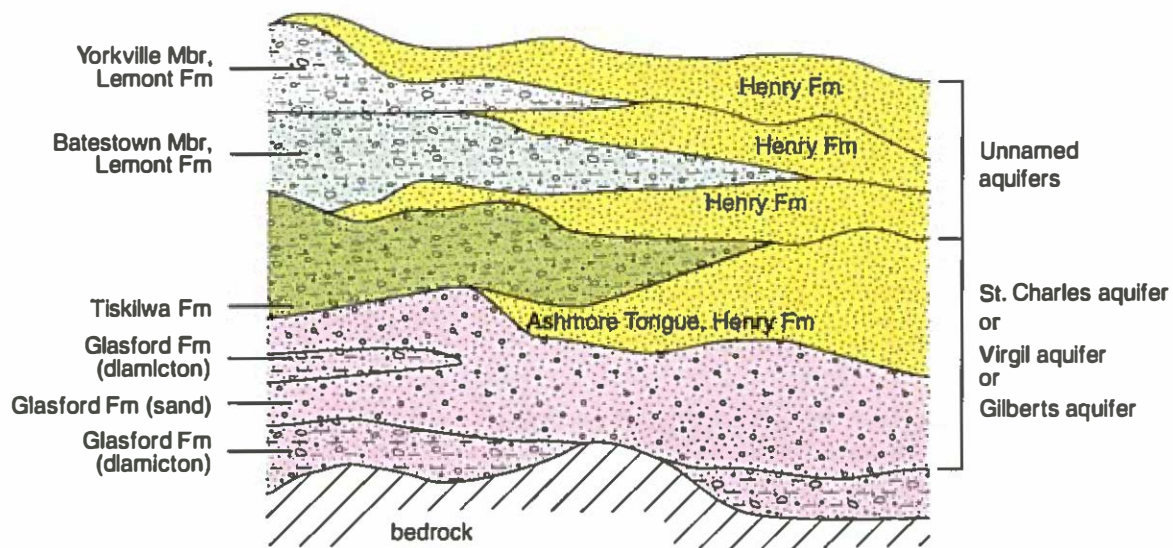
Figure 50 Schematic diagram of the St. Charles, Virgil, Gilberts, and unnamed aquifers.
