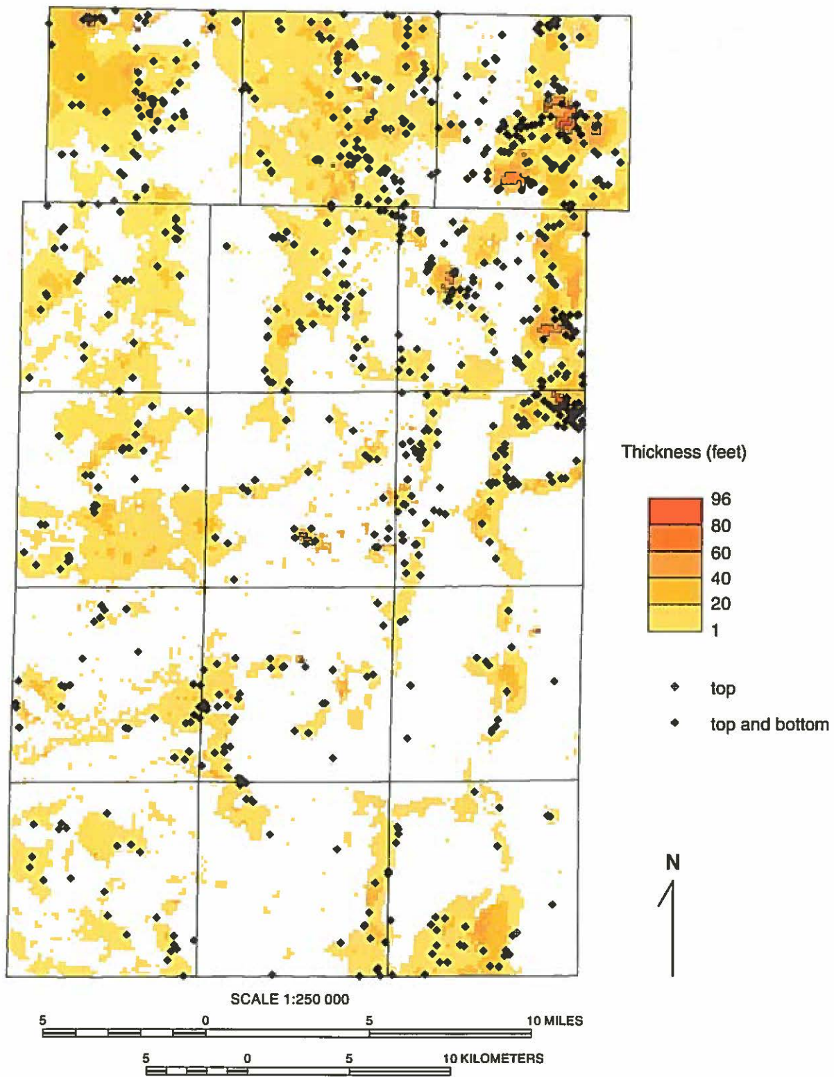
Figure 13 Isopach map of the surficial Henry Formation in Kane County and the distribution of primary wells used in mapping the unit.
