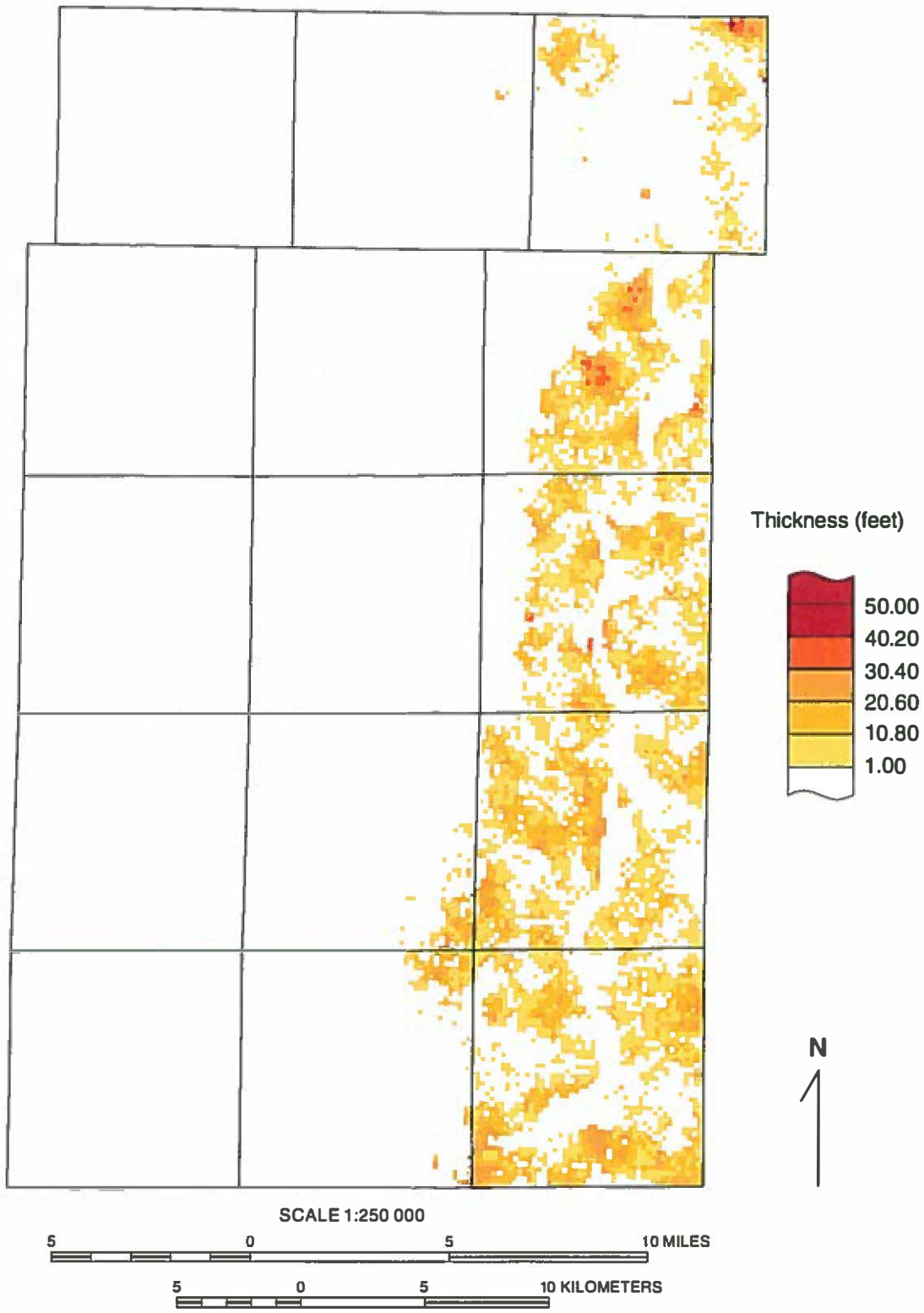
Figure A2 Simulation map of the thickness of the sub-Yorkville tongue of the Henry Formation showing large local variability.
