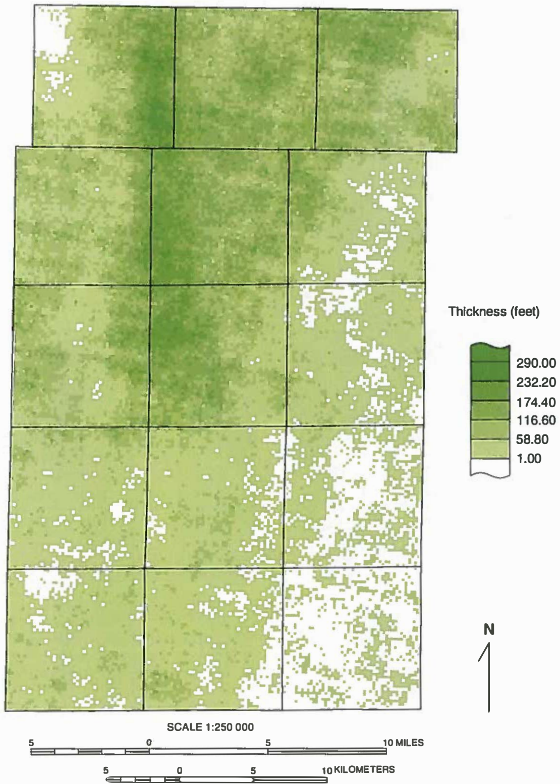
Figure A12 Simulation map of the thickness of the Tiskilwa Formation diamicton showing large local variability.
