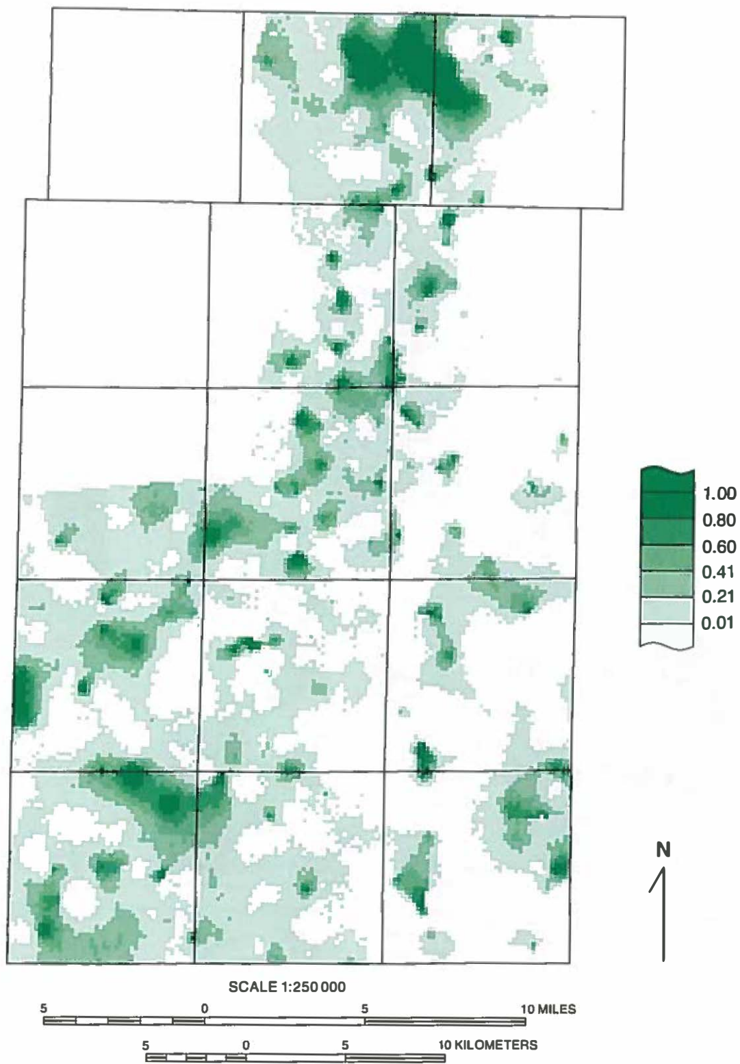
Figure A9 Probability that the Batestown Member diamicton is greater than 20 feet thick.
