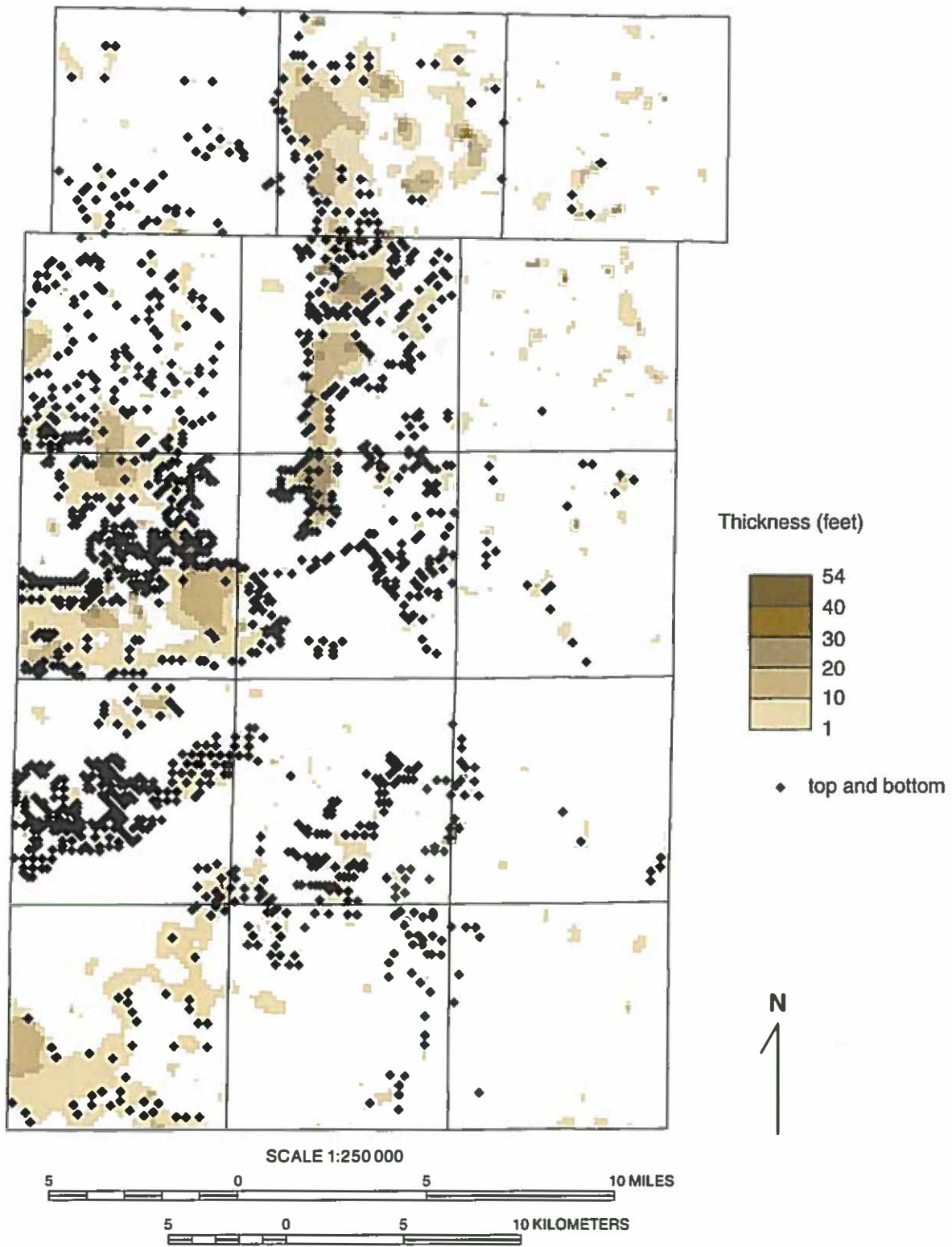
Figure 12 Isopach map of the surficial fine-textured layer (i.e., the combined thickness of Grayslake Peat, fine-textured facies of the Cahokia Formation, and surficial deposits of the Equality Formation) in Kane County and the distribution of synthetic data points used in mapping the unit.
