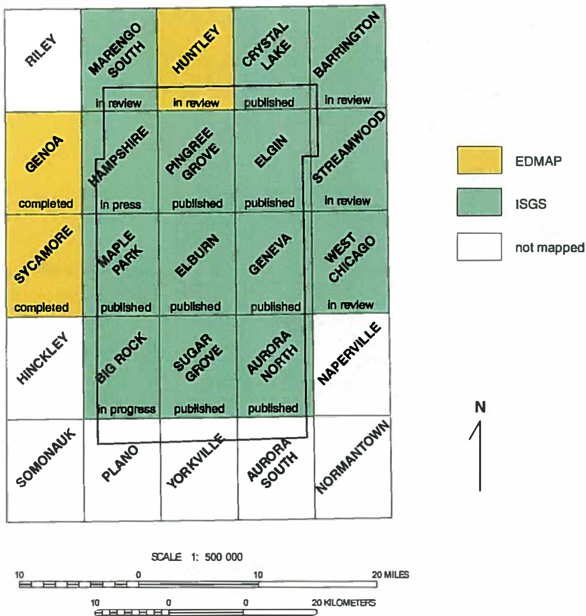
Figure 5 U.S. Geological Survey 7.5-minute quadrangles in Kane County and adjoining areas and the status of associated geologic maps.
