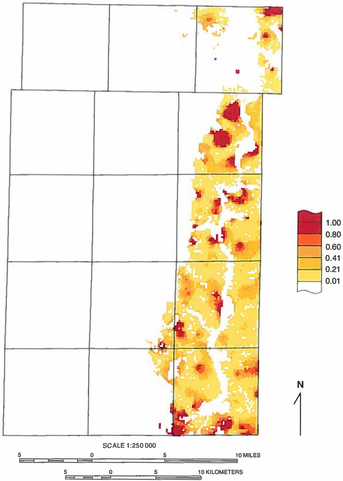
Figure A3 Probability that the sub-Yorkville tongue is greater than 10 feet thick.
