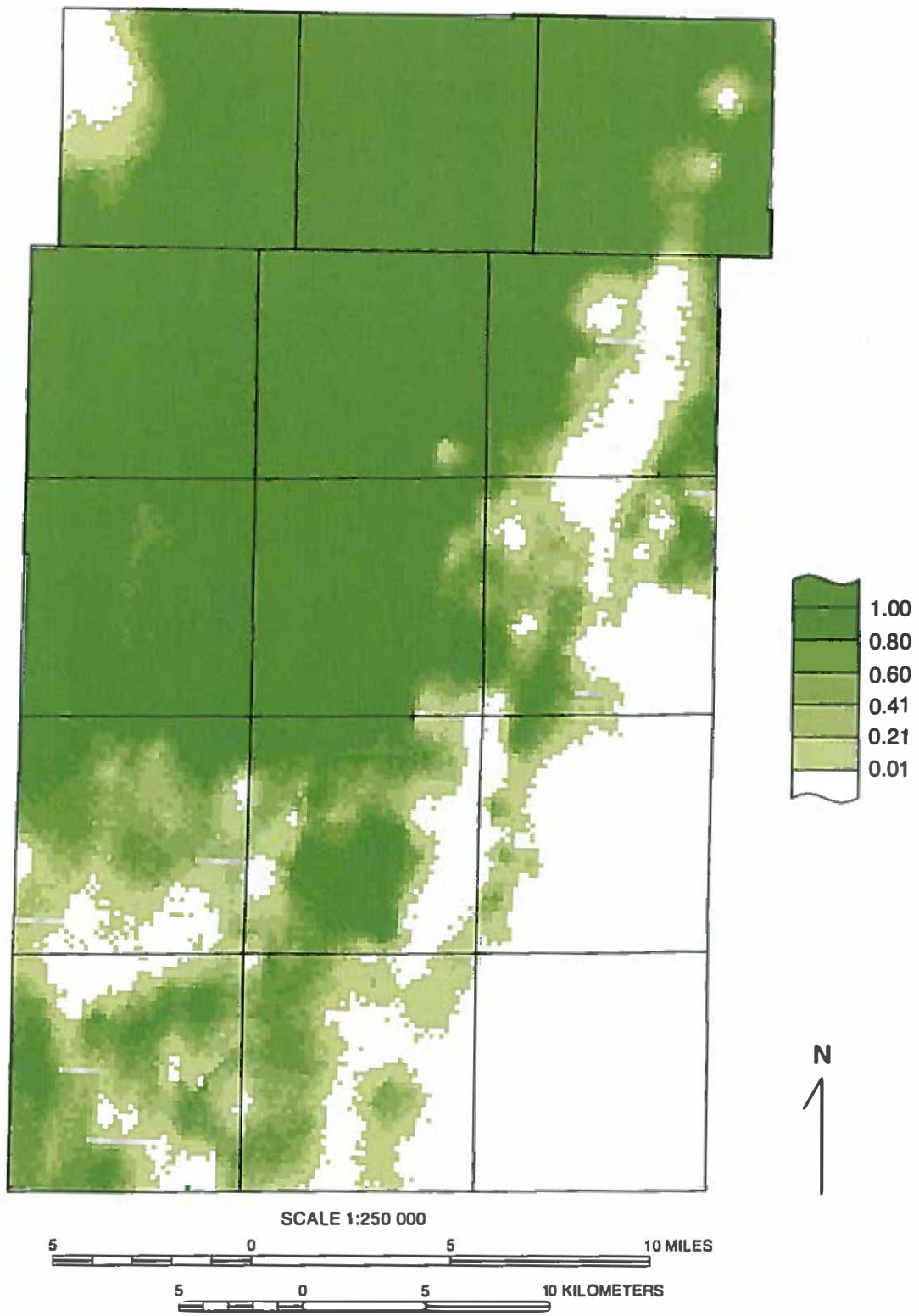
Figure A13 Probability that the Tiskilwa Formation diamicton is greater than 20 feet thick.
