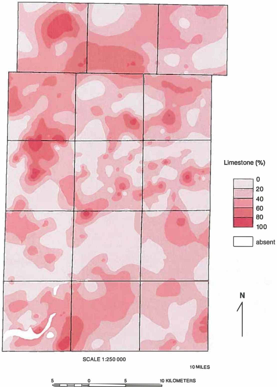
Figure 44 Estimates of percent carbonate rock by thickness of the Maquoketa Group of the Ordovician System in Kane County.
