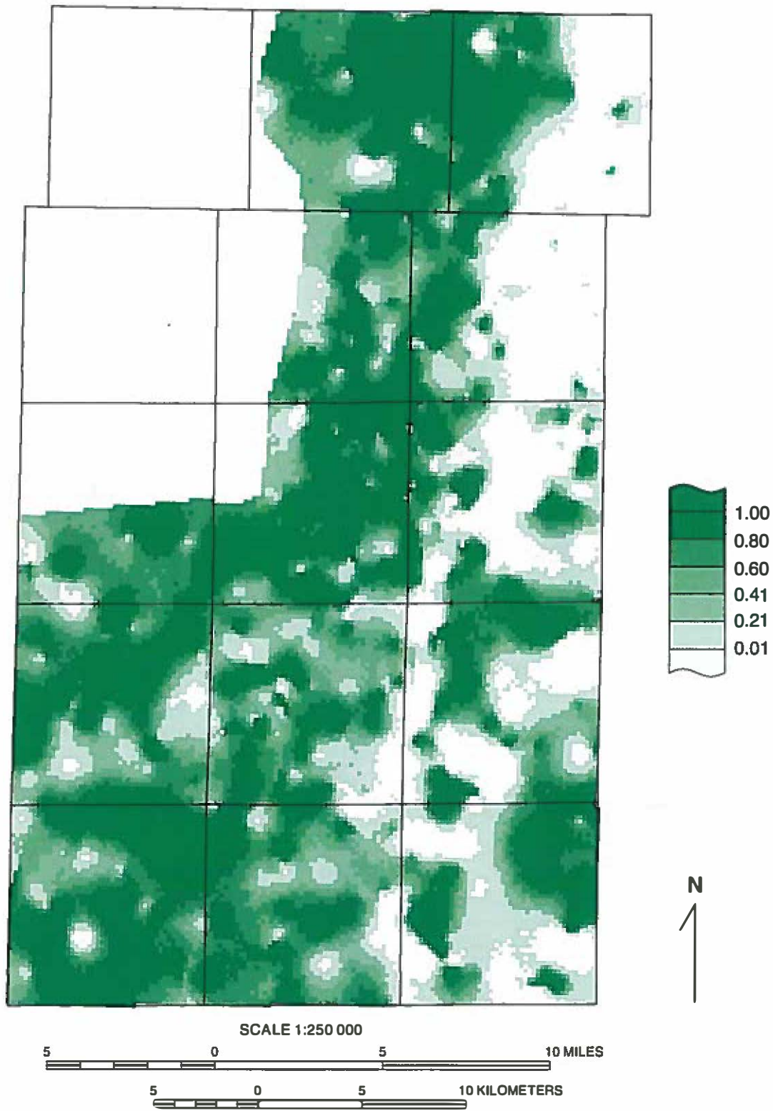
Figure A8 Probability that the Batestown Member diamicton is greater than 10 feet thick.
