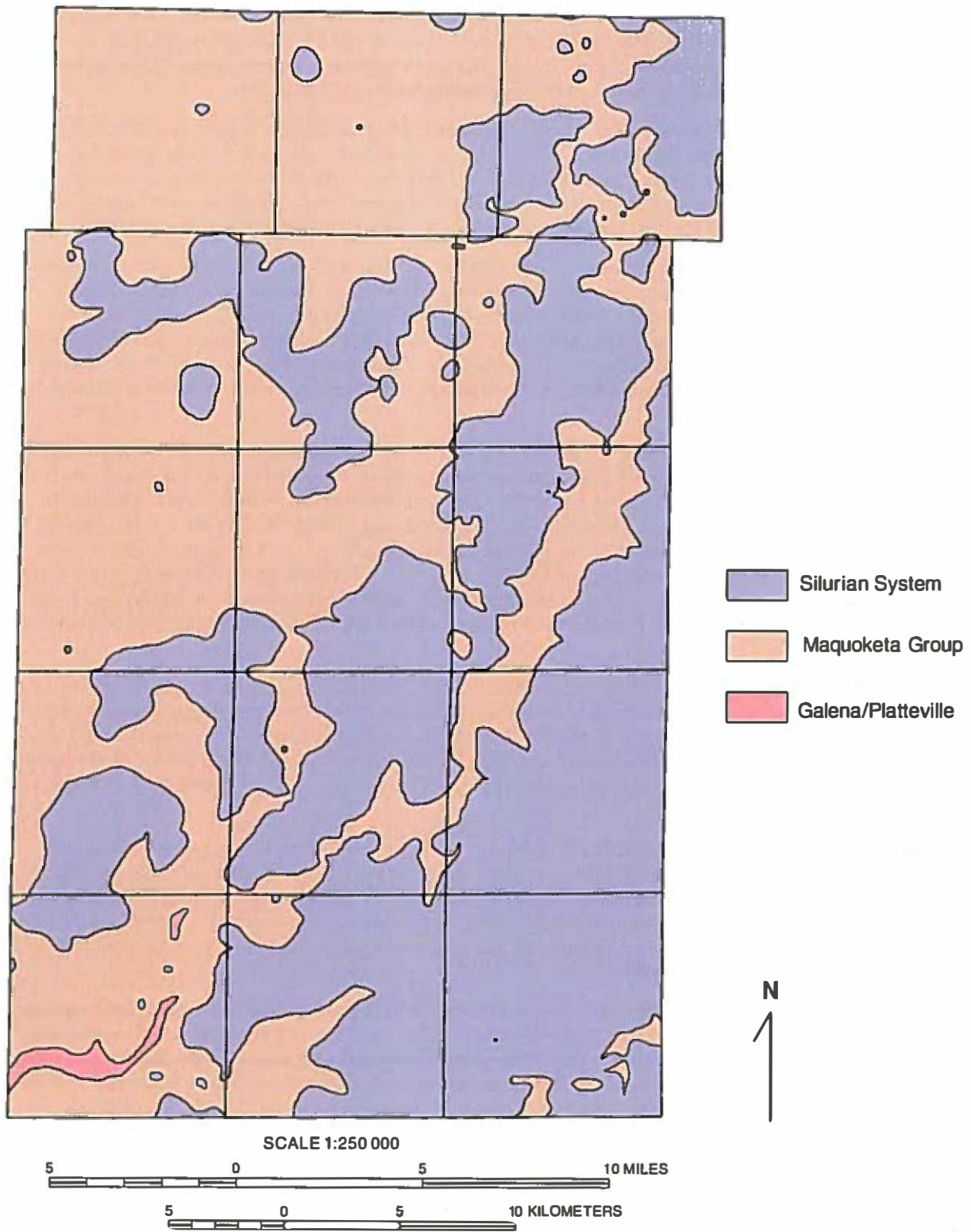
Figure 41 The subcrop pattern of the major stratigraphic bedrock units in Kane County.
