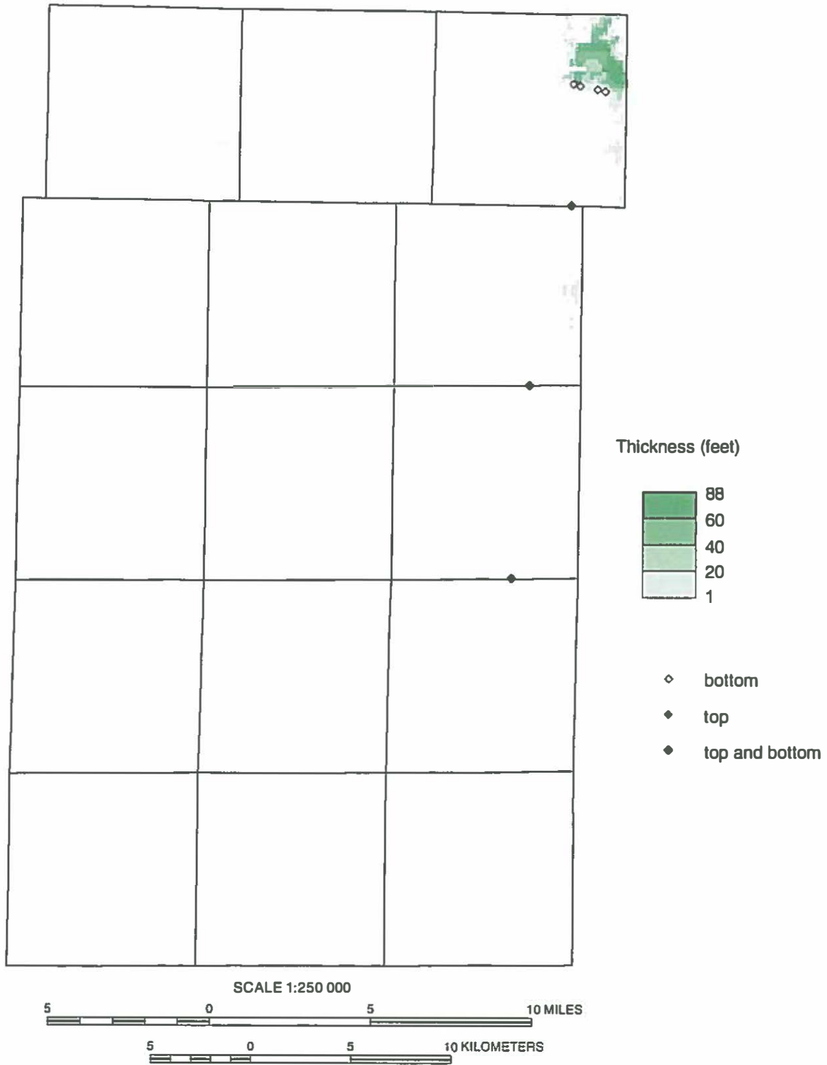
Figure 17 Isopach map of the Haeger Member, Lemont Formation, in Kane County and the distribution of synthetic data points used in mapping the unit.
