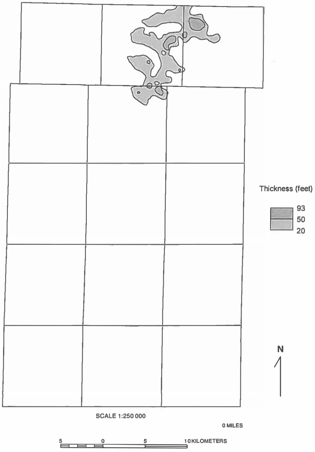
Figure 56 Distribution and thickness of the Gilberts aquifer in Kane County.
