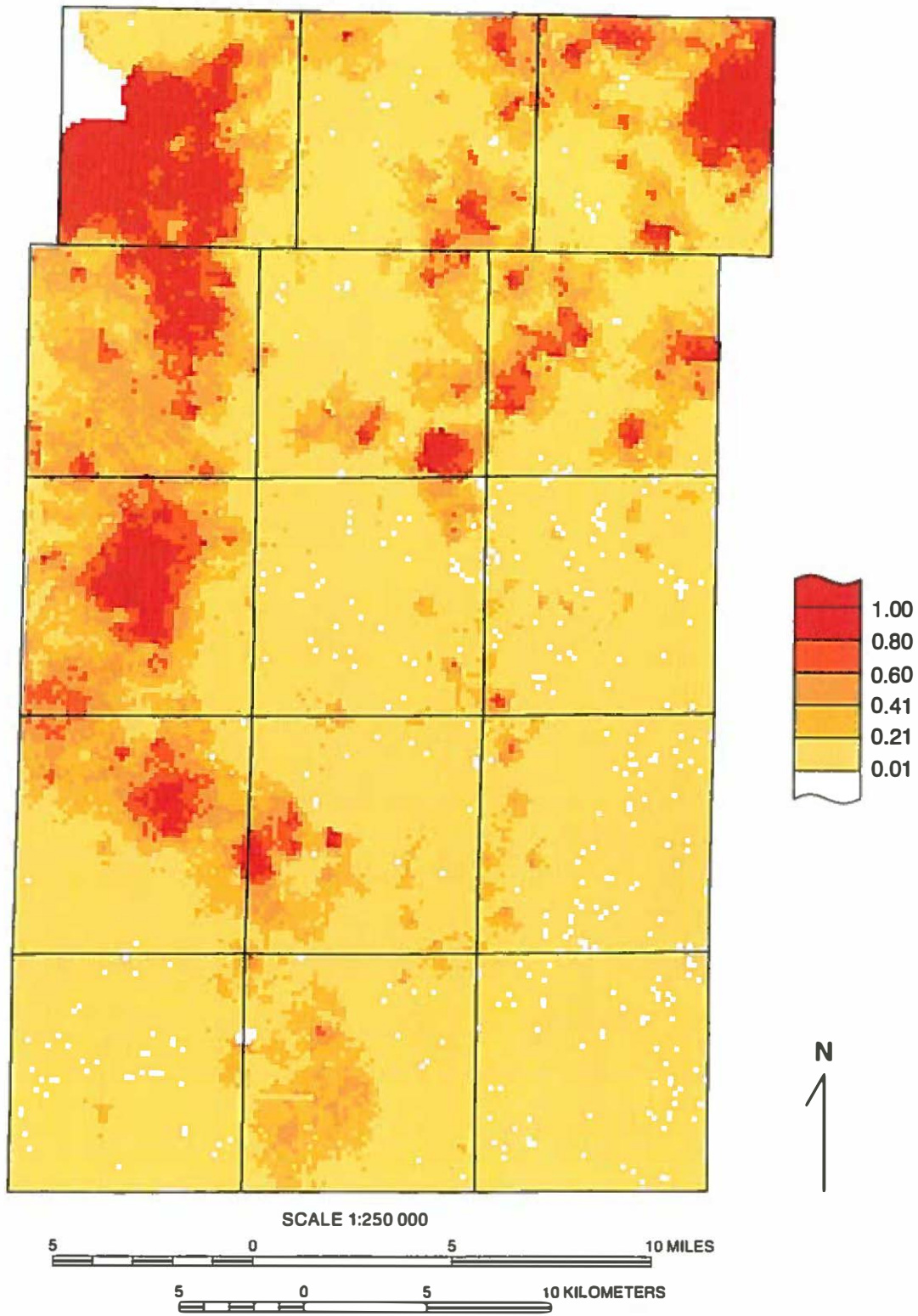
Figure A18 Probability that the Ashmore Tongue is greater than 10 feet thick. This map was based on the Step 2 simulation results.
