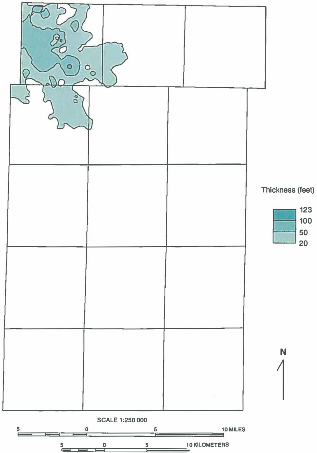
Figure 54 Distribution and thickness of the Hampshire aquifer in Kane County.
