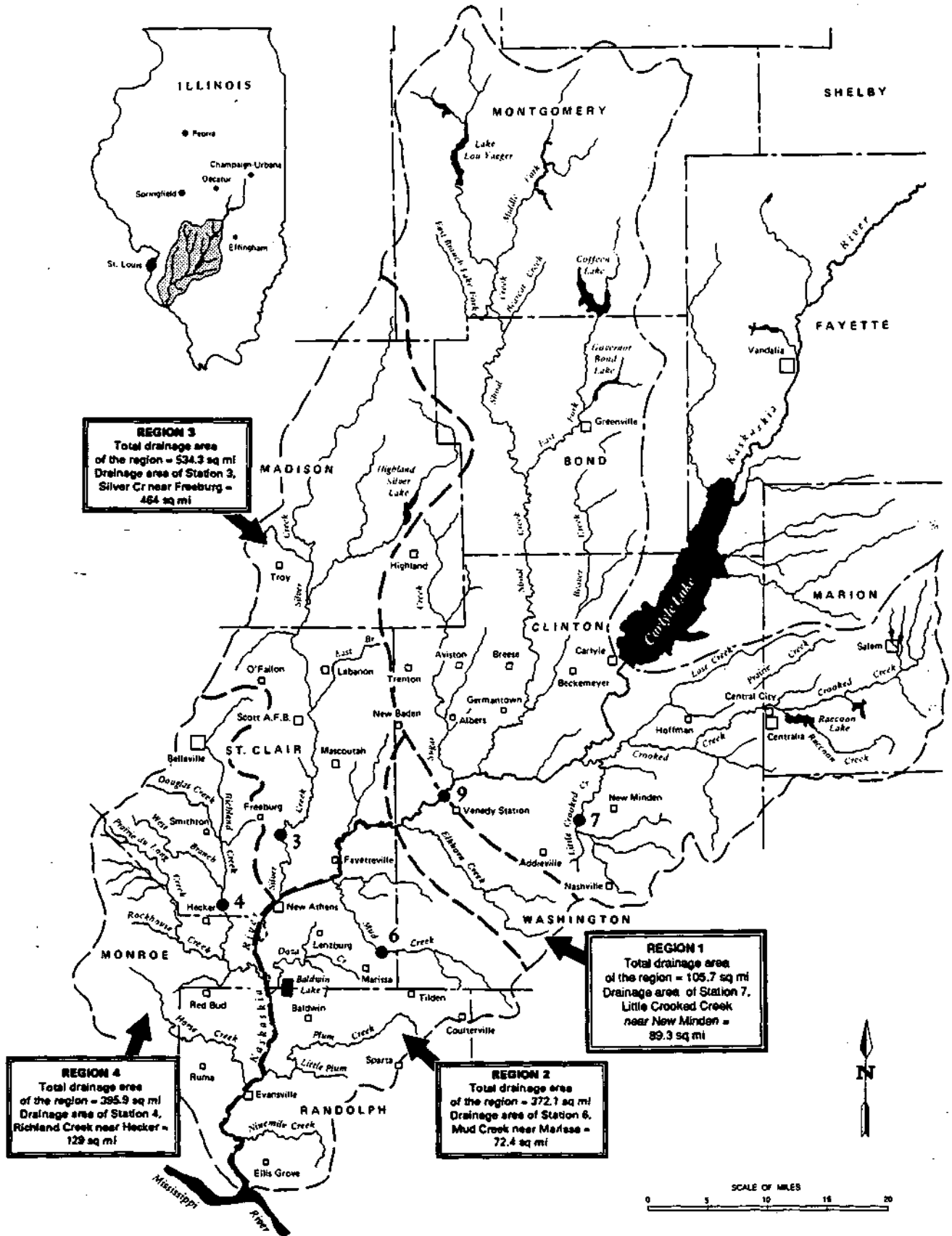
Figure 5. Division of the Kaskaskia River basin below Venedy Station into four hydrologically similar regions
