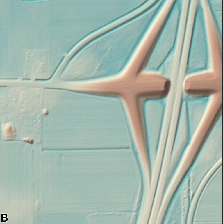
Figure 3 The feature shown is a cloverleaf structure associated with I-55 located at the Will County boundary (T32N, R09E). Figure 3A is a digital surface model (DSM), whereas Figure 3B is a DTM of the same area. In contrast to a DTM, which represents only ground features, a DSM portrays all aboveground features. For example, the roadway overpass (a) shown on the DSM has been removed on the DTM because the elevated roadway is not considered part of the ground surface. Likewise, the patterns of scattered points at (b) on the DSM represent the cables of an aboveground transmission line, which have been removed on the DTM. Vehicles moving along I-55 (c), building structures (d), and trees and other vegetation (e), all of which are visible on the DSM, have been removed on the DTM. Scale is 1:6,000 (1 in. = 500 ft).
