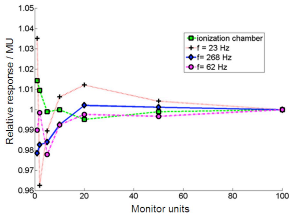
FIG. 8. Normalized photocell and ion chamber response per monitor unit ( R(m,f) / m ) as a function of monitor unit ( m_{ref} = 100, 6\text{ MV} ). Different sampling frequencies affect the total sensibility of the detector cell. Dose rate was r_{ref} = 400\text{ MU/min} .
