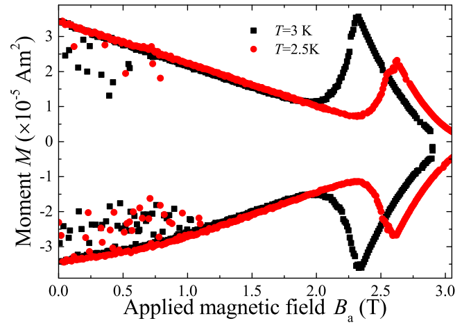
FIG. 1. Dependencies of magnetization on the applied magnetic field measured at standard VSM settings f = 40 Hz and A = 2 mm.
