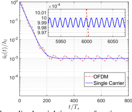
Fig. 3: Normalized weighting error functions with the loop gain \mu A^2=1000 , \alpha T_s=0.003 , T_o=80T_s , and \beta_s=\beta_o=0.25 .
