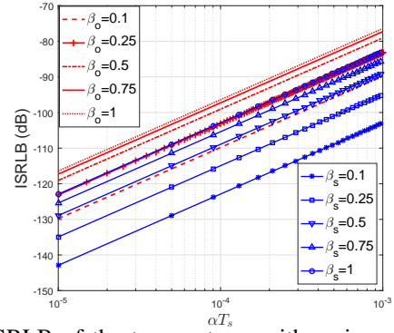
Fig. 5: ISRLB of the two systems with various values of \beta_s and \beta_o .
