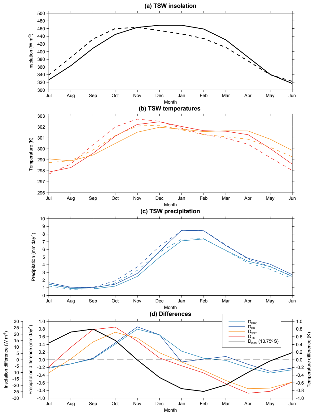
Figure 7. The monthly, ensemble and regional mean (a) insolation (taken at 13.75° S for insolation, black line, \text{W m}^{-2} ), (b) surface temperature (land and ocean combined, red line, K) and sea surface temperature (when available, amber line, K) and (c) total precipitation (blue line, \text{mm day}^{-1} ) and convective precipitation (turquoise line, \text{mm day}^{-1} ) at 0 ka (solid lines) and 6 ka (dashed lines) within the TSW box. The difference in those fields (insolation, temperature and precipitation) for 6 – 0 ka is plotted in (d).
