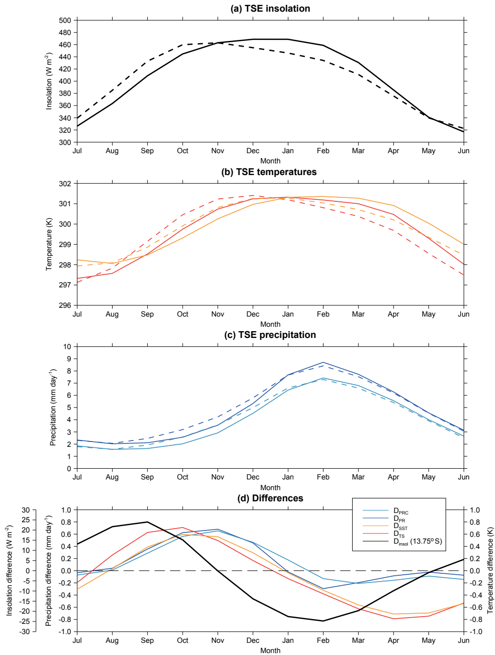
Figure 8. The monthly, ensemble and regional mean (a) insolation (taken at 13.75^{\circ} S for insolation, black line, W m^{-2} ), (b) surface temperature (land and ocean combined, red line, K) and sea surface temperature (when available, amber line, K) and (c) total precipitation (blue line, mm day^{-1} ) and convective precipitation (turquoise line, mm day^{-1} ) at 0 ka (solid lines) and 6 ka (dashed lines) within the TSE box. The difference in those fields (insolation, temperature and precipitation) for 6 – 0 ka is plotted in (d).
