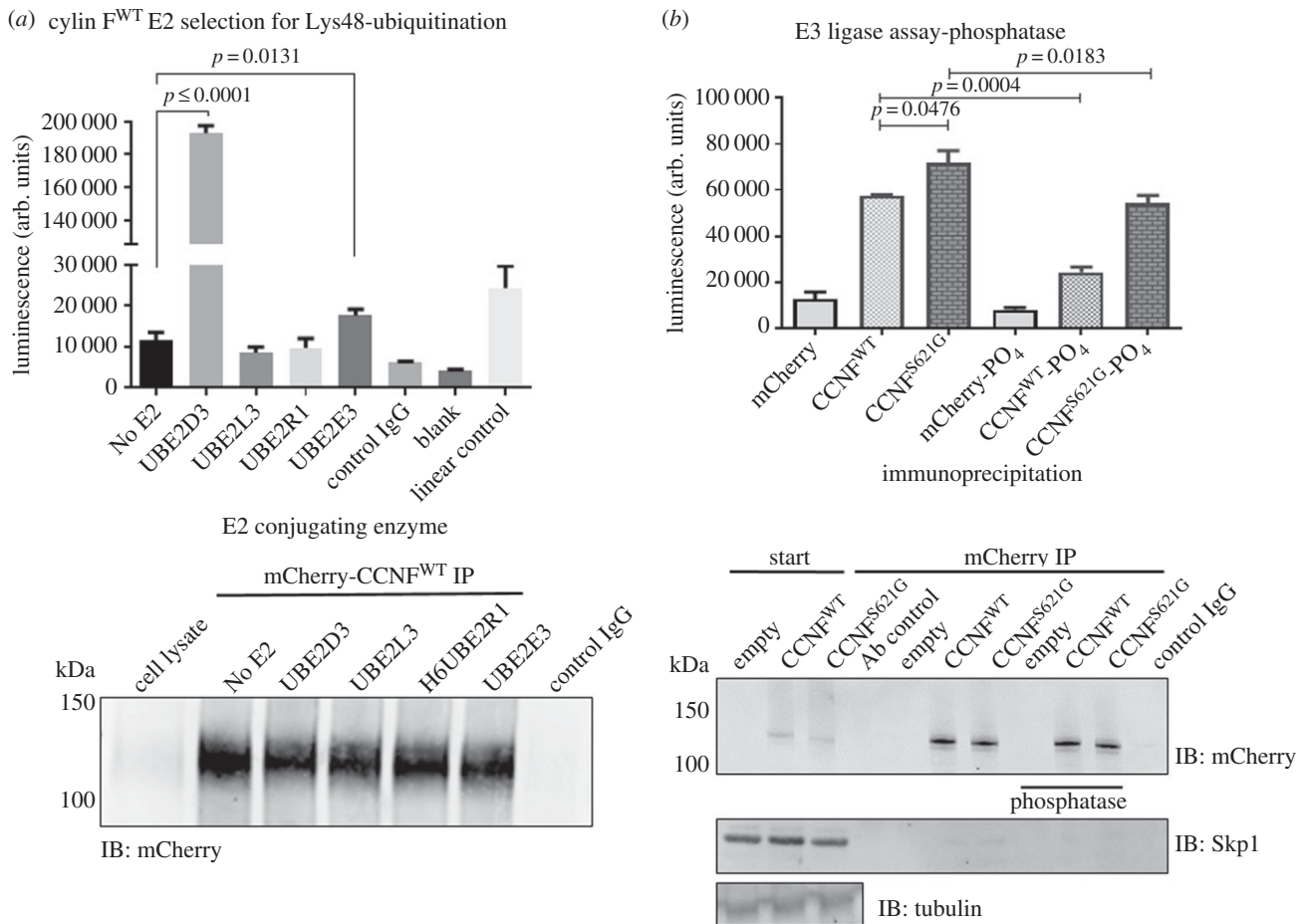
Figure 1. SCF (cyclin F) E3 ligase activity is regulated by phosphorylation. E3 ligase activity assays were used to assess the most suitable E2 conjugating enzyme for mCherry–cyclin F to ubiquitylate substrates. (a) Comparison of four common E2 enzymes (UBE2D3, UBE2L3, UBE2R1 and UBE2E3) found that UBE2D3 was the most suited and provided the highest conjugation activity for SCF (cyclin F) ( p \leq 0.0001 , n = 3 , Student's t -test) followed by UBE2E3 ( p = 0.0131 , n = 3 ). (b) SCF (cyclin F) was immunoprecipitated from transfected HEK293 cells, treated with Antarctic phosphatase and Lys48-specific E3 ligase activity was measured. The E3 ligase activity of cyclin F S621G appeared to be more active than the wild-type by approximately 1.3-fold ( n = 3 , p = 0.0476 , one-way ANOVA), and following dephosphorylation the E3 ligase activity of immunoprecipitated SCF (cyclin F) was significantly reduced in both mutant and wild-type cyclin F respectively by 1.3-fold ( p = 0.0183 , n = 3 , one-way ANOVA) and 2.3-fold ( p = 0.0004 , n = 3 , one-way ANOVA). Data are represented as the mean \pm s.e.m. using one-way ANOVA with Tukey's post hoc test. Immunoblots were carried out following E3 ligase activity assays to demonstrate equivalent levels of immunoprecipitated mCherry–cyclin F used for activity assays.
