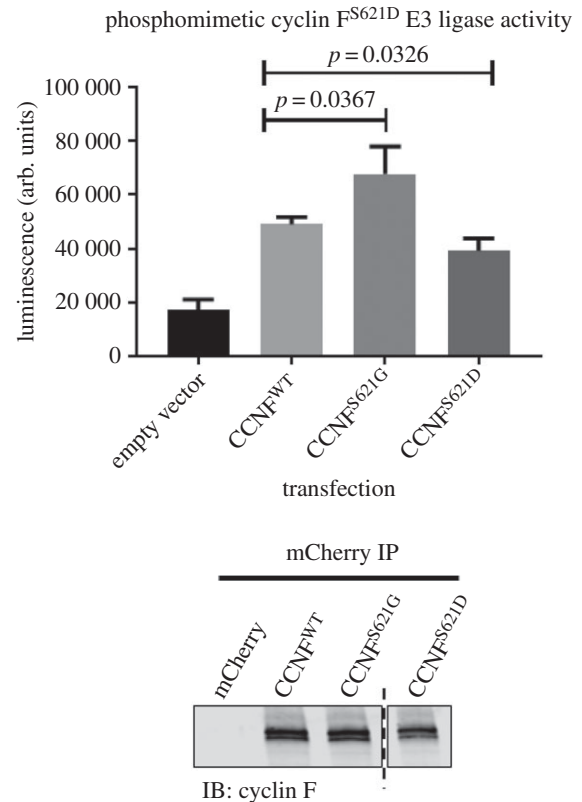
Figure 5. Phosphomimetic cyclin F S621D reduces SCF (cyclin F) Lys48-ubiquitylation activity. E3 ligase activity of immunoprecipitated phosphomimetic mCherry–cyclin F S621D was less active compared with the wild type by approximately 20% ( p = 0.0326 , n = 3 , Student's t -test). Immunoblots were carried out following E3 ligase activity assays to demonstrate equivalent levels of immunoprecipitated mCherry–cyclin F used for activity assays. Vertical dashed line indicates cropped lanes.
