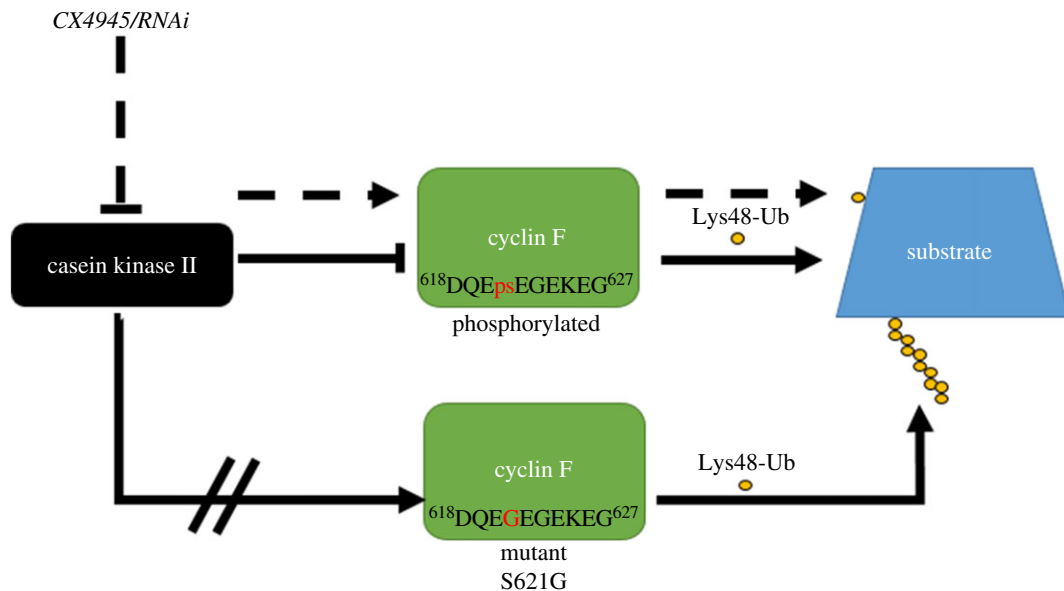
Figure 6. Proposed mechanism of phosphorylated Ser621 in cyclin F and its effect on the SCF^{(\text{cyclin F})} Lys48-ubiquitylation activity. CK2 is responsible for phosphorylating Ser621 in cyclin F and regulating the SCF^{(\text{cyclin F})} E3 ligase activity. Inhibition of CK2 activity by either CX4945 or siRNA knock down prevents phosphorylation of mCherry–cyclin F at Ser621 and elevates its Lys48-specific E3 ligase activity. Additionally, a mutation at Ser621 (p.Ser621Gly) has been found in a large multi-generational Australian family with ALS/FTD, and expression of this mutant version (cyclin F S621G ) in cells displays elevated Lys48-specific E3 ligase activity.
