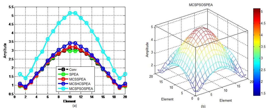
Figure 7. Optimal Excitation Amplitude for SPEA-based Rectangular Arrays 2(M \times N) = 20 \times 20 , Dolph-Chebyshev, \maxIter = 1000 . (a) We compare four SPEA-based and conventional rectangular antenna arrays excitation amplitude in 2D plot. (b) The proposed MCSPSOSPEA rectangular array excitation amplitude in 3D plot.
