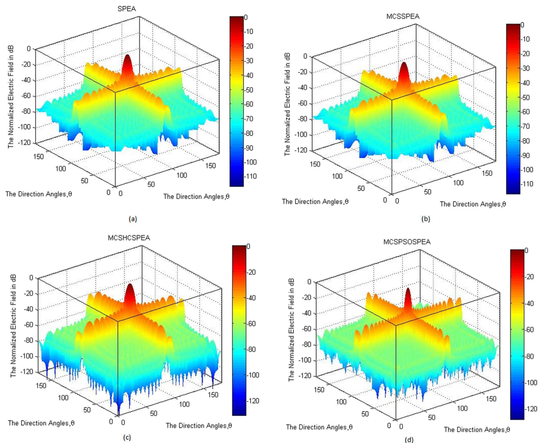
Figure 6. 3D Normalized Antenna Pattern for SPEA-based Rectangular Arrays 2(M \times N) = 20 \times 20 , Dolph-Chebyshev, \maxIter = 1000 . We simulate four SPEA-based rectangular arrays, which are (a) Original SPEA. (b) Hybrid MCSSPEA. (c) Hybrid MCSHCSPESA. (d) Hybrid MCSPSOSPEA.
