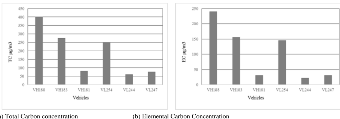
Fig.4. TC and EC concentrations for different test vehicles [11]
