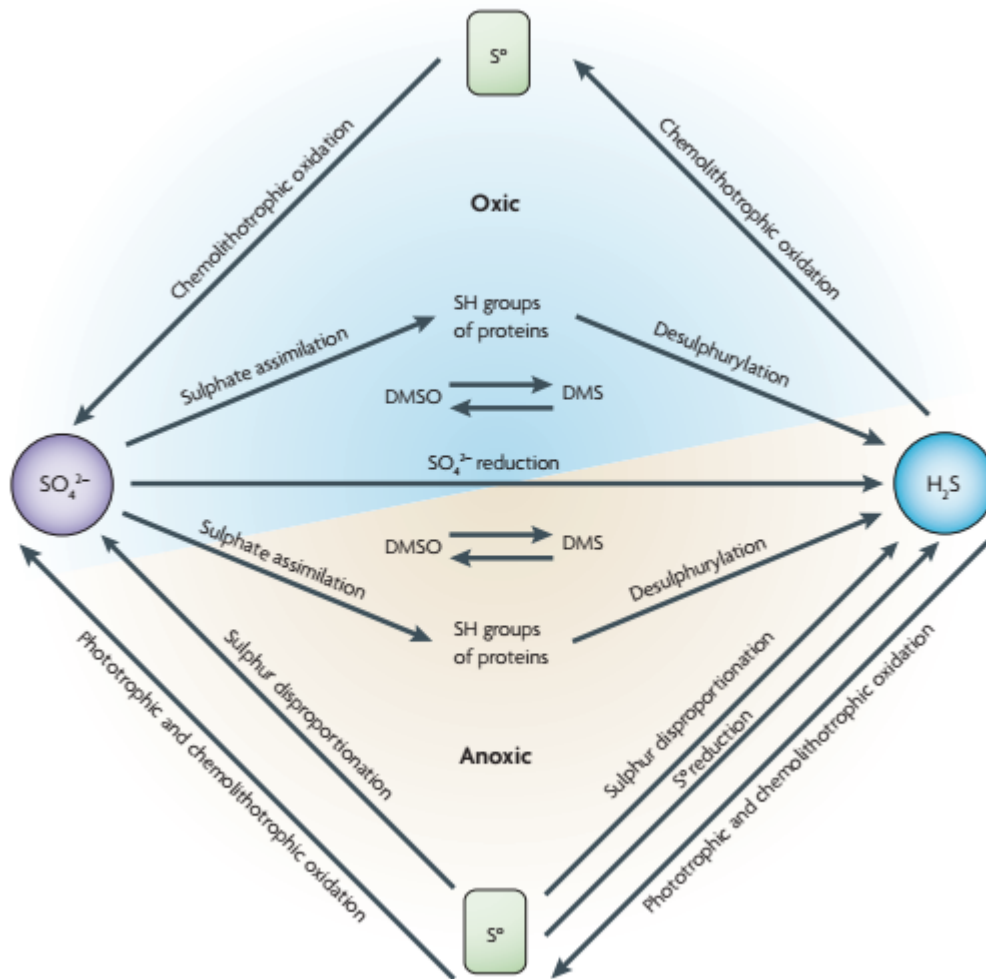
Figure 6: Microbial metabolic sulfur transformation pathways. Sulfate-reducing bacteria (SRB) use sulfate ( \text{SO}_4^{2-} ) as a terminal-electron acceptor in the degradation of organic matter, which results in the production of hydrogen sulfide ( \text{H}_2\text{S} ). Subsequently, the sulfide can be oxidized through a variety of metabolic pathways via sulfur-oxidizing bacteria to elemental sulfur ( \text{S}^0 ) and \text{SO}_4^{2-} . Other transformations carried out by specialized groups of microorganisms result in sulfur reduction and sulfur disproportionation. Organic sulfur compounds (i.e. dimethyl sulfoxide; DMSO) can be transformed into dimethyl sulfide (DMS) and vice versa by several groups of microorganisms. From Muyzer and Stams (2008).
