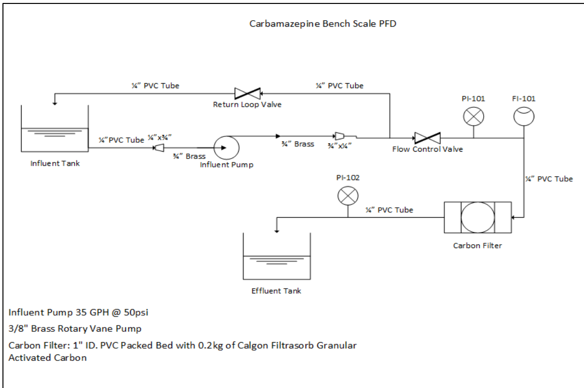
Figure 7.3.2 Packed Bed Process Flow Diagram
