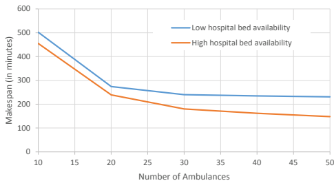
(a) Makespan C_{max}|F_w vs No of ambulances
