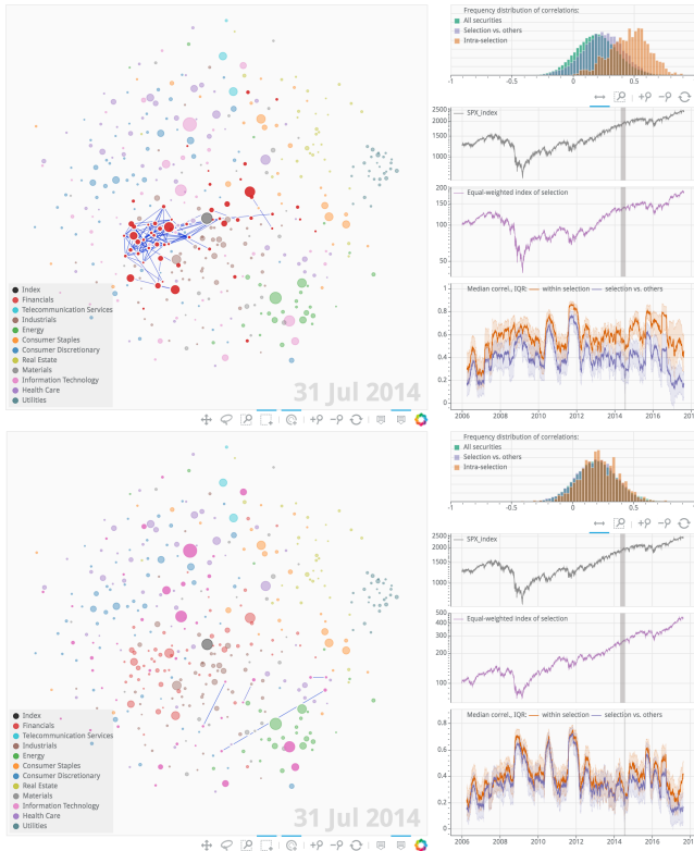
Figure 8: Industry sectors with different levels of homogeneity exhibit different behaviours in the swarm (links for r < 0.7 filtered out in all examples). Upper: Central clustering ( B4 ): stocks in the financials group (red) are less tightly bunched than utilities or energy stocks, but occupy a central location in the swarm. Lower: Broad dispersion ( B6 ): IT sector (magenta) stocks are scattered throughout a wide area of the swarm. The histogram shows that their correlation structure is similar to that of the entire market's. In fig. 1: Peripheral bunching ( B5 ): the utilities sector exhibits high intra-sector correlation and low correlation to other stocks.
