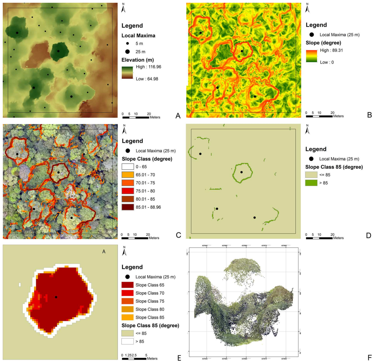
Fig. 2. All the detected treetops—local maxima within circular neighbourhoods of 5 m—overlaid on the Digital Surface Model (A); Local maxima within 25-m radius overlaid on the slope raster (B); Polygons representing slope classes greater than 65° overlaid on the ortho-mosaic (C); Binary classification of polygons generated from a DSM with 85° as the cut-off (D); Tree polygons enclosed by slope classes 65°–85° (E); and an RGB image generated in ArcMap™ 10.1 from the UAV point cloud within 25-m radius of the located treetop, with Northing on the X-axis and Elevation on the Y-axis (F).
