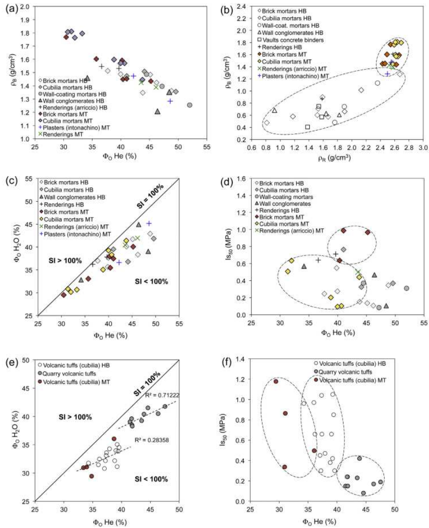
Fig. 8. Physical properties of mortars and cubilia stones from Maritime Theater (MT) mortars and, to make a comparison, from nearly Helicaminus Baths building (HB): (a) He open porosity ( \Phi_{He} ) vs bulk density, divided in different groups of mortar typology; (b) bulk density vs real density, (c) helium open porosity vs water open porosity of mortars, (d) He open porosity ( \Phi_{He} ) vs punching strength of mortars, (e) helium open porosity vs water open porosity of cubilia pyroclastites, (f) He open porosity ( \Phi_{He} ) vs punching strength of cubilia pyroclastites.
