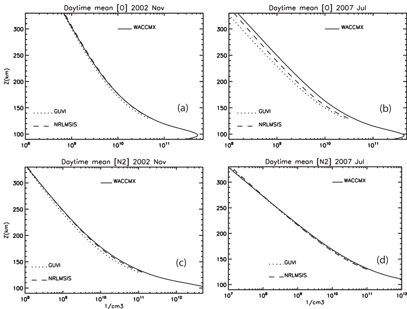
Figure 4. Similar to Figure 3, but comparing (a, b) O and (c, d) N 2 number densities for (a, c) solar maximum and (b, d) solar minimum conditions.
