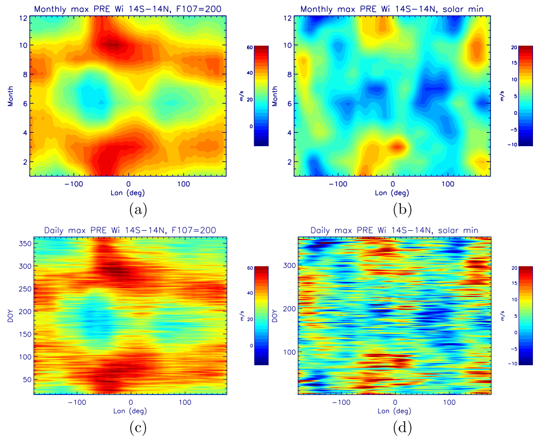
Figure 11. (a,b) Monthly averaged values of maximum pre-averaged enhancement (PRE) between 14°S and 14°N from WACCM-X simulations under solar maximum and solar minimum conditions, respectively. (c, d) Similar to Figures 11a and 11b but daily values of PRE.
