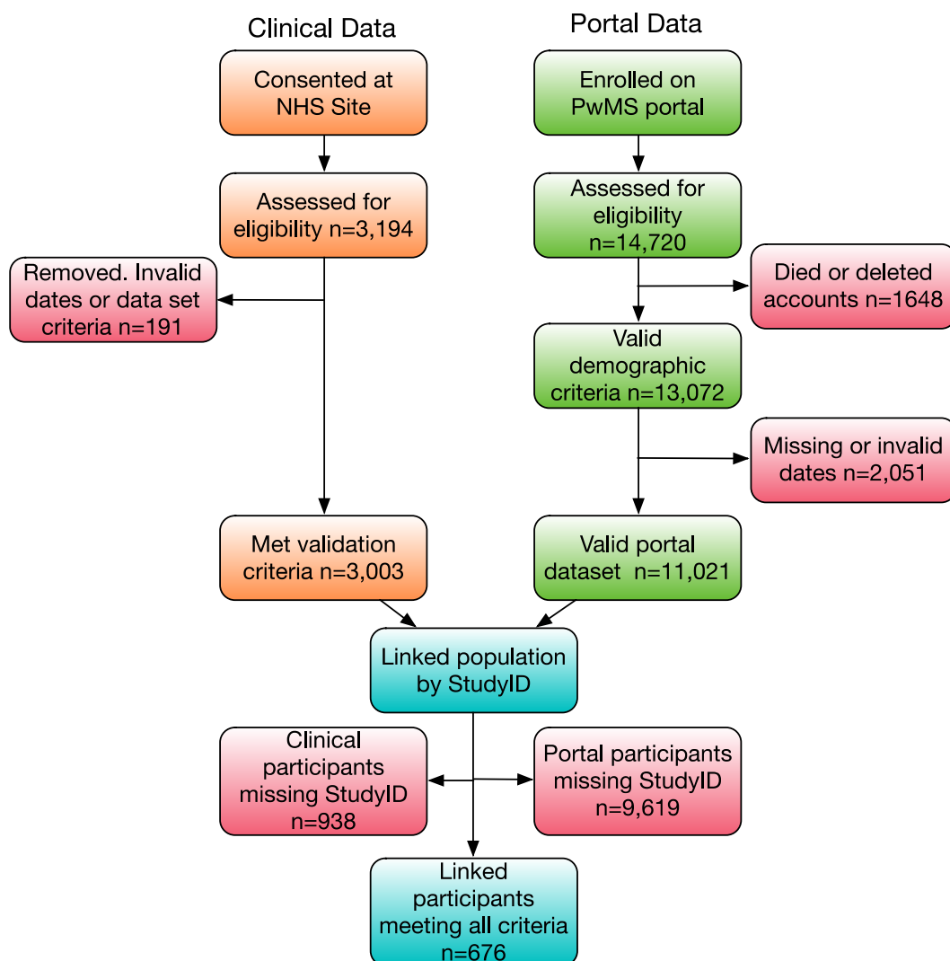
Figure 2: Consort diagram showing data selection criteria
