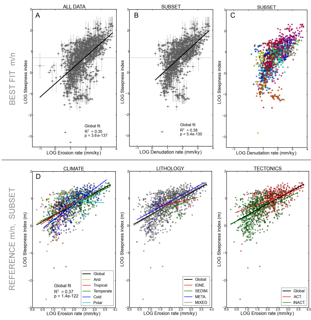
Fig. 5: Channel steepness, M_\chi , against denudation rates E in log-log scale. (A) and (B) The nonnormalized full and \bar{p} \leq 0.16 subset data, respectively, with error bars. (C) The same subset with symbol colors identifying the different zones. On the second row, (D), (E), and (F) the \bar{p} \leq 0.16 subset data with fixed m/n_{ref} = 0.5 , showing specific colors and linear regressions for each category under the climate, lithology, and tectonics subgroups, respectively.
