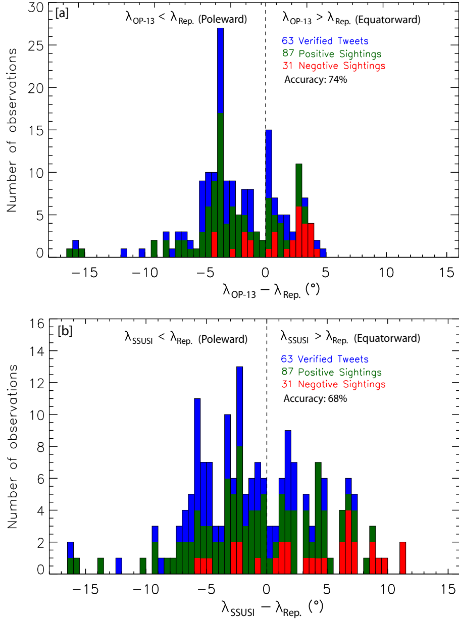
Figure 5: Histogram plots showing the distribution of latitude difference between citizen science reports ( \lambda_{Rep.} ) with fixed flux level boundaries obtained from [a] OVATION Prime 2013 model ( \lambda_{OP-13} ) and [b] Zhang-Paxton empirical auroral model ( \lambda_{SSUSI} ). The stacked bars represent number of different types of reports (red: negative reports, green: positive sightings, and blue: verified tweets) in each 0.5^\circ geomagnetic latitude bins.
