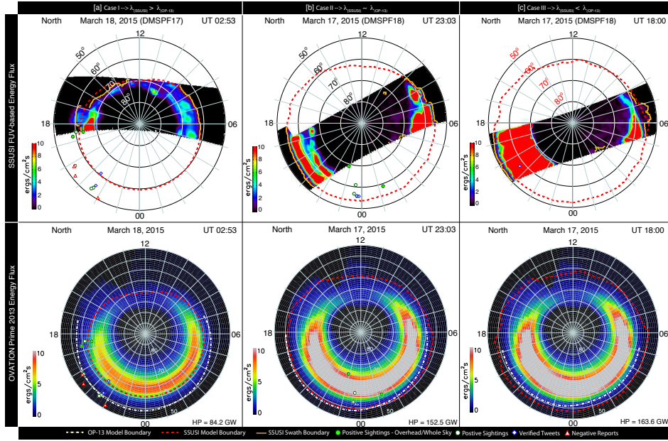
Figure 6: Three typical cases [a] \lambda_{SSUSI} > \lambda_{OP-13} , [b] \lambda_{SSUSI} \sim \lambda_{OP-13} , and [c] \lambda_{SSUSI} < \lambda_{OP-13} are identified from 36 conjunctions to emphasize the differences and similarities between data and models. Top panel shows the auroral energy flux map obtained from FUV images captured by the SSUSI instrument on board DMSP satellites F-17 and F-18 during 17-18 March 2015 for three different conjunctions. Bottom panel shows the output of the summed energy flux ( \sum j ) for four auroral types predicted by OP-13 auroral precipitation model for the same conjunction times. The Zhang-Paxton model boundary is shown on both panels for ease of comparison.
