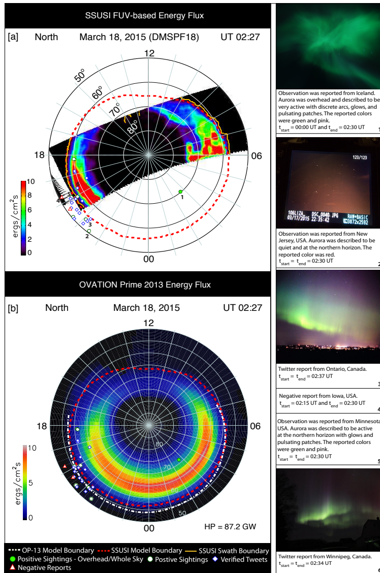
Figure 3: Plot of citizen science data together with [a] the auroral energy flux map obtained from FUV image captured by the SSUSI instrument on board DMSP-F18 satellite and [b] the output of the summed energy flux ( \sum_j ) for four auroral types predicted by the OP-13 auroral precipitation model for 18 March 2015 at 02:27 UT. The yellow solid line outlining the FUV image is the SSUSI swath boundary. 26 citizen science reports that fall within the conjunction criteria include all types of reports. For illustrating report contents, we have numbered a few from one to six in Panel [a]. A detailed description of each report is given in the boxes with corresponding numbers on the right (additional metadata and precise location are typically available).
