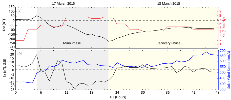
Figure 1: Variation of (a) Dst (black curve) and Kp (red curve) indices and (b) IMF Bz (black curve) and solar wind speed (blue curve) during 17-18 March 2015. All data are obtained from the OMNI data set provided by NASA Goddard Space Flight Center. Except the Kp index (3-hourly average), all parameters are hourly averaged. The vertical dashed line separates the days. The gray and yellow shaded regions correspond to the main and the recovery phases of the storm, respectively.
