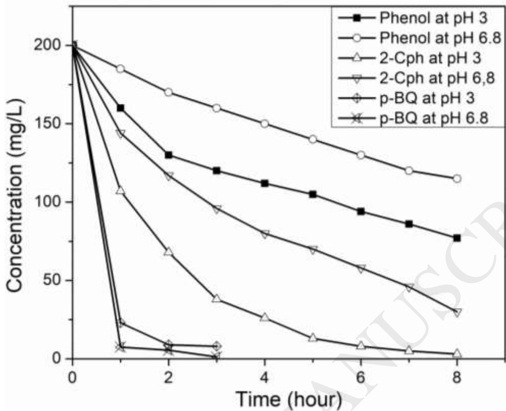
Figure 7. Electrochemical degradation of 200 mg/L of p-BQ, 2-Cph, and phenol in different pH solutions (pH 3 and pH 6.8) with 0.25 M Na 2 SO 4 as supporting electrolyte and 25 °C temperature.
