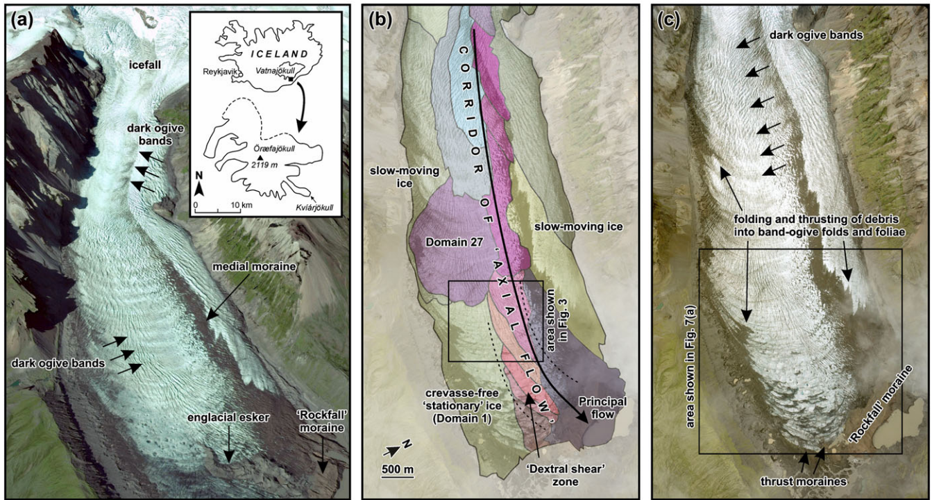
Figure 1. (a) Oblique view of Kviárjökull, December 2012 (copyright Google Earth). Annotated features are discussed in the text. (b) Domains mapped by Phillips et al. (2017), superimposed onto an August 2009 aerial image. Annotations highlight an ‘axial flow’ corridor of more elongate lobes, and deflection of flow toward the true-left by dextral shear near the terminus, as proposed by Phillips et al. (2017). (c) Annotated aerial image showing a heavily crevassed ice surface, and highlighting dark ogive banding and prominent transverse englacial foliation. The dark ogive banding first appears immediately below the ice fall, see (a). The thrusts and the lighter-coloured ‘rockfall’ moraine are discussed in the text. [Colour figure can be viewed at wileyonlinelibrary.com ]
