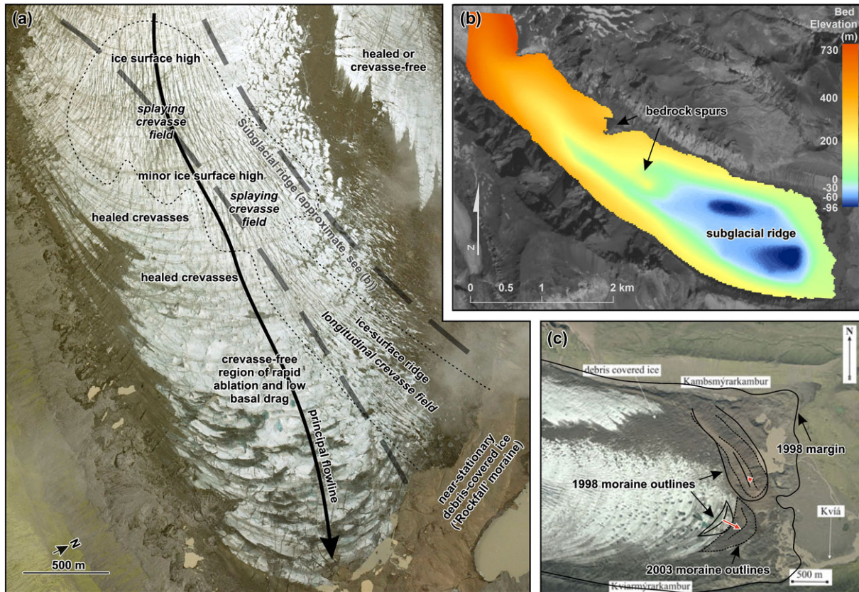
Figure 7. (a) Interpreted crevasse and flow patterns near the terminus. The thin dashed line defines an area of open crevasing, with active crevasing annotated in italicised text. Thick semi-transparent dashed lines indicate the approximate location of the subglacial ridge shown in (b). Arcuate development of transverse foliae indicates that the central flowline (black arrow) is directed through the crevasse-free area toward the true-right, in agreement with feature-tracking (Figure 2(b)). (b) Bed topography of the tongue and terminus region (Magnússon et al. , 2012). (c) Mapped displacement of prominent surface debris accumulations between 1998 and 2003. Displacement of the 'rockfall' moraine (see Figure 1(a)) is c. 100 m, whereas displacement of the emergent thrust moraine crest in the crevasse-free area is 300 to 500 m. The background to (c) has been obtained from Phillips et al. (2017). [Colour figure can be viewed at wileyonlinelibrary.com ]
