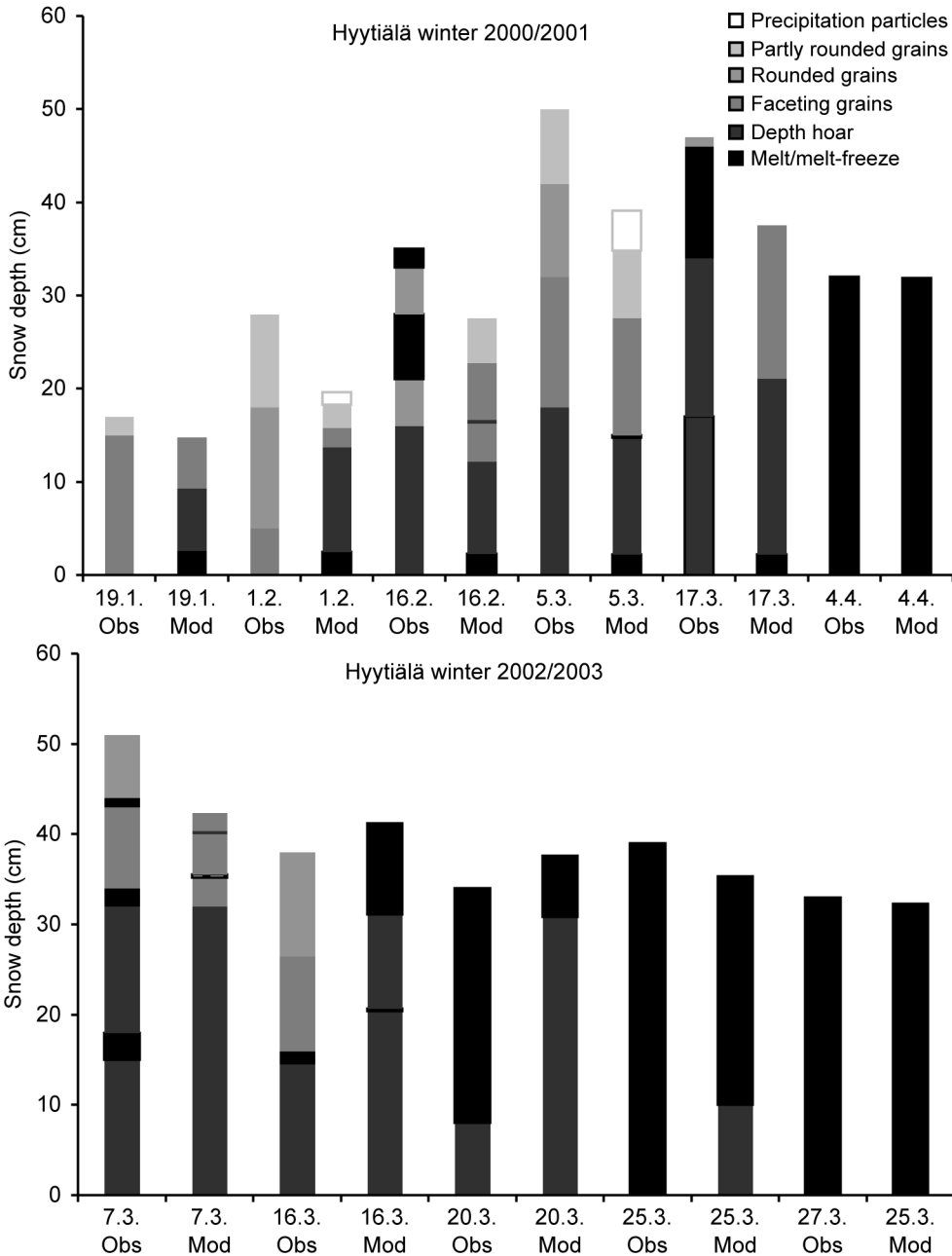
Fig. 6. The observed and model snow pack structure in Hyttiälä during early and late winter 2000/2001 and during melt period 2002/2003.
