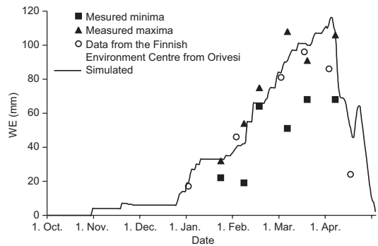
Fig. 3. Snow water equivalents (WE) in Hyttiälä in winter 2000/2001.
