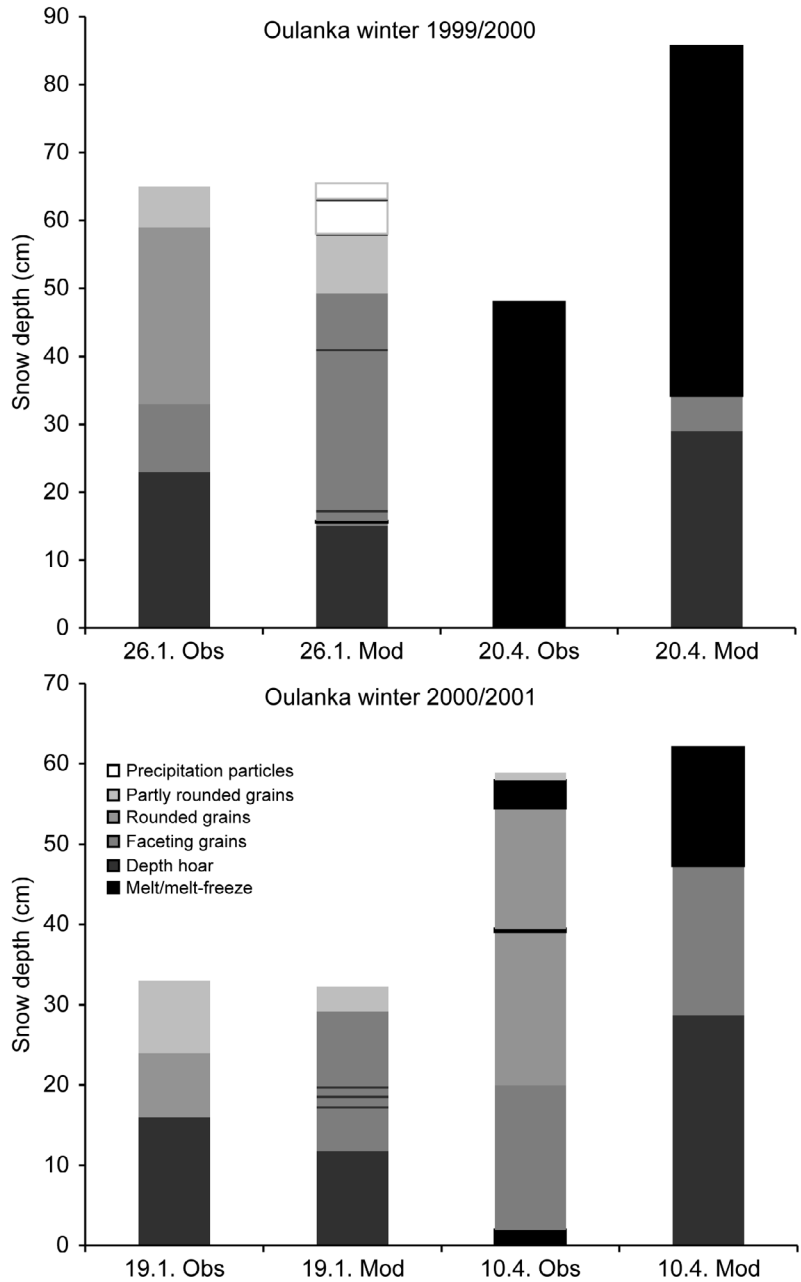
Fig. 8. The observed and modelled snow pack structure in Oulanka during early and late winters 1999/2000 and 2000/2001.
