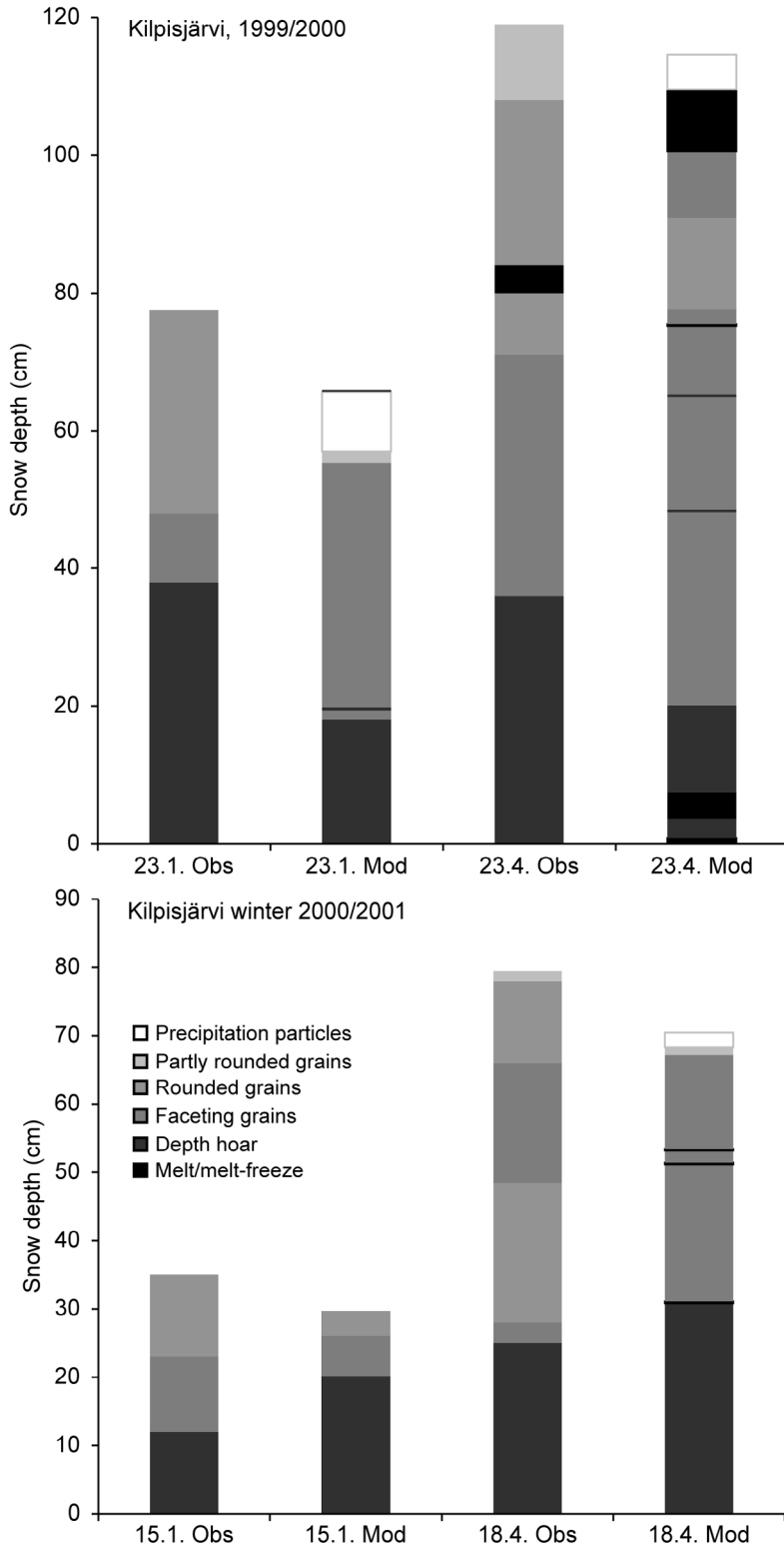
Fig. 9. The observed and modelled snow pack structure in Kilpisjärvi during early and late winters 1999/2000 and 2000/2001.
