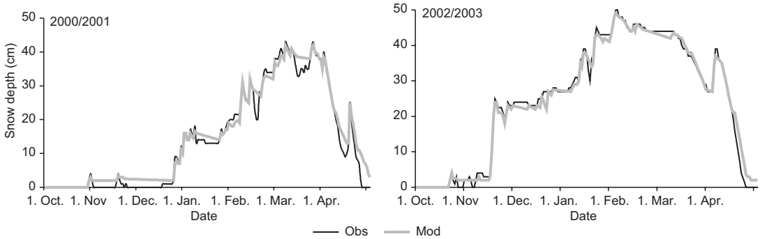
Fig. 2. The measured and simulated snow depths in winter in Hyttiälä. Snow depth data by FMI.
