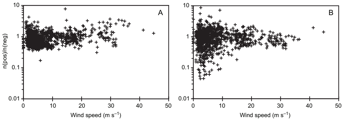
Fig. 6. Ratio between positive and negative ion concentrations as a function of wind speed. (A) cluster ions, and (B) intermediate ions.
