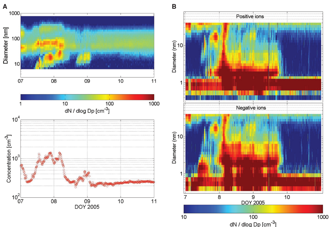
Fig. 3. (A) Neutral + charged particle size distributions (upper panel) and concentrations (lower panel) (DMPS measurements), and (B) air ion size distributions on 7–10 January 2005.
