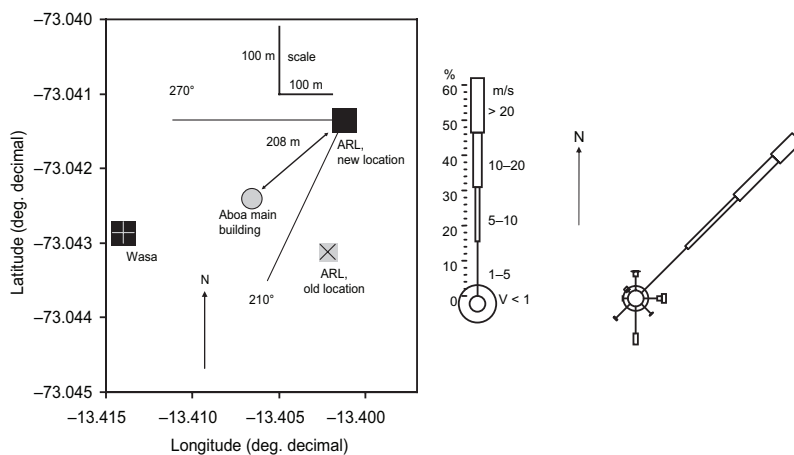
Fig. 1. Location of the aerosol research laboratory (ARL) of Aboa, the contamination sector, and the directional distribution of wind speeds during the FINNARP 2004 expedition.
