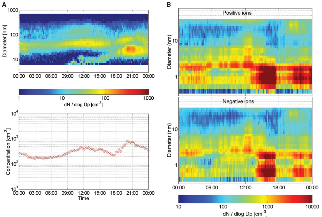
Fig. 7. Example of a day that was classified (A) into the event class 1 for the DMPS data but (B) into the class WIP for the air ion data.
