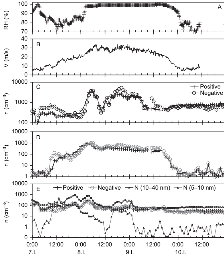
Fig. 4. Weather and air ion data on 7–10 January 2005. (A) Relative humidity, (B) wind speed, (C) cluster ion concentrations, (D) intermediate ion concentrations, and (E) overlapping range (10–40 nm) air ion concentrations and particle concentrations measured with the DMPS (N(10–40 nm) and N(5–10 nm)).
