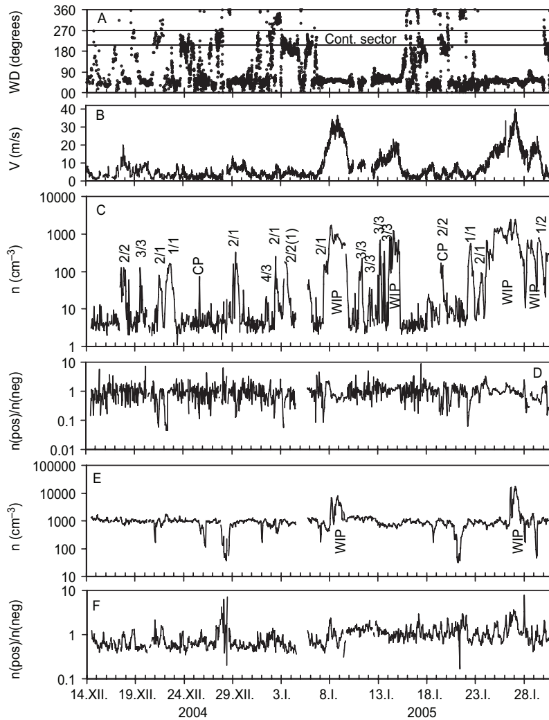
Fig. 2. Wind and air ion data during the campaign. (A) wind direction (WD) (Cont. sector = contaminated sector), (B) wind speed, (C) intermediate ion concentrations (positive + negative ions), (D) the ratio of positive and negative intermediate ion concentrations, (E) cluster ion concentrations (positive + negative ions), and (F) the ratio of positive and negative cluster ion concentrations from top to bottom, respectively. The numbers in panel C denote the event type (positive ion event type/negative ion event type). Non-event day classification numbers are not presented. WIP: Wind/snow-induced Particles, CP: Contamination particles.
