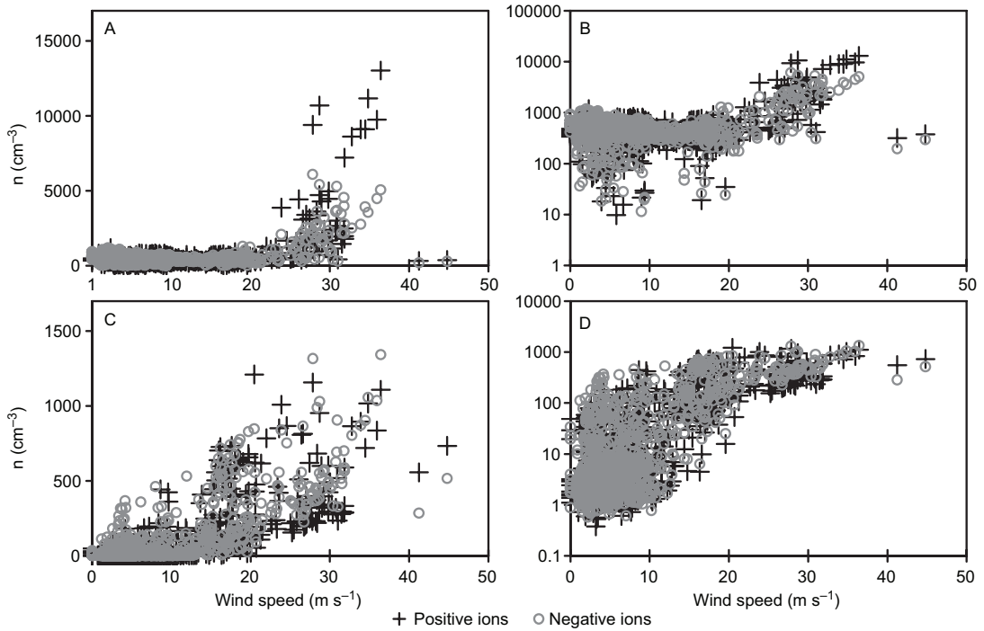
Fig. 5. Cluster (A and B) and intermediate ion (C and D) concentrations as a function of wind speed. Left: linear scale; right: logarithmic scale.
