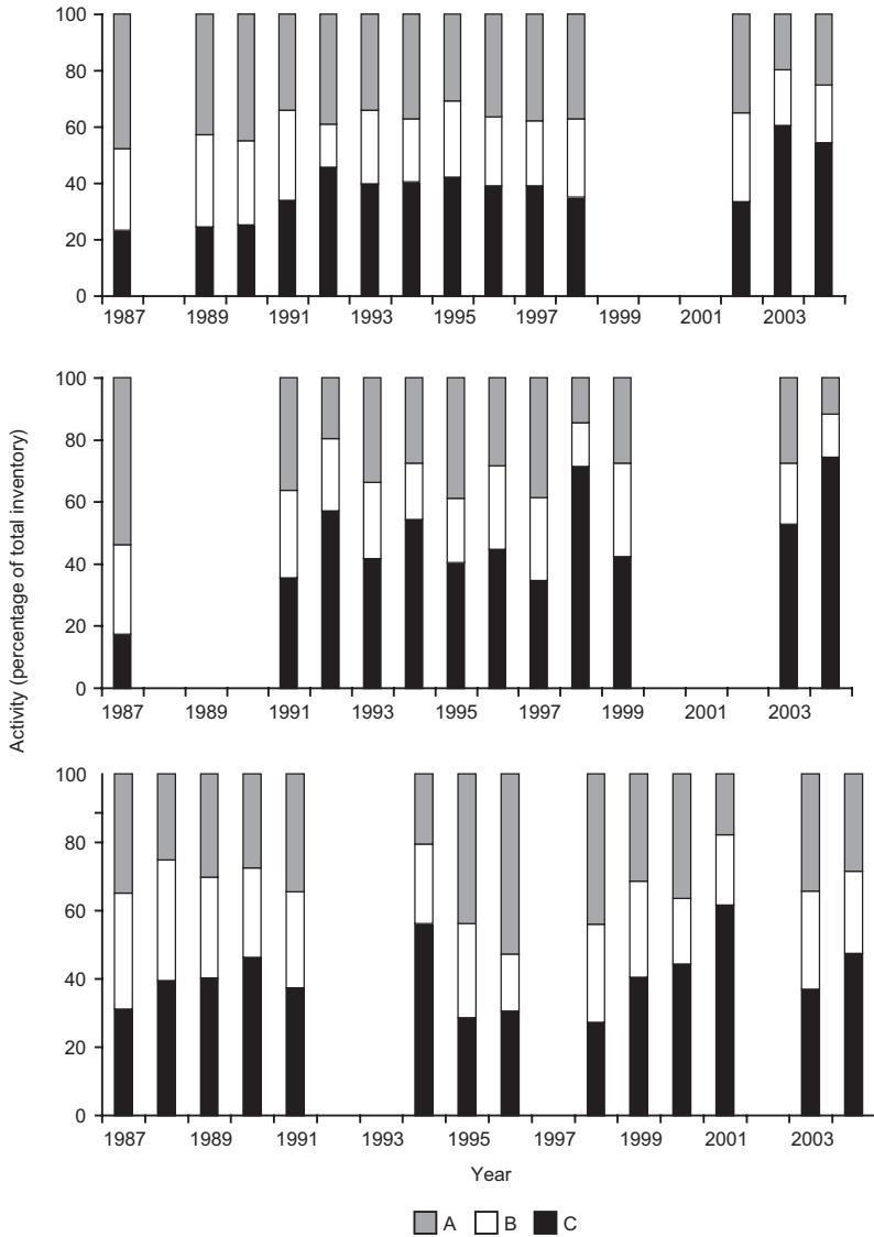
Fig. 5. Mean per cent of the total inventory of 137 Cs in different layers in lichen measured in Loviisa (top), Olkiluoto (middle) and Padasjoki (bottom).
