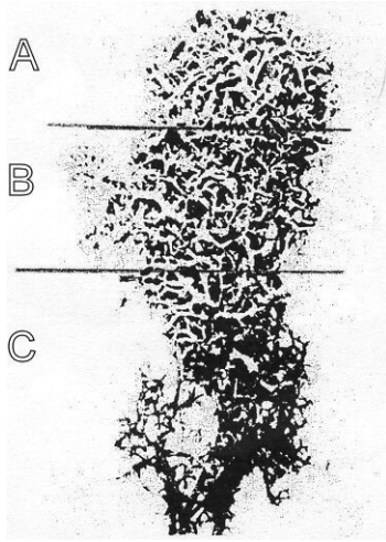
Fig. 1. Fractionation of lichen Cladonia stellaris .
