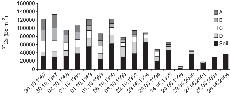
Fig. 4. Amounts of 137 Cs in different layers of lichen and soil beneath the lichen in Padasjoki. All parallel samples are presented separately.
