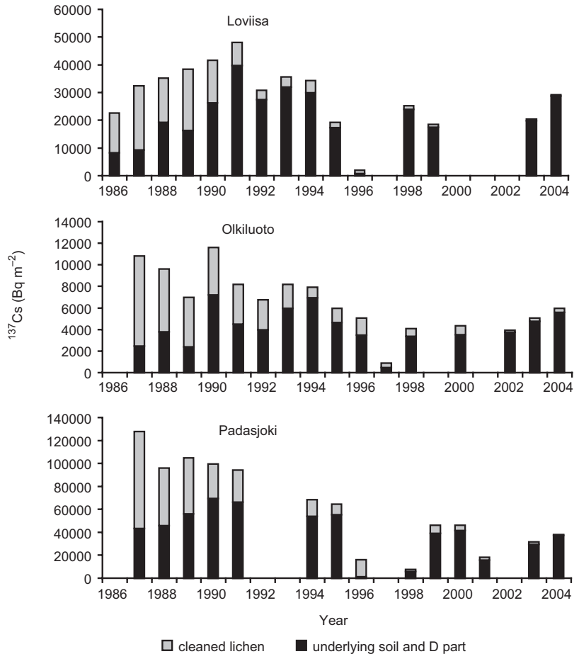
Fig. 3. Average amounts of ^{137}\text{Cs} (Bq m -2 ) in the total profile and cleaned lichen.
