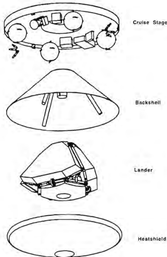
Fig. 1. Exploded view of Mars Pathfinder flight system, showing pack-pack-style cruise stage; backshell with three solid rockets, tetrahedron-shaped lander, and aeroshell.
