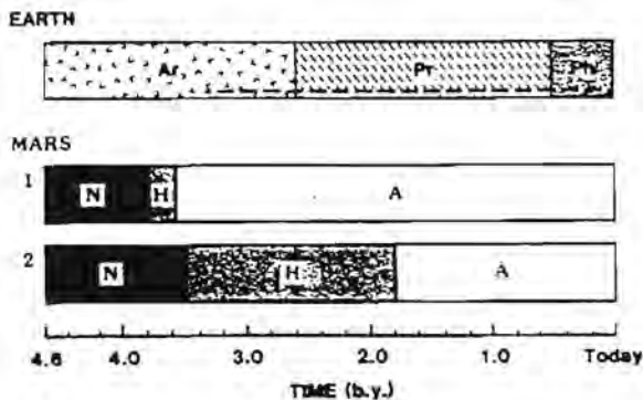
Fig. 1. Geologic time for the Earth can be broken into the Archean (Ar), Proterozoic (Pr), and Phanerozoic (Ph) periods. The dashed line represents the amount of time life is known to have existed on this planet. Geologic time for Mars is divided into the Noachian (N), Hesperian (H), and Amazonian (A) periods. The absolute ages are estimated from two different models of cratering rates. A sample of Hesperian material could determine whether model 1 [17] or model 2 [18] is correct. Because geologic evidence suggests that liquid water existed on the martian surface during both the Noachian and Hesperian, absolute ages based on model 2 imply that microbial life may have also evolved on Mars. (Reproduced from [19].)
