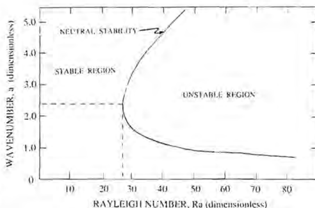
Fig. 2. Wavenumber vs. Rayleigh number. Critical Rayleigh number is 27.1 and critical wave number is 2.33. (After [6].)
