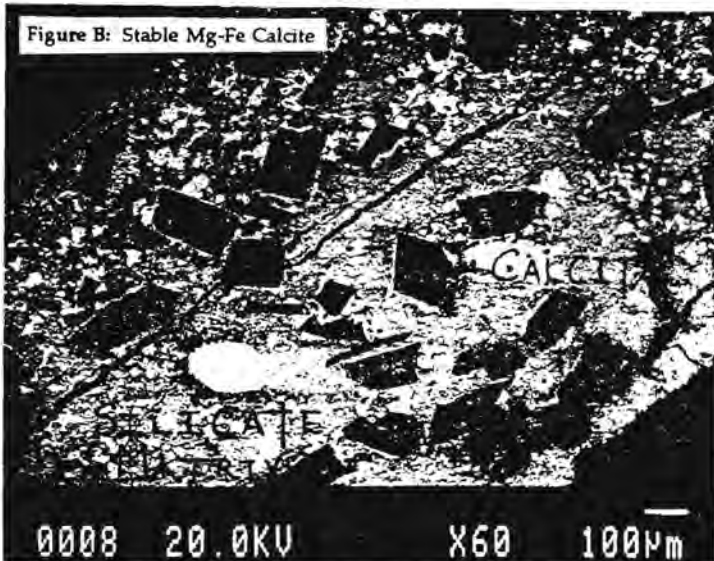
Figure B. Backscatter image of Mg-Fe calcite crystals within run product.
