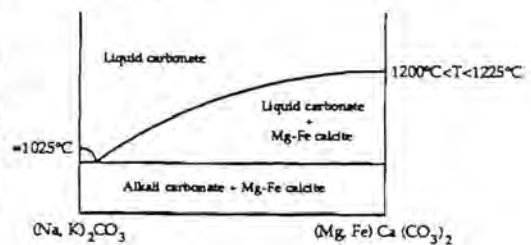
Figure D: Schematic projection of carbonate melting relations onto the alkali carbonate-Mg-Fe calcite join. Silicate relations not shown, but this diagram is for a phase assemblage which includes olivine, two pyroxenes and garnet.
