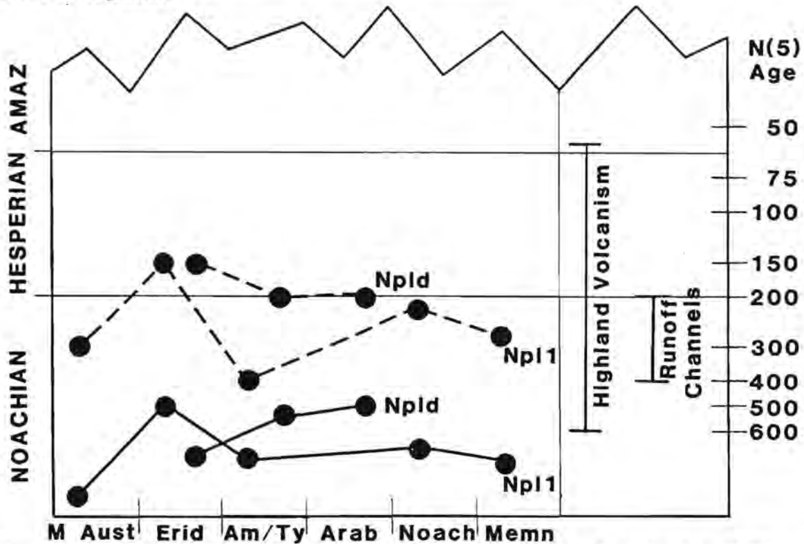
Figure 1. Timing of resurfacing in the areas mentioned in text. N(5) ages represent the number of craters >5-km-diameter per million square kilometers. Solid lines represent age of material based on all craters. Dashed lines represent termination of resurfacing event based on fresh, superposed craters.
