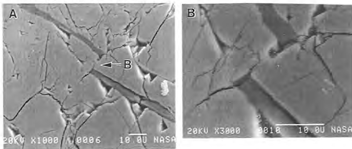
Figure 2. SEM photomicrographs (secondary-electron images) of a Nakhla rust vein broken by a partially healed fault in an olivine grain. Frame (B) is a detailed view of the area marked by an arrow in (A). Scale bars are in micrometers.
