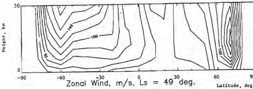
Figure 2b - Cross section of zonal wind (m/s) at 9 am local time for L_s = 49^\circ .
