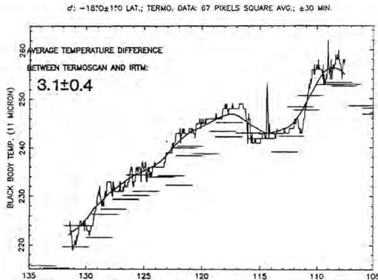
Figure 1: Comparison of Termoskan data with analogous IRTM data for a 2 degree wide strip of constant latitude centered on -18 degrees. The dark line represents a sliding boxcar average of Termoskan data which has been averaged to 2 x 2 degree squares. The lighter line is a 1 pixel IRTM strip for reference. The points represent IRTM data with the error bars representing the footprint of each IRTM data point. IRTM data is constrained to match the Termoskan data to within ±10 degrees of L_s and to within ±30 minutes of local time. After comparing each IRTM point with the averaged Termoskan point of the same longitude, the average temperature difference between Termoskan and IRTM is 3.1 \pm 0.4 K with the Termoskan temperatures being warmer. Local time of day in the data shown ranges from about 8.5 to 10.3.
