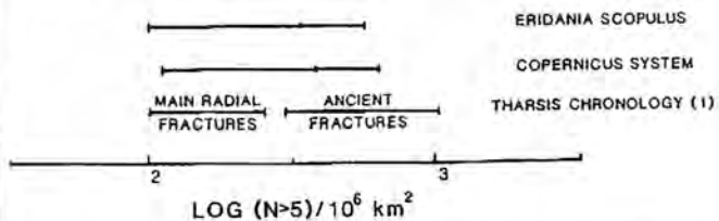
Figure 2. Crater ages derived from linear crater counts (6) for the scarp/ridge systems compared to the Tharsis tectonic history of Wise et al (1).
