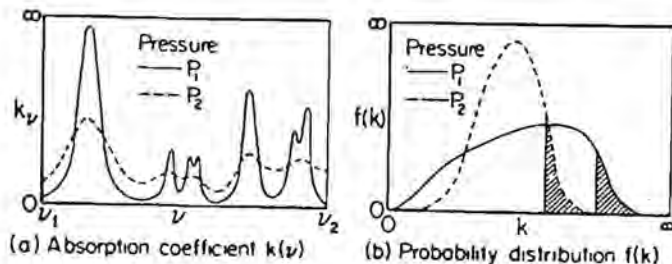
Figure 2. A schematic illustration portraying the essence of the exponential-sum approach. (a) shows a schematic of absorption line spectra at two different pressures. In (b) the two probability density functions f(k) associated with (a) are illustrated. The shaded area depicts the strongest absorption (i.e., largest k ) for the same spectral interval (i.e., f(k) for different pressures are correlated). Integration of f(k) over k replaces the integration of k_\nu over \nu (modified from [28], [29]).
