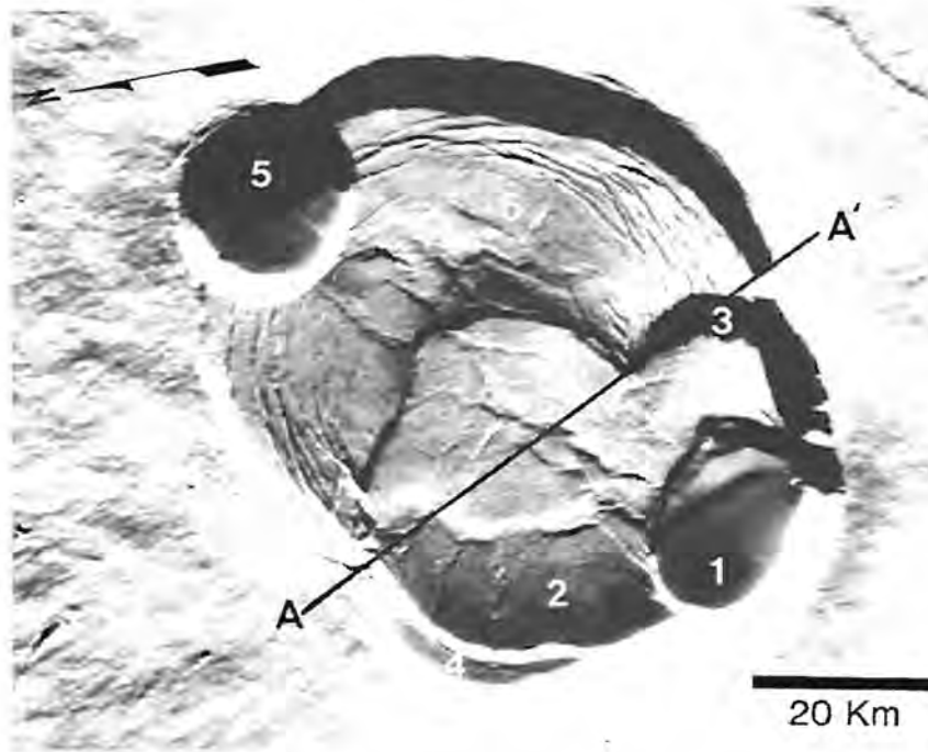
Fig. 1. Nested summit caldera of Olympus Mons.
