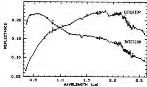
Figure 4. Reflectance spectra of interior and exterior surfaces of cordierite-biotite knotted schist sample SPLT001.
