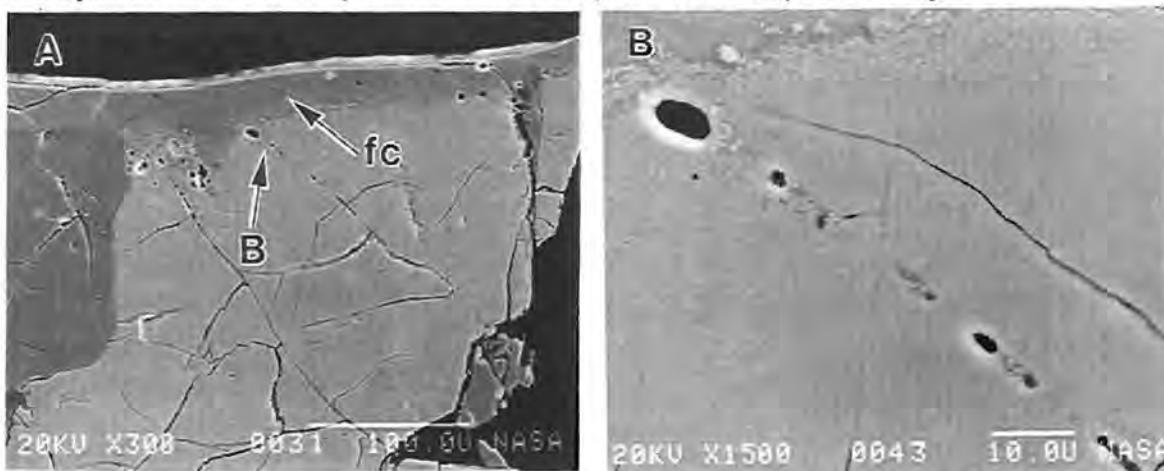
Figure 1. SEM photomicrographs (secondary-electron images) of a Nakhla rust vein truncated and partially decrepitated as it approaches fusion crust (fc). Scale bars are in micrometers.
