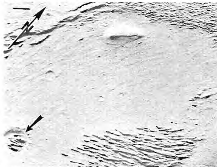
Figure 2. Erosional remnants of an older cover persist as yardangs in topographically-protected locations, here a crater undergoing erosional exhumation. Part of Viking orbiter frame 728A62, NGF rectilinear version. The scale bar is 1 km long.
