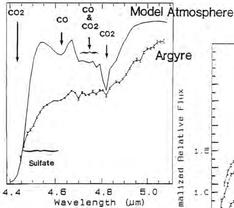
Figure 1. Representative spectra (Argyre region) and Mars model atmosphere of 7 mbar, 2 airmass, 240K, and CO / CO2 with atmospheric and surface absorptions labeled.
