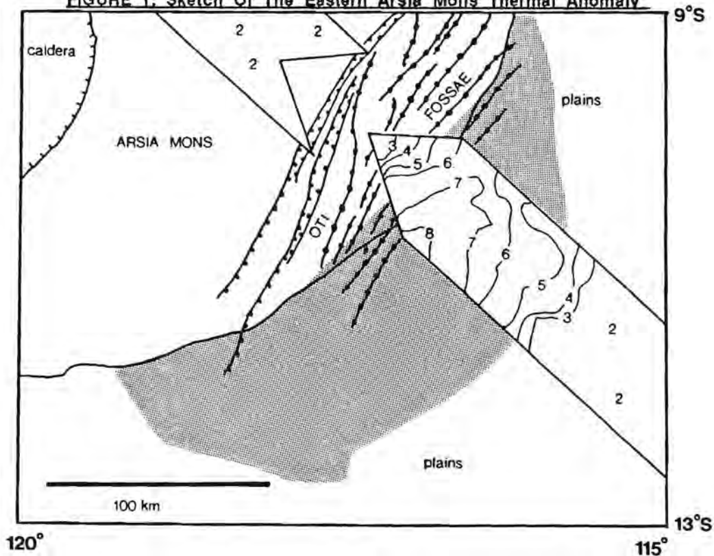
FIGURE 1: Sketch Of The Eastern Arsia Mons Thermal Anomaly.
