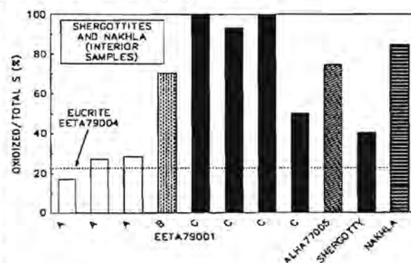
Figure 1. Relative abundances of sulfate in interior samples.
