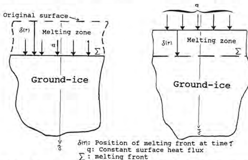
Fig. 2: Melting semi infinite solid with complete removal of melt from surface.
