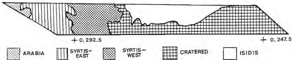
Figure 2. Schematic map for the above window of spectral units defined by (2) using the spectral characteristics of the first 51 channels of the ISM data.
