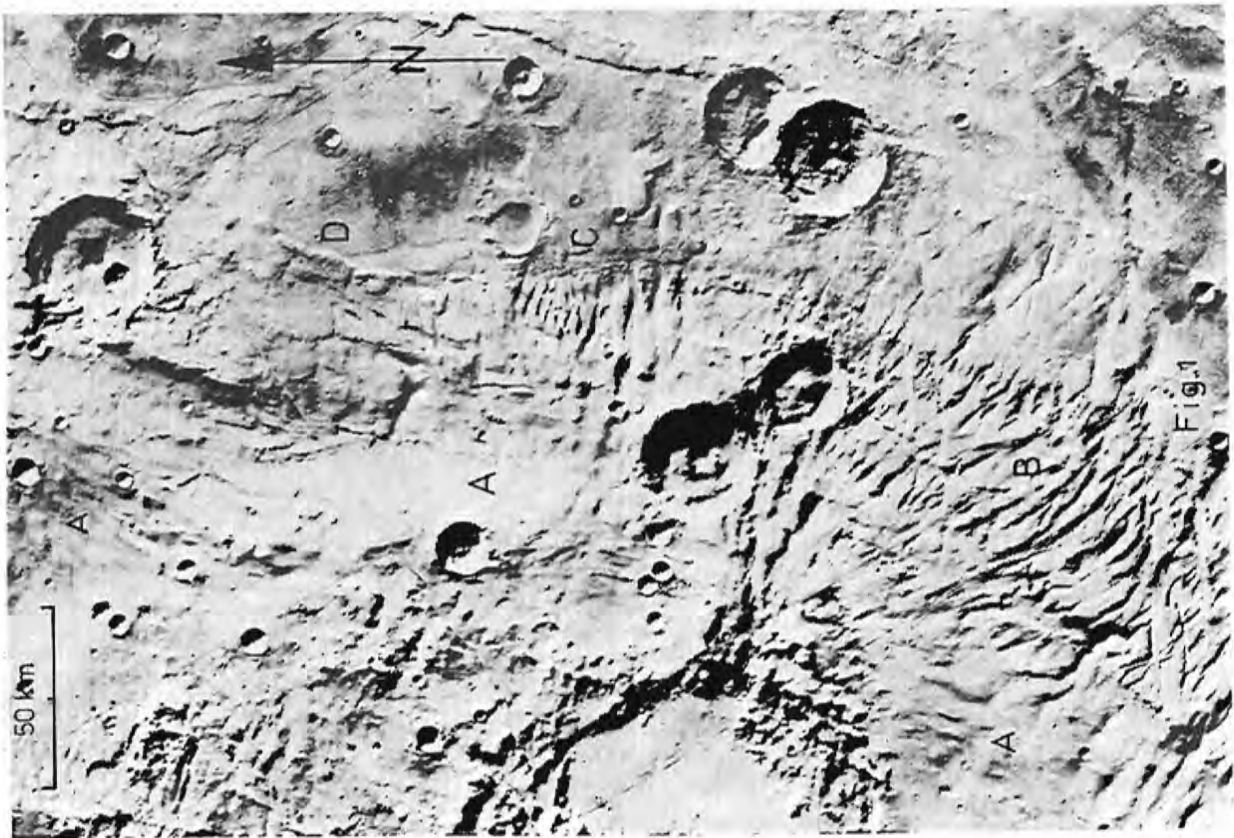
Fig. 1 Eastern margin of the TaNoVa - Updoming in sector A; Compressional ridges (A); rows of so called flat irons (B); cuesta landscape (C); and front of over-thrusted material (D).
