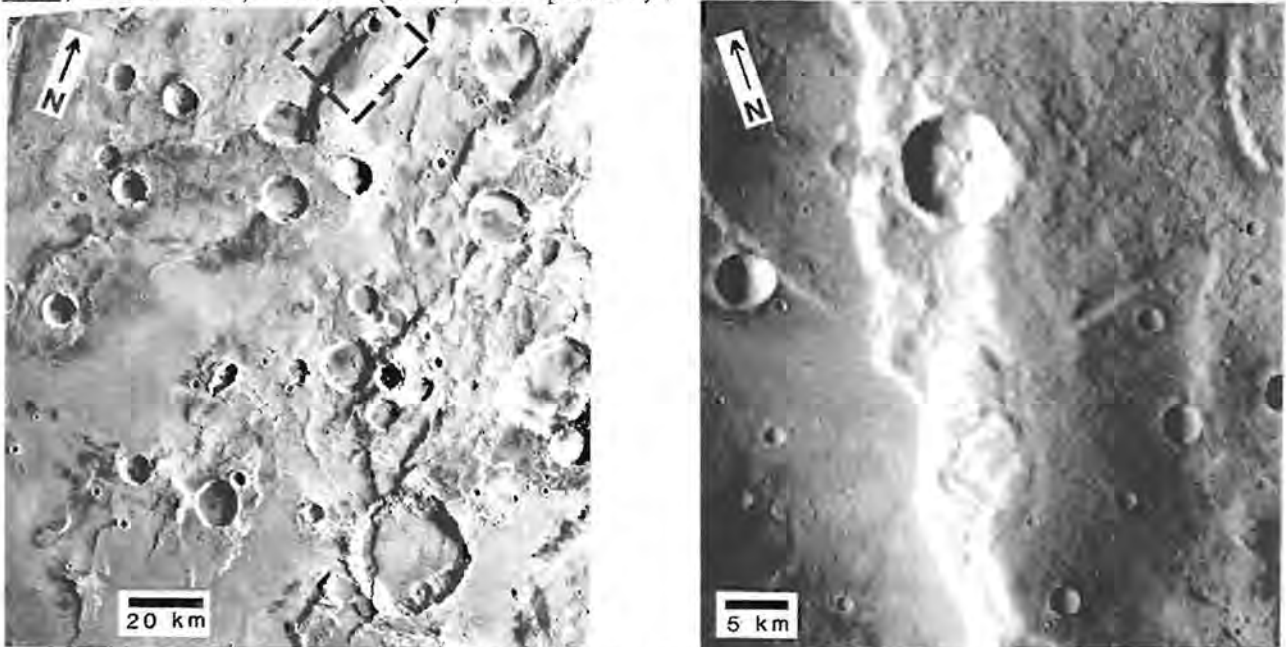
Fig. 1. Scarps in MTM -10147. a) Viking frame 639A10; box shows location of part b. b) Viking frame 454S01.
