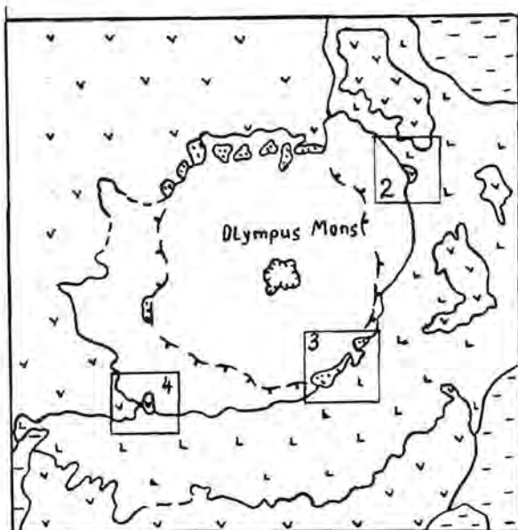
fig.1 Centr of the Olympus Mons. The places of fig.2,3,4.
