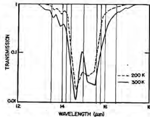
Figure 1. \text{CO}_2 15\ \mu\text{m} band transmission at 20 km altitude looking upward, at temperatures of 200K and 300K [25]. Also shown are the sub-intervals used for the 8 term and 16 term fits.
