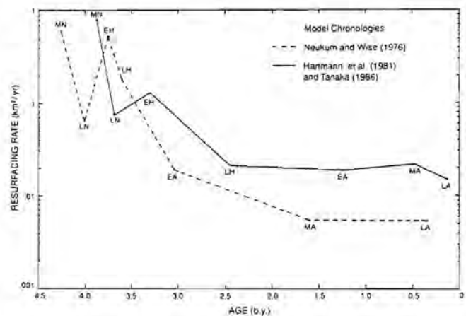
Fig. 2. Average resurfacing rates for volcanic plains corresponding to each martian epoch (modified from Tanaka et al. , 1988). Rates are based on the reconstructed areas of volcanic plains for two crater chronologies. Note the corrected resurfacing rates (reduced by a factor of 1000) from those of Tanaka et al. (1988). Martian epochs: MN, Middle Noachian; LN, Late Noachian; EH, Early Hesperian; LH, Late Hesperian; EA, Early Amazonian; MA, Middle Amazonian; LA, Late Amazonian.
