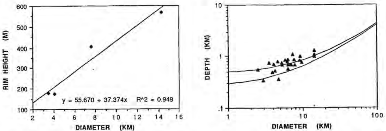
Fig. 2 (Left) Four of the studied craters possess measurable rim heights, permitting a linear least squares fit and, hence, the rim height to crater diameter relationship to be obtained. Fig. 3 (Right) Using the relationships between depth (Fig. 1) and rim height (Fig. 2) to crater diameter, the minimum depth of a crater that is required to penetrate the average thicknesses of the ridged plains materials can be inferred (2). Bottom curve - 200 m; top curve - 400 m plains thickness.
