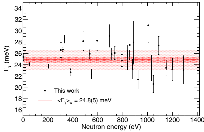
FIG. 12. Experimental values of \Gamma_\gamma for individual resonances are shown together with the average total radiative width. The narrow shadowed region indicates the uncertainty in \langle \Gamma_\gamma \rangle and the broader one shows the one standard deviation corridor around the obtained average.
