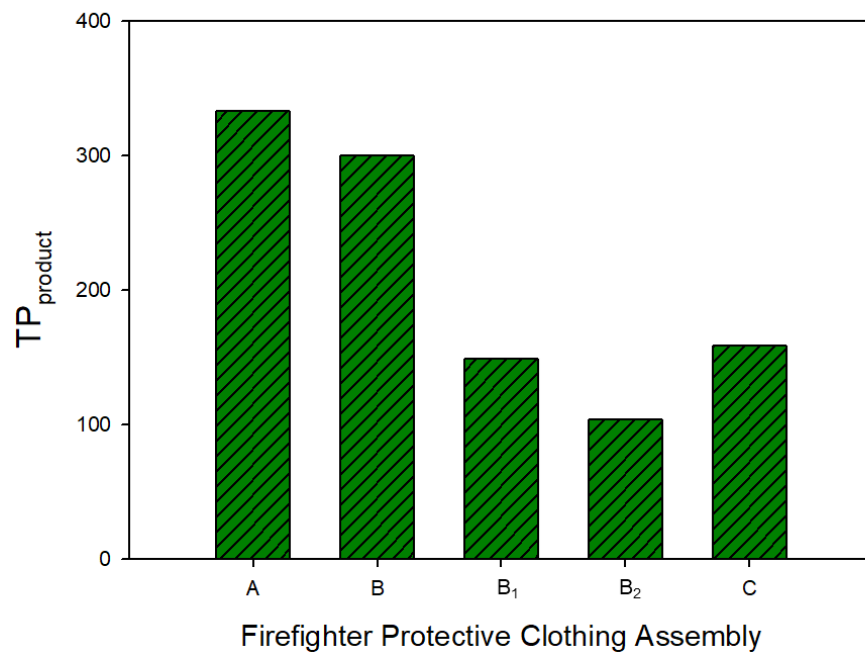
Figure 7. TP_{product} values (areas of rectangles in Figure 6) for the firefighter protective clothing assemblies.
