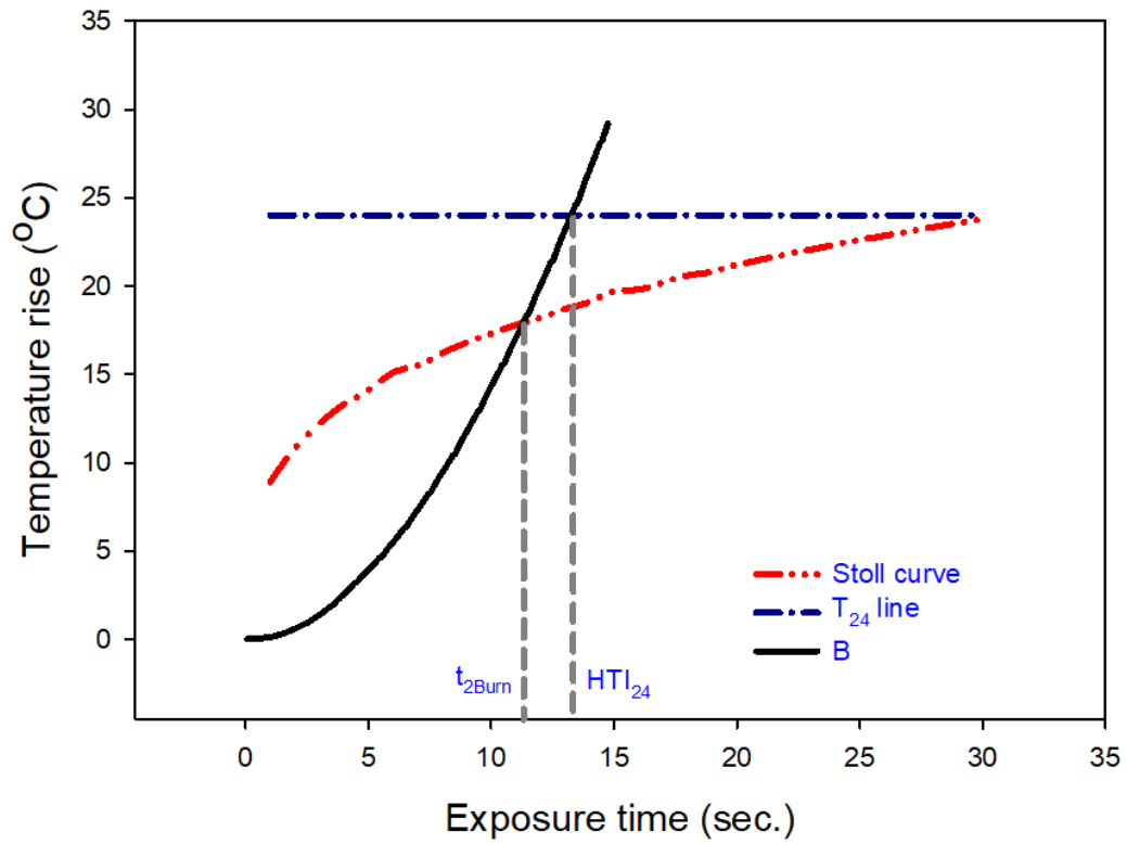
Figure 1. Determination of t_{2Burn} and HTI_{24} using B sample as an example in the FPP test. The point of intersection between the stoll curve and the B sample curve is t_{2Burn} . The point of intersection between T_{24} line and B curve is HTI_{24} .
