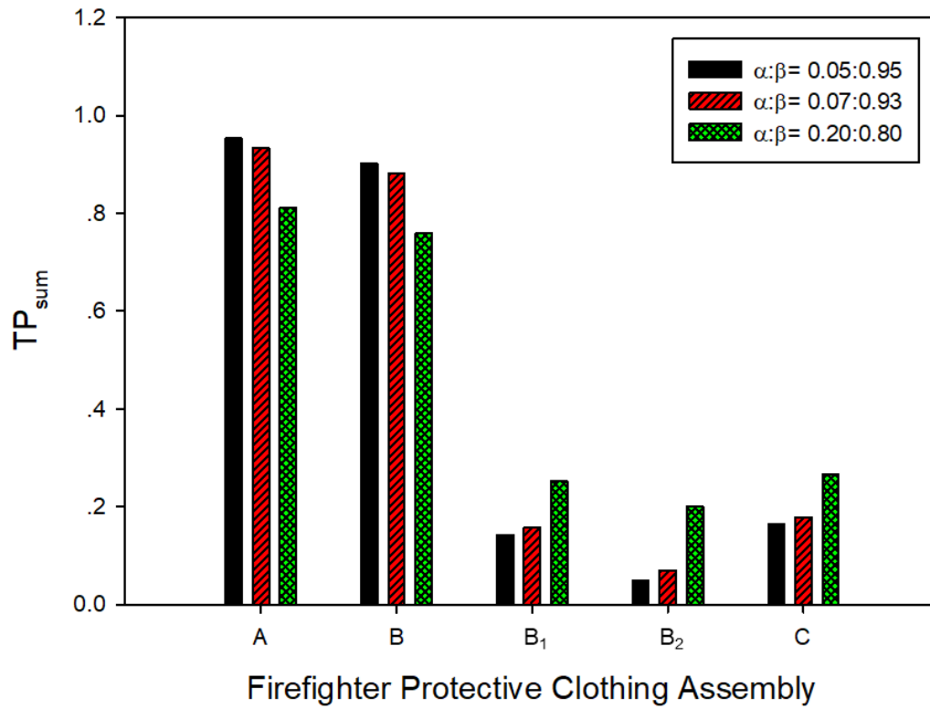
Figure 5. TP sum values for the firefighter protective clothing assemblies at various weighting values.
