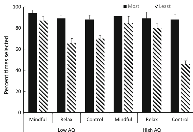
Fig. 2 Percentage times most and least-selected elements were chosen for each group at test
