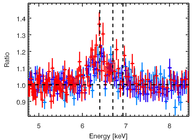
Figure 6. Suzaku -XIS [red] and NuSTAR FPMA [light blue] and FPMB [blue] ratio to a simple power law fitted to the 4.5-5.5 keV and 6.5-8.0 keV plotted in the rest frame of 3C 390.3. Also indicated by the three vertical lines are the rest frame positions of Fe K\alpha , Fe XXV and Fe XXVI. NuSTAR is binned to a signal-to-noise of 10 while Suzaku is binned to a signal-to-noise of 17 to agree better with the resolution of NuSTAR .
