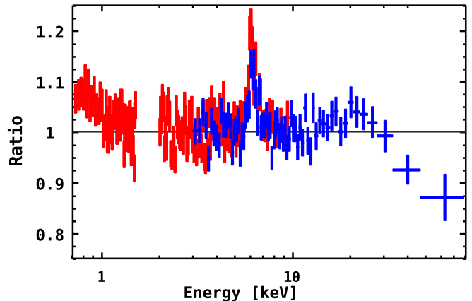
Figure 2. Residuals to a simple absorbed power law fitted to the 2-4 keV and 8-10 keV band for the front-illuminated Suzaku -XIS [red] and NuSTAR -FPMA [blue]. The data have been rebinned strongly for plotting.
