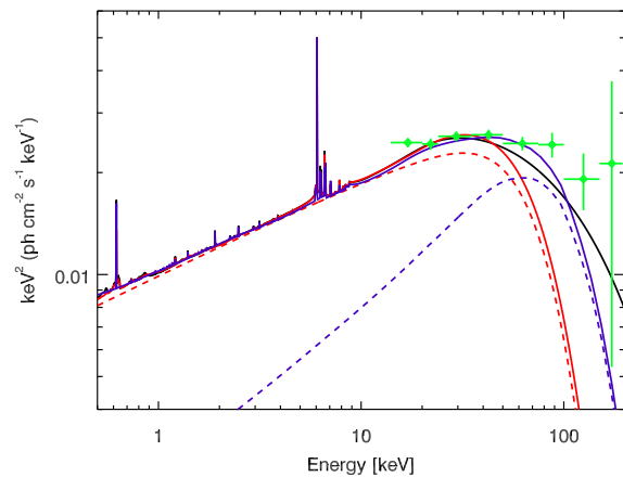
Figure 8. 70 month Swift -BAT spectrum with overlaid unabsorbed best fit models for the three different continua considered here: pexmon (black curve), compTT (red curve), eqpair (purple curve). The dashed curves show only the primary continuum for the two Comptonization fits.
