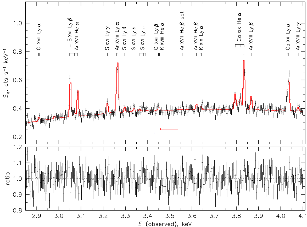
FIG. 1.— SXS spectrum from the whole field of view, combining 3 pointings. Energy is in the observer frame; bins are 4 eV for clarity (2 eV bins were used for fitting). Vertical error bars are 1\sigma Poisson uncertainties in each bin, horizontal error bars denote the bins. Red curve is a best-fit BAPEC model with kT = 3.5 keV, abundances of 0.54 solar (same for all elements), l.o.s. velocity dispersion of 180 km/s, and a power-law component as required by a fit in a broader band (see text). Prominent atomic lines seen in the model (identified using AtomDB) are marked, along with the interesting Ar xvii satellite line (B14) that’s too faint to be seen in the model. Brackets show 90% confidence intervals on the unidentified 3.5 keV line energy for the most-restrictive XMM MOS stacked-clusters sample in B14 (red) and for the XMM MOS Perseus spectrum from the region covered by the SXS (blue).
