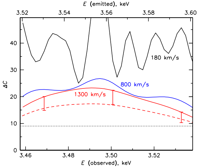
FIG. 2.— Difference of C statistic between a model with the best-fit XMM MOS flux ( 9 \times 10^{-6} phot s^{-1} cm^{-2} ) and the best-fit SXS flux (shown in Fig. 3; flux is allowed to take negative values) as a function of line energy within the B14 most restrictive confidence interval for the line. Curves for different line widths are shown (black: 180 km\ s^{-1} , blue: 800 km\ s^{-1} , red: 1300 km\ s^{-1} ). For the 1300 km\ s^{-1} case, we also show \Delta C between models with the XMM MOS line flux and zero line flux (red dashed line). Error bars illustrate a systematic uncertainty of the SXT effective area described in §3.1; its effect is most significant for the broad line and we do not show other cases for clarity. Dotted line is at \Delta C = 9 , which corresponds to 3\sigma exclusion for Gaussian errors.
