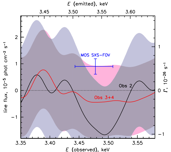
FIG. 5.— The best-fit flux (curves) and \pm 3\sigma limits (shaded bands) for a 1300 km s -1 broadened line (similar to the red line and pink band in Fig. 3), derived separately for the early subset (“Obs 2”, black and gray) and later subset (“Obs 3+4”, red and pink). The axes and the blue cross are the same as in Fig. 3. The “dip” around 3.5 keV is present in the early subset and not in the late one, but the results are statistically consistent.
