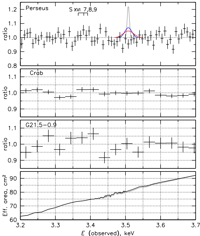
FIG. 4.— Ratios of data to best-fit models in the interesting energy range. Upper panel shows ratio of the same Perseus spectrum and model as in Fig. 1, but binned by 8 eV. A line at 3.57 keV (rest-frame) with a flux derived by XMM in the SXS FOV (§4.2) is shown with curves of different colors, which denote different l.o.s. velocity dispersions (gray: 180 km s -1 , blue: 800 km s -1 , red: 1300 km s -1 , see §4.2). Position of the potentially interesting S xvi feature (§4.3.1) is marked. Two middle panels show the residuals for power-law sources Crab and G21.5–0.9. The area modification (§3.1) is not included. The Crab spectrum has sufficient statistics to exclude a significant effective area artifact around 3.5 keV. Lower panel shows the effective area curve (gray line shows the modification from §3.1), including the fine structure above the Au M1 edge measured during ground calibration.
