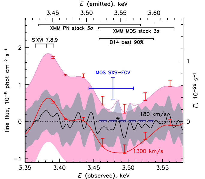
Fig. 3.— The best-fit line flux (solid curves) and the flux limits for C_{\min} + 9 ( \pm 3\sigma ; shaded bands) for an additional emission line as a function of energy. We show an interesting broad band encompassing XMM MOS and pn 3\sigma intervals for stacked-cluster samples from B14 (brackets at top). Black line with gray band (labeled 180 \text{ km s}^{-1} ) corresponds to a turbulent-broadened line, red line with pink band ( 1300 \text{ km s}^{-1} ) corresponds to a DM line. A magenta outline shows the highest flux limit from those for different widths in the 180\text{--}1300 \text{ km s}^{-1} interval. Red and black error bars illustrate the systematic uncertainty of the effective area (§3.1), shown for the best-fit curve and the upper limit for the broad line. This effect is negligible for the narrow line, so only one location is shown. A line flux of 5 \times 10^{-6} \text{ phot cm}^{-2} \text{ s}^{-1} corresponds to \text{EW} \approx 1 \text{ eV} . Blue cross shows the MOS detection for the SXS FOV with 1\sigma one-parameter uncertainties. Blue dashed line shows the expected flux based on the stacked-cluster signal (§5). Also shown for reference is the “B14 best” interval covered by Fig. 2. The only interesting unmodeled positive deviation — though a low-significance one — is near the energies of the high- n transitions of S XVI, marked at top. The right vertical axis shows the approximate corresponding sterile neutrino decay rate \Gamma .
