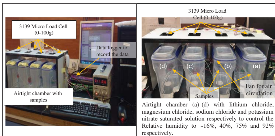
Figure 7. A custom built successive desiccator chamber system.
