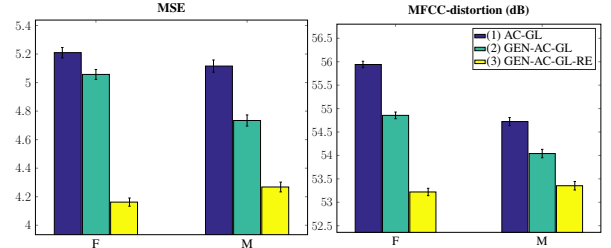
Figure 4: Average test set MSE and MFCC distortion with 95% confidence intervals for the male (M) and the female (F) voice. The baseline training scheme (1) consistently gives higher errors than the ones (2–3) trained with generated acoustic features. Using re-estimated excitation waveforms in training (3) further reduces the errors.
