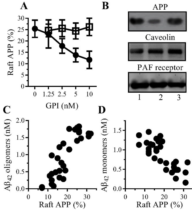
Figure 10 - GPIs reduced APP within lipid rafts – (A) The amounts of APP in DRMs (Rafts) in 7PA2 cells treated with GPIs (●) or desialylated GPIs (□) as shown. Values are means \pm SD from triplicate experiments performed 3 times, n=9. (B) Immunoblots showing the amounts of APP, caveolin and PAF receptors in DRMs (rafts) from 7PA2 cells treated with control medium (1), 10 nM GPIs (2) or 10 nM desialylated GPIs (3). (C) There was a significant correlation between the amounts of APP in lipid rafts (DRMs) and the concentrations of A \beta 42 oligomers found in CM from 7PA2 cells treated with GPIs (1.25 to 10 nM), Pearson’s coefficient =0.84, P<0.01. (D). There was a significant inverse correlation between the amounts of APP in lipid rafts (DRMs) and the concentrations of A \beta 42 monomers found in CM from 7PA2 cells treated with GPIs (1.25 to 10 nM), Pearson’s coefficient= -0.79, P<0.01.
