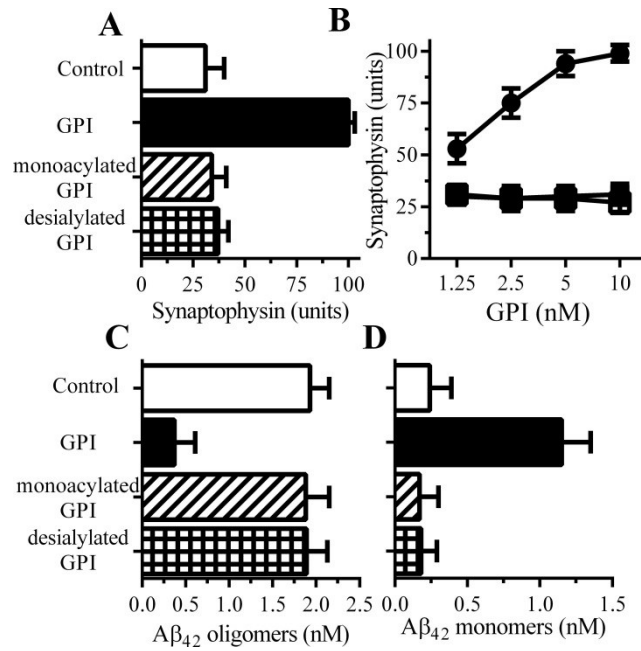
Figure 8. GPI-mediated suppression of toxic A \beta release is dependent upon sialic acid - (A) The amounts of synaptophysin in neurons incubated with CM from 7PA2 cells treated with control medium ( \square ), 10 nM GPIs ( \blacksquare ), 10 nM monoacylated GPIs (striped bars) or 10 nM desialylated GPIs (hatched bars). Values are means \pm SD from triplicate experiments performed 3 times, n=9 . (B) The amounts of synaptophysin in neurons incubated with CM from 7PA2 cells treated with GPIs ( \bullet ), monoacylated GPIs ( \square ) or desialylated GPIs ( \blacksquare ) as shown. Values are means \pm SD from triplicate experiments performed 3 times n=9 . The concentrations of A \beta_{42} oligomers (C) and A \beta_{42} monomers (D) in CM from 7PA2 cells treated with control medium ( \square ), 10 nM GPIs ( \blacksquare ) 10 nM monoacylated GPIs (striped bars) or 10 nM desialylated GPIs (hatched bars). Values are means \pm SD from triplicate experiments performed 3 times, n=9 .
