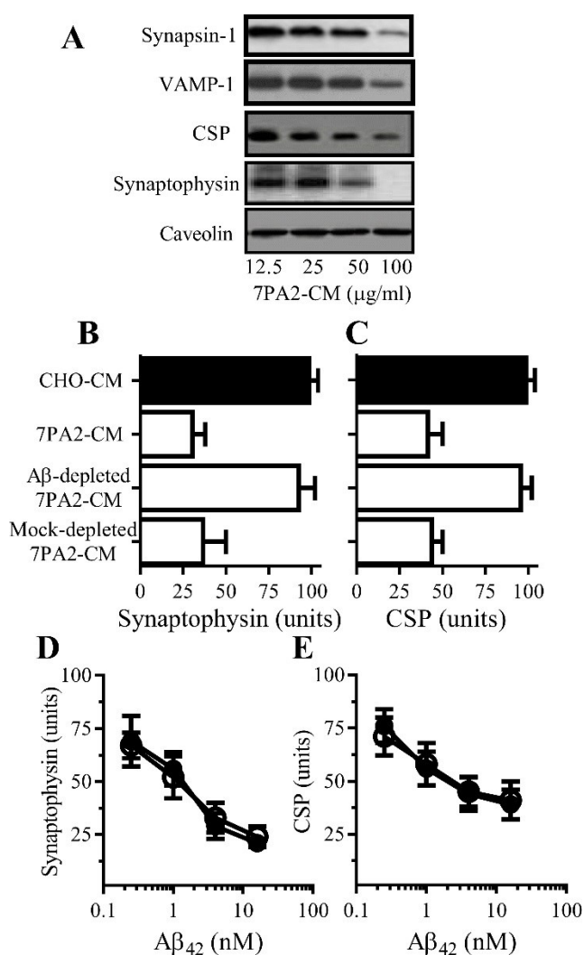
Figure 1. Soluble Aβ caused synapse damage in neurons - (A) Immunoblots showing the amounts of synapsin-1, VAMP-1, CSP, synaptophysin and caveolin in neurons incubated with 7PA2-CM as shown. The amounts of synaptophysin (B) and CSP (C) in neurons incubated with CHO-CM (■) or 7PA2-CM, Aβ-depleted 7PA2-CM or mock-depleted 7PA2-CM (□). Values are means ± SD from triplicate experiments performed 3 times, n=9 . The amounts of synaptophysin (D) and CSP (E) in neurons incubated with 7PA2-CM (○) or soluble brain extract (●) containing Aβ 42 as shown. Values are means ± SD from triplicate experiments performed 3 times, n=9 .
