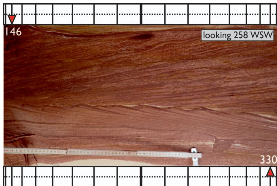
FIG. 4.—Example of presentation technique applied to an individual bed. Bidirectional dip of superimposed foresets within tidal herringbone cross-stratification. Dip direction of upper set shown at top of image and dip direction of lower set at bottom of image. Silurian Tumblogooda Sandstone, Kalbarri National Park, Western Australia.
