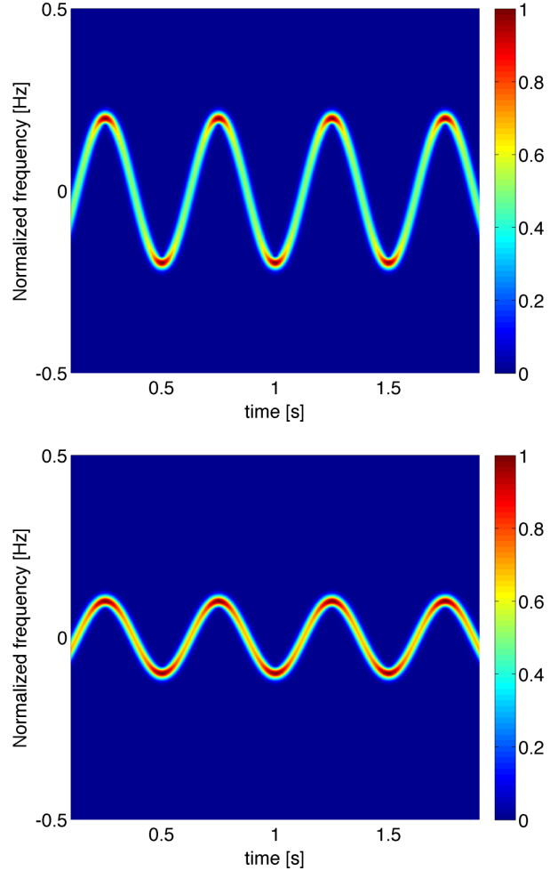
Fig. 2. Micro-Doppler of an oscillating target from 2 different aspect angles.
