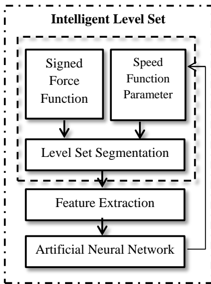
Fig. 4 The intelligent level set.
