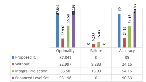
Fig. 18 Comparison of segmentation performance accuracy in each method.
