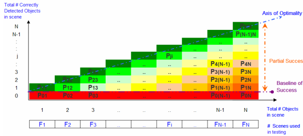
Fig. 12 Tabular presentation form by using metric-based empirical estimation object counting technique.
