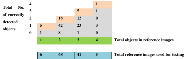
Fig. 14 Segmentation results using predefined IC selection.
