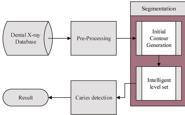
Fig. 1 General framework.
