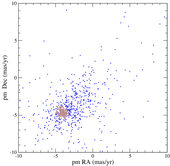
Figure 6. Gaia DR2 proper motions for targets within 3.5 arcsec of the centre of Be 55, showing concentration of selected candidate members in grey. This field has a much lower stellar density than that of Be 51, but the cluster members are about two magnitudes brighter, resulting in smaller uncertainties.
