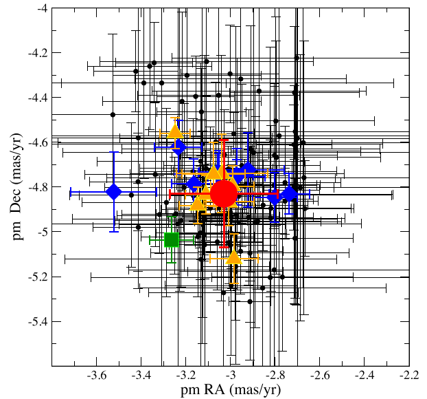
Figure 7. Gaia DR2 proper motions, with uncertainties, for cleaned sample of 117 stars identified as probable members of Be 51. The Cepheid #162 is shown with a green square; the eight other cool supergiants (listed in the top panel of N18 table 3) are shown with yellow triangles; B-type stars observed spectroscopically are shown with blue diamonds. One B-type star, #143, is not included here or in Fig. 9 because its astrometric solution in DR2 appears faulty (it has a negative parallax with very large associated uncertainty: -0.36 \pm 0.21 ). The large red circle indicates the weighted average for the cleaned sample, with error bars corresponding to the median uncertainty for single stars: pmRA = -3.03 \pm 0.20 mas yr ^{-1} , pmDec = -4.83 \pm 0.24 mas yr ^{-1} .
