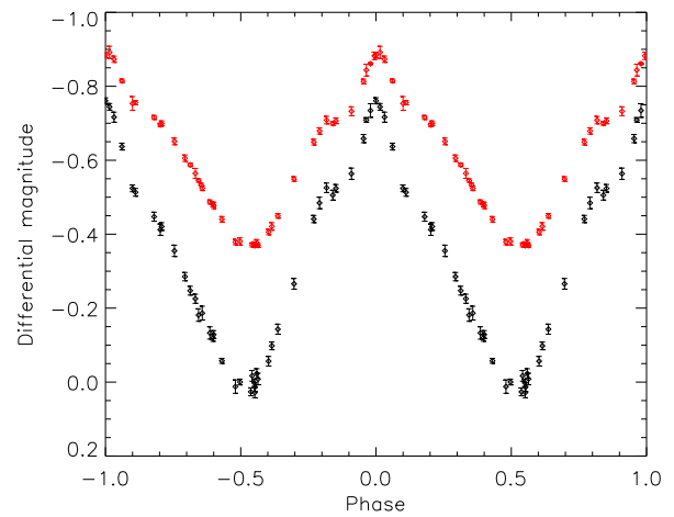
Figure 2. Differential light curves for #162 in V (black, lower curve) and i' (red, upper curve), folded on P = 9.83 d, with phase zero set from the V -band maximum. An artificial offset of 0.2 mag between the two curves has been inserted for clarity.
