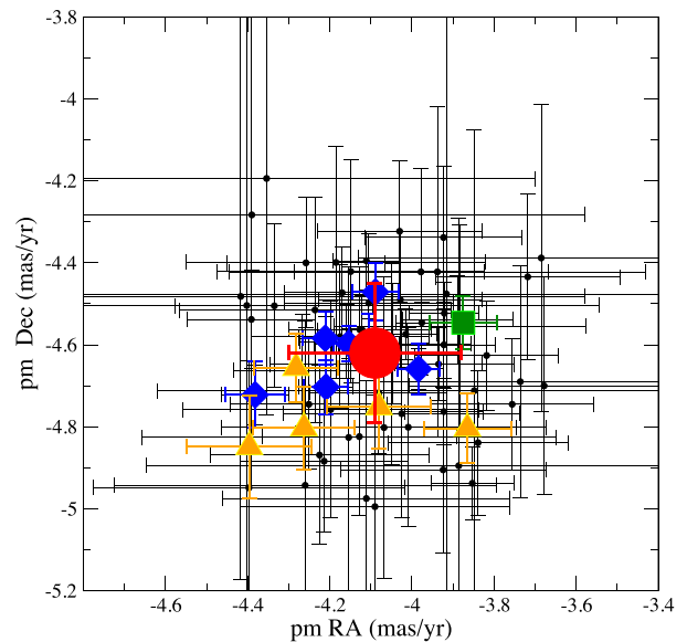
Figure 8. Gaia DR2 proper motions, with uncertainties, for cleaned sample of 44 stars identified as probable members of Be 55. The Cepheid #107 is shown with a green square; the five other cool supergiants (listed in N12 table 7, excluding possible foreground interloper S61) are shown with yellow triangles; B-type stars observed spectroscopically are shown with blue diamonds. One B-type star, #129, is not found in DR2. The large red circle indicates the weighted average for the cleaned sample, with error bars corresponding to the median uncertainty for single stars: pmRA = -4.09 \pm 0.19 mas yr ^{-1} , pmDec = -4.62 \pm 0.18 mas yr ^{-1} .
