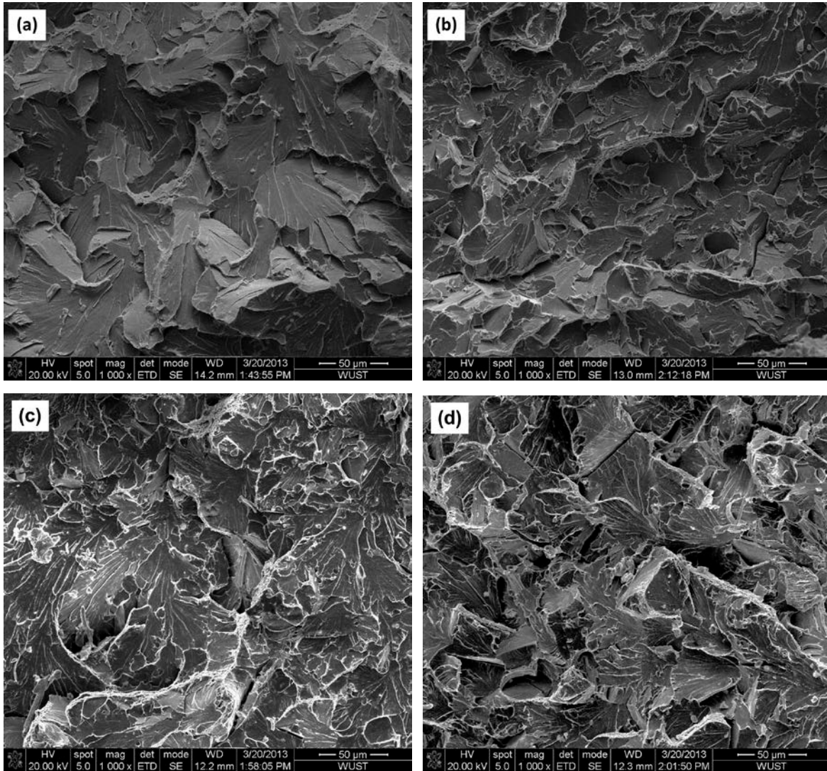
Fig. 7. Fracture surfaces (-30 °C) of normalized-tempered Cr-Mo alloyed steels (a) 0.54 %
