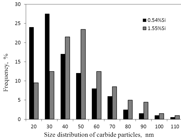
Fig. 5. Size distribution of alloy carbide particles: comparison between the high silicon and low silicon steels grades.
