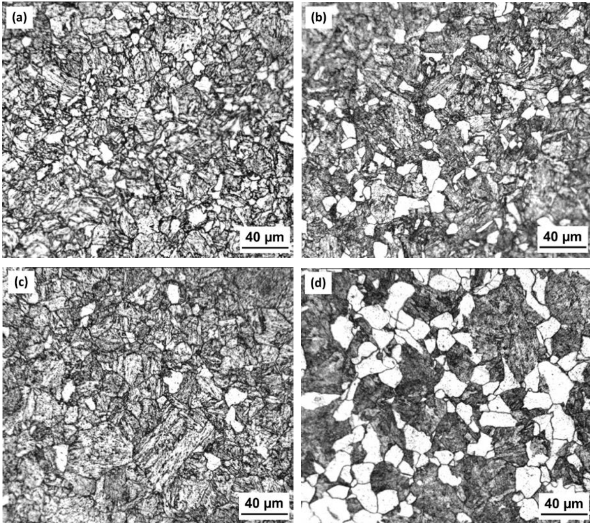
Fig. 1. Optical micrographs of tempered Cr-Mo alloyed steels (a) 0.54 % Si, 650 °C, (b) 1.55 % Si, 650 °C, (c) 0.54 % Si, 700 °C, (d) 1.55% Si, 700 °C.
