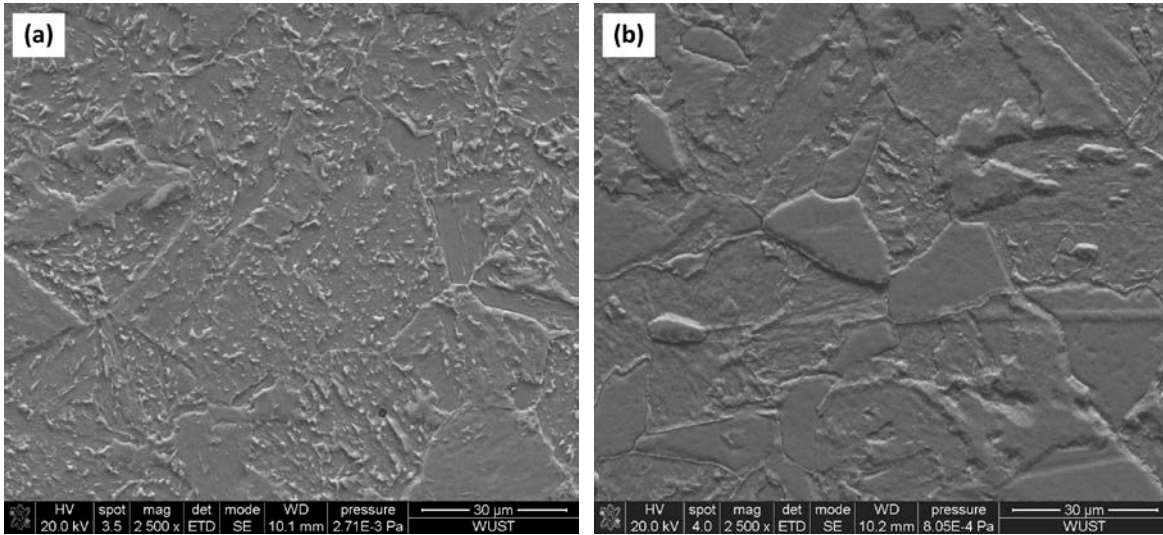
Fig. 2. SEM micrographs of steel samples tempered at 650 °C (a) 0.54 % Si, (b) 1.55 % Si.
