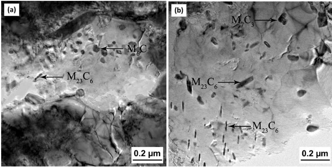
Fig. 4. TEM micrographs of precipitates in (a) 0.54 % Si and (b) 1.55 % Si steels
