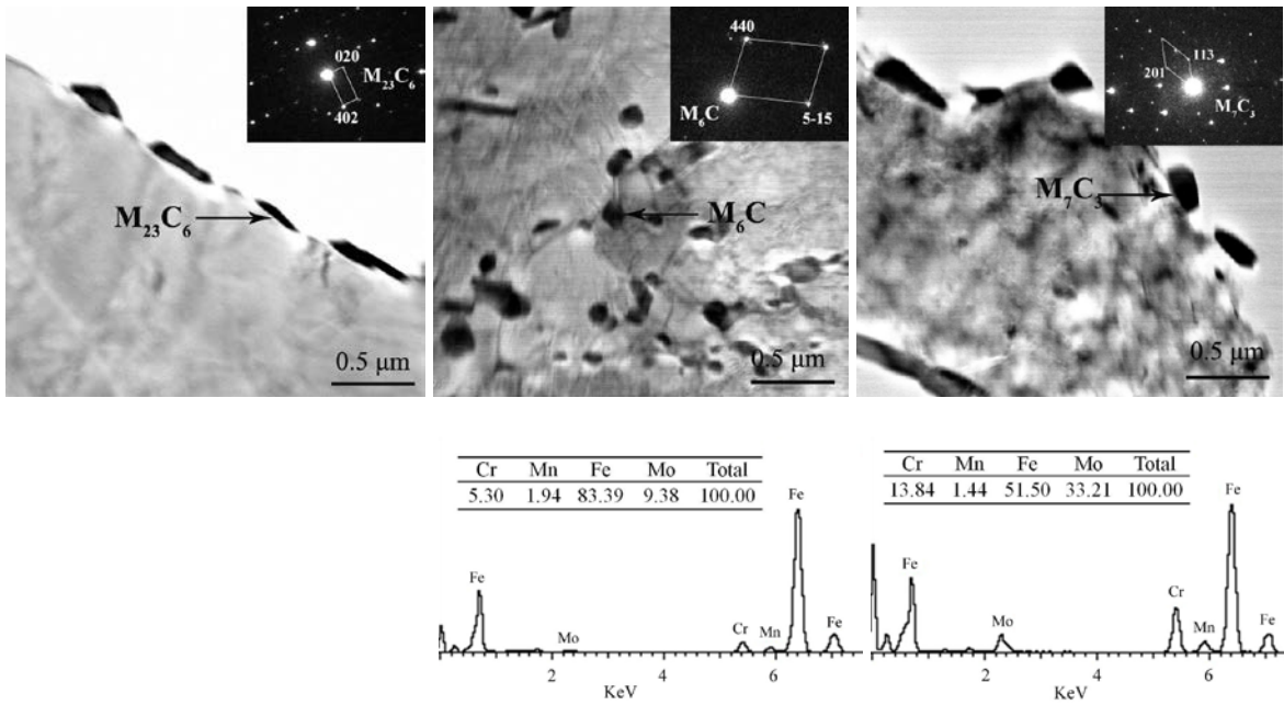
Fig. 3. TEM micrographs of various carbides and corresponding EDS results
