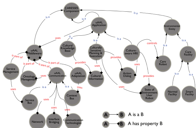
Fig. 10. Overview of Ontology
