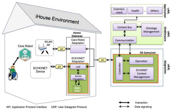
Fig. 7. System Architecture
