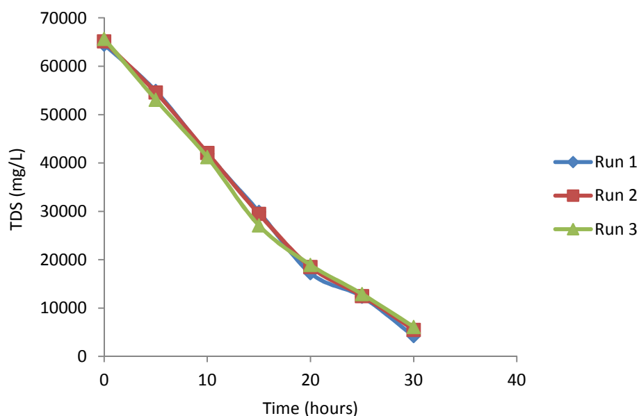
Figure 6: Effect of vermifiltration on distillery effluent TDS
