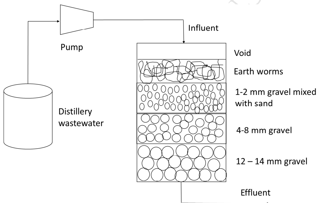
Figure 2: Vermifiltration technology working principle
