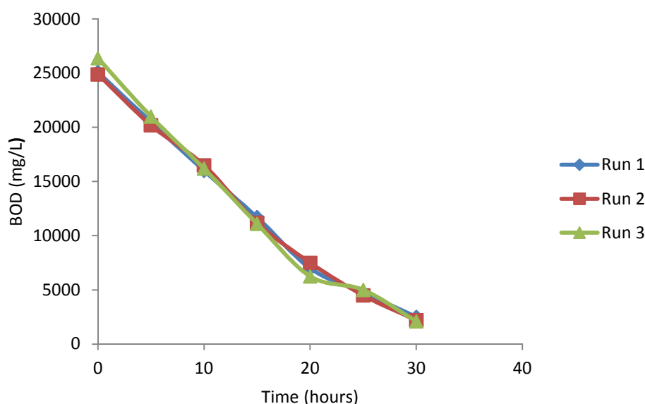
Figure 5: Effect of vermifiltration on distillery effluent BOD
