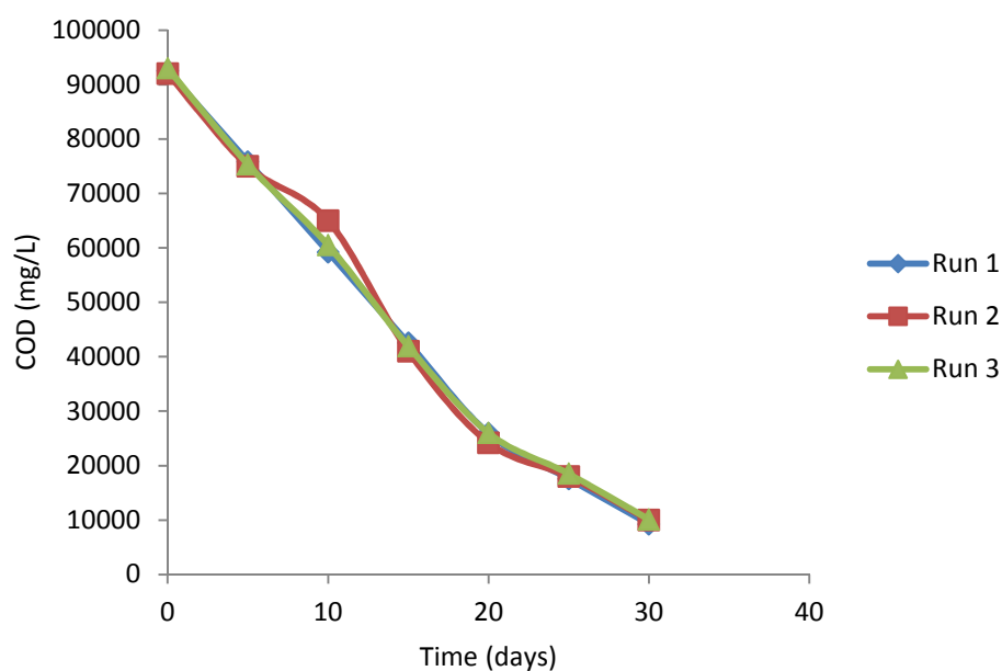
Figure 8: Effect of vermifiltration on distillery effluent COD
