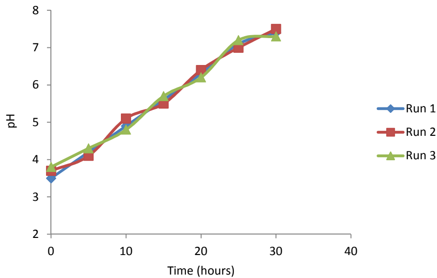
Figure 3: Effect of vermifiltration on distillery effluent pH
